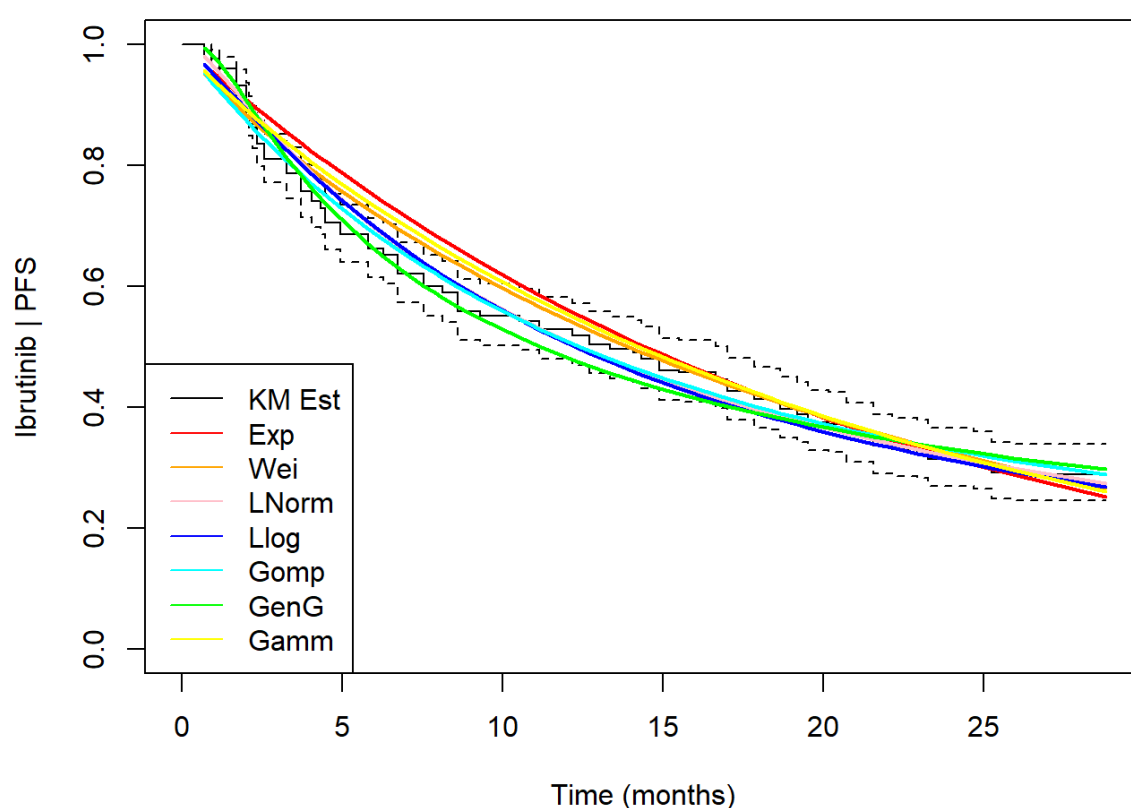
Figure 36: Parametric model fit over trial length (ibrutinib PFS)
