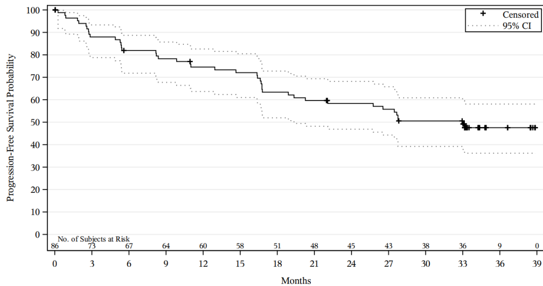
Figure 11: Kaplan-Meier plot of PFS by INV in BGB-3111-206 (full trial population)
