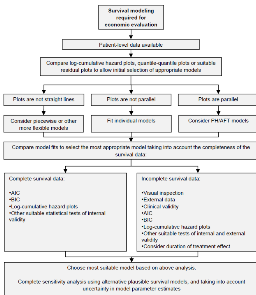
Figure 23: Survival Model Selection Process Algorithm Presented by NICE DSU TSD-14, and Referenced by Other HTA Agencies
