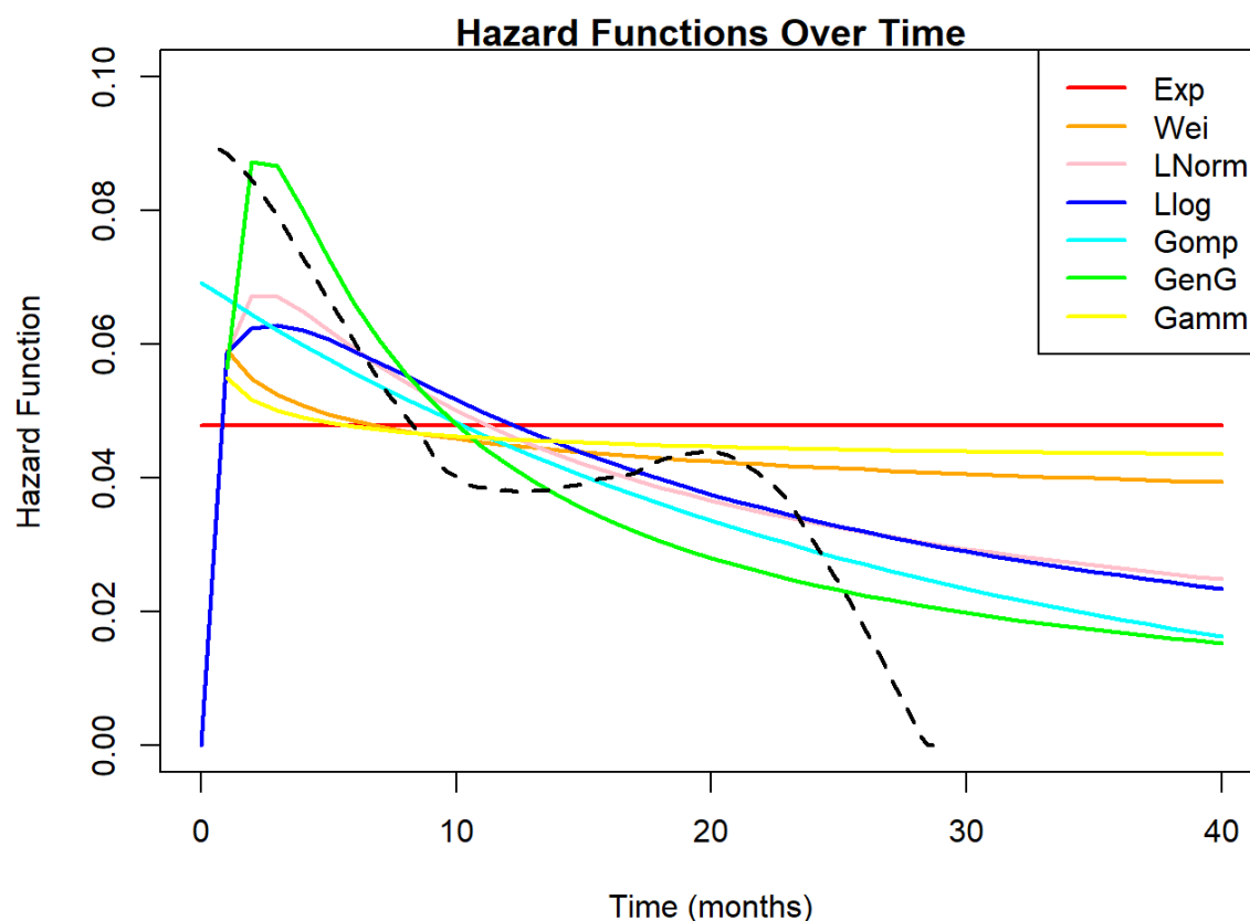
Figure 38: Parametric model hazard functions with observed hazards overlaid in black (ibrutinib PFS)
