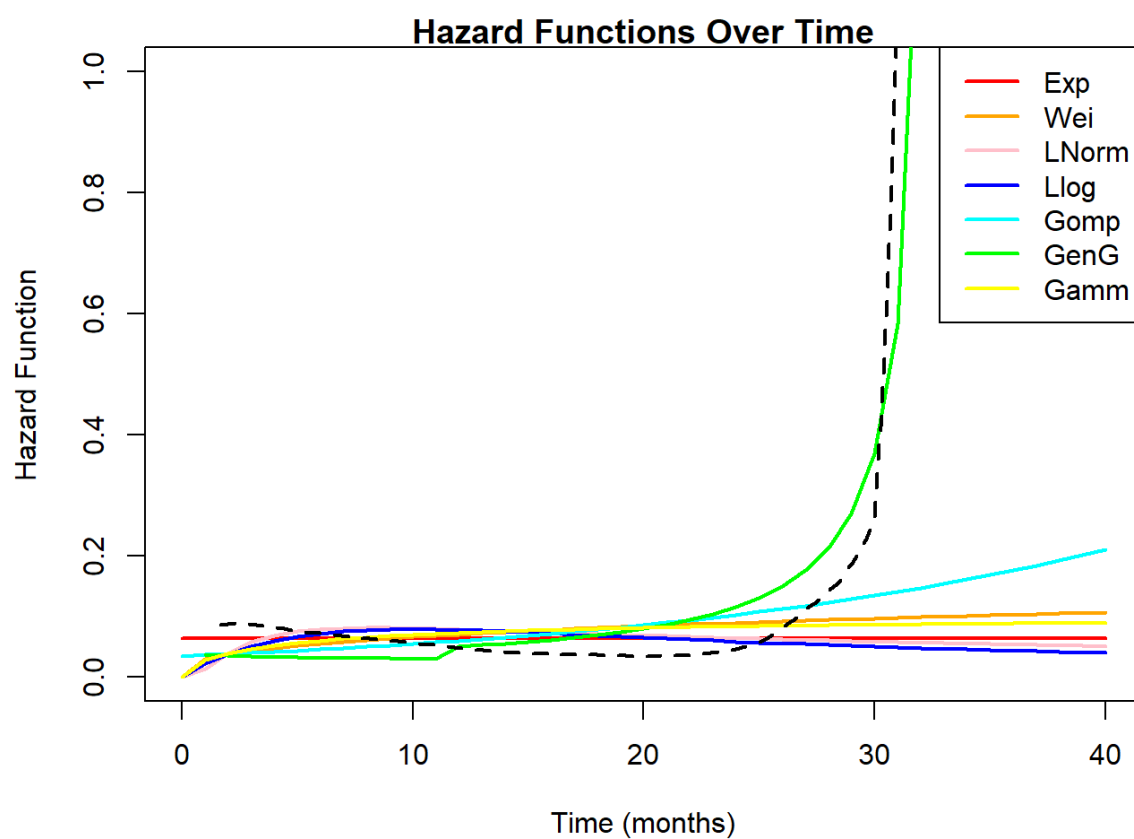
Figure 47: Parametric model hazard functions with observed hazards overlaid in black (ibrutinib TTD)
