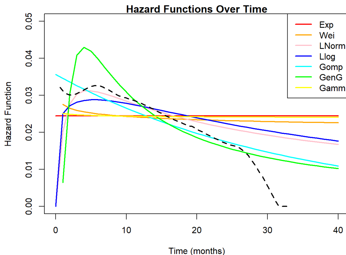
Figure 43: Parametric model hazard functions with observed hazards overlaid in black (ibrutinib OS)
