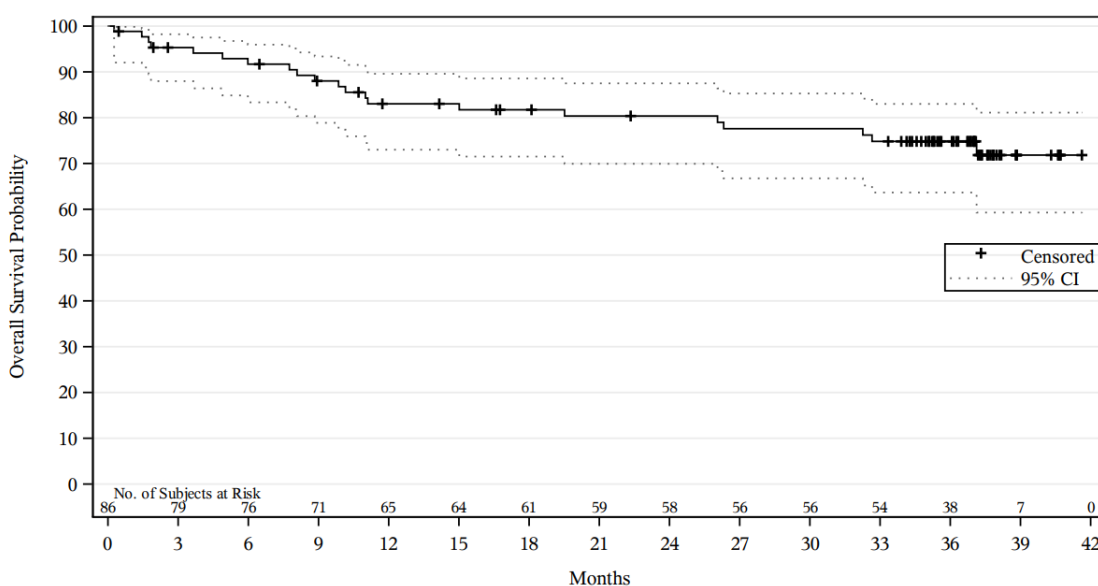
Figure 14: Kaplan-Meier plot of OS in BGB-3111-206 (full trial population)
