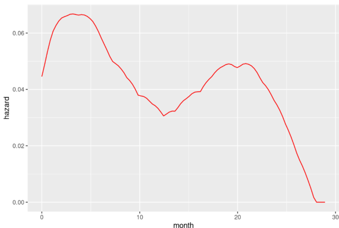
Figure 27: Smoothed hazard plot for ibrutinib (pooled RAY-MCL1001, SPARK and PCYC-1104, N=370)
