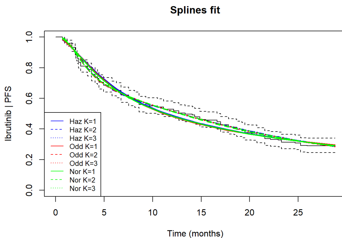
Figure 39: Spline model fit over trial length (ibrutinib PFS)
