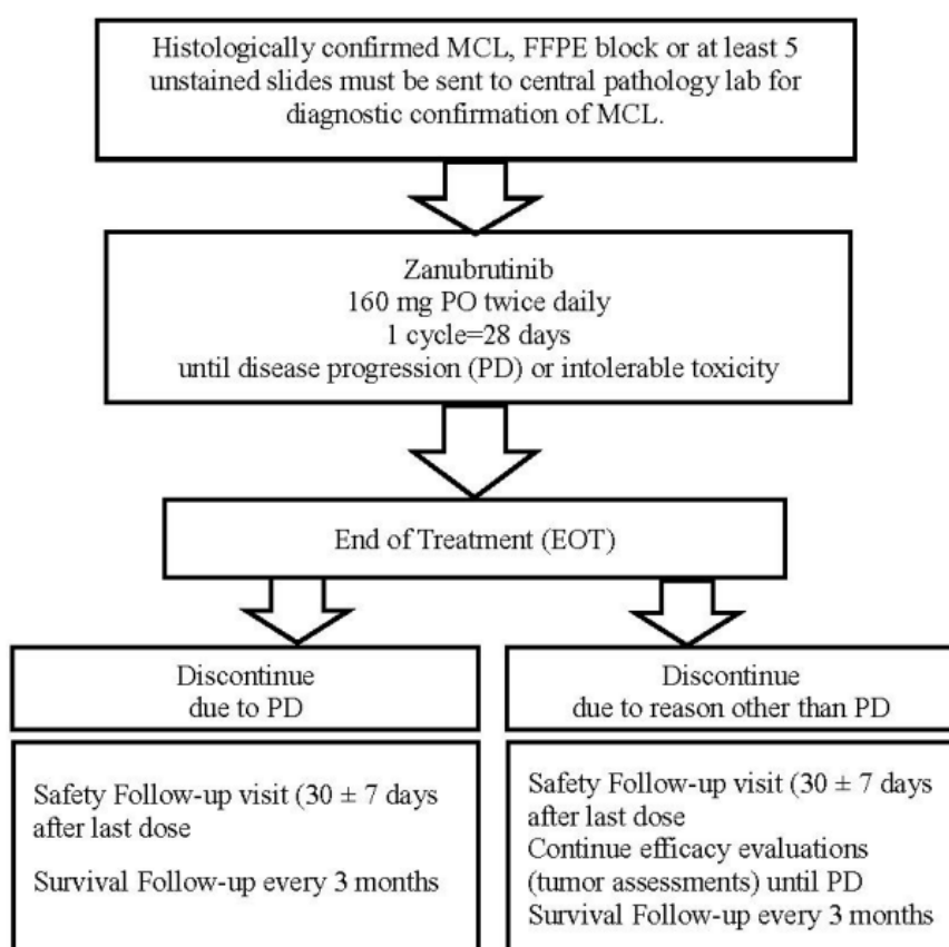
Figure 9: BGB-3111-206 schematic and design
