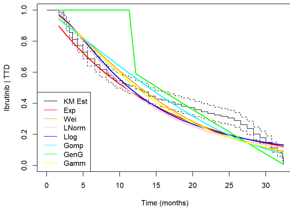
Figure 46: Parametric model fit over trial length (ibrutinib TTD)
