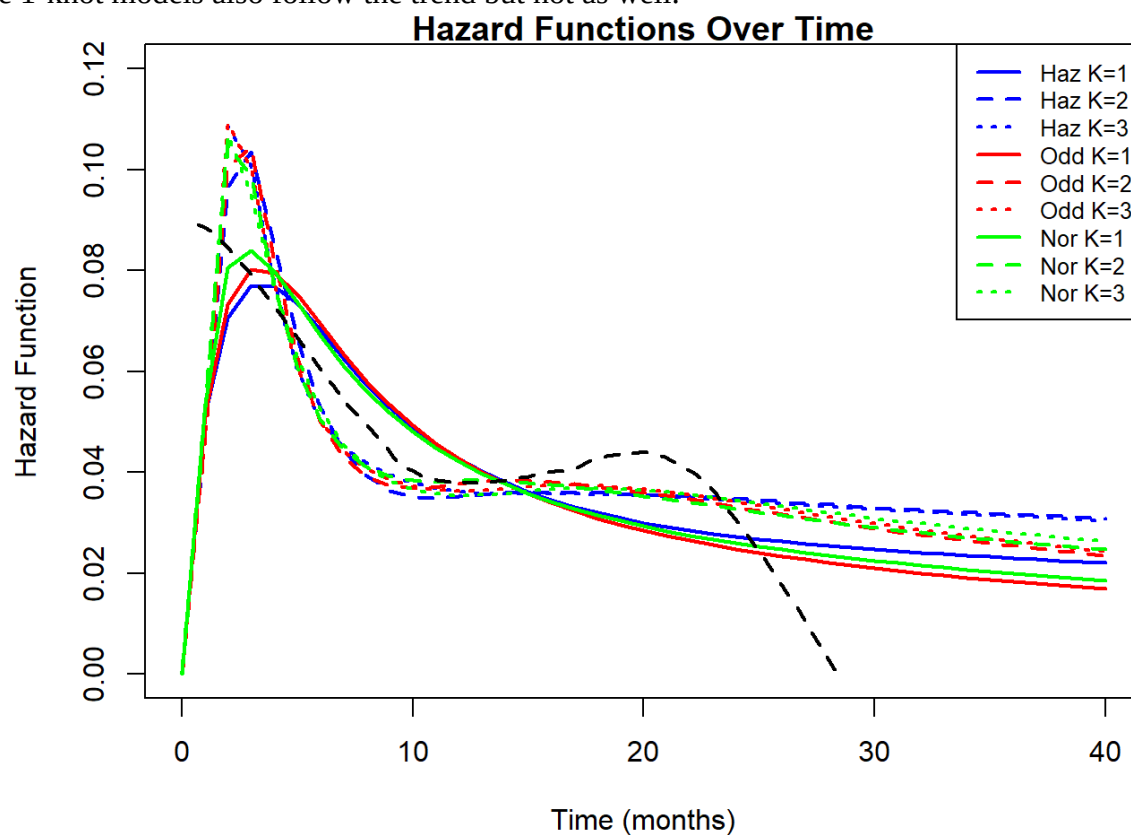
Figure 40: Spline model hazard functions with observed hazards overlaid in black (ibrutinib PFS)
