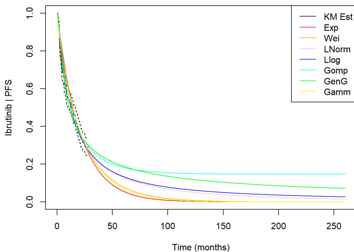
Figure 37: Parametric model fit over 20 years (ibrutinib PFS)
