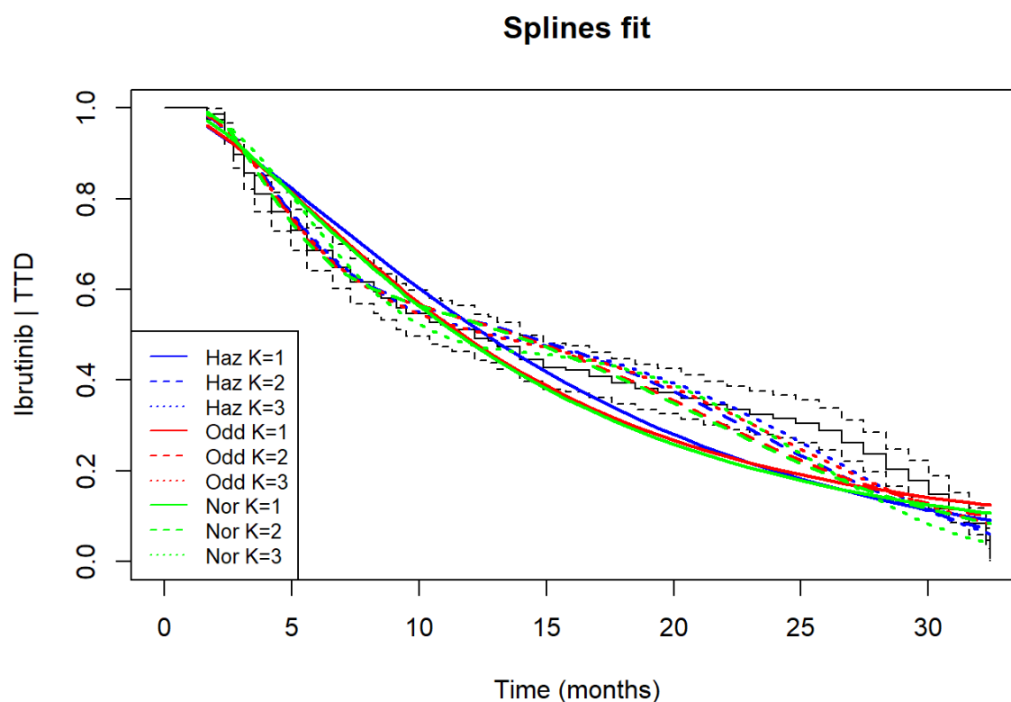
Figure 48: Spline model fit over trial length (ibrutinib TTD)
