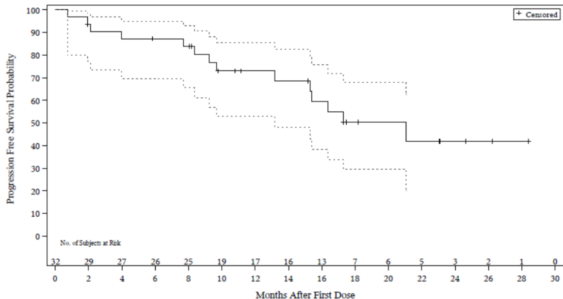
Figure 2: Kaplan-Meier plot of PFS by IRC in BGB-3111-AU-003 (full trial population)
