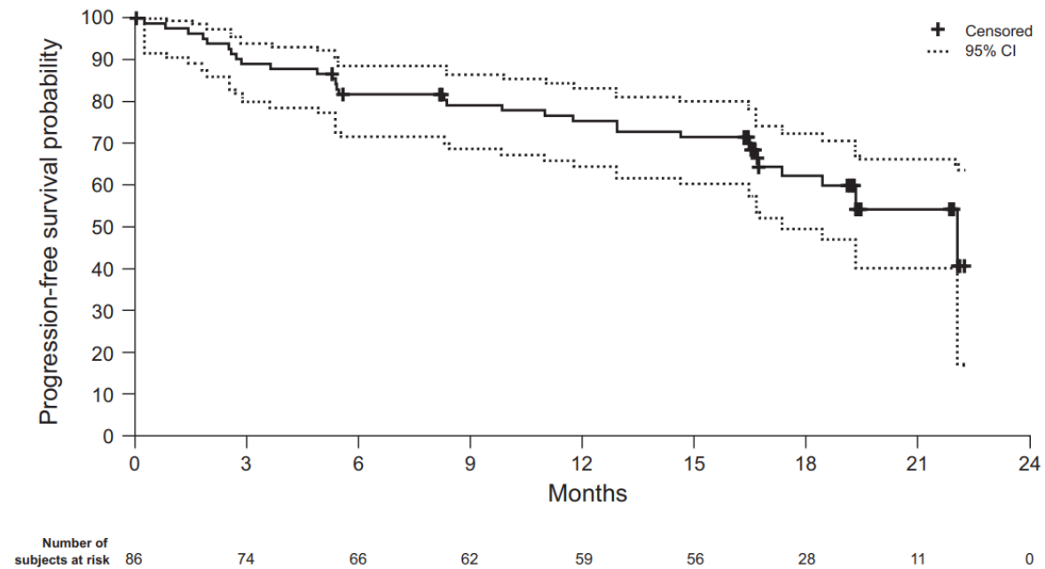
Figure 10: Kaplan-Meier plot of PFS by IRC in BGB-3111-206 (full trial population)
