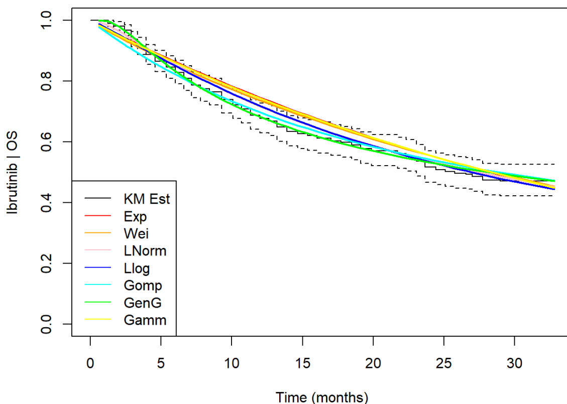
Figure 41: Parametric model fit over trial length (ibrutinib OS)
