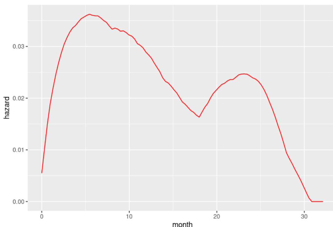
Figure 31: Smoothed hazard plot for OS– ibrutinib (pooled RAY-MCL1001, SPARK and PCYC-1104, N=370)
