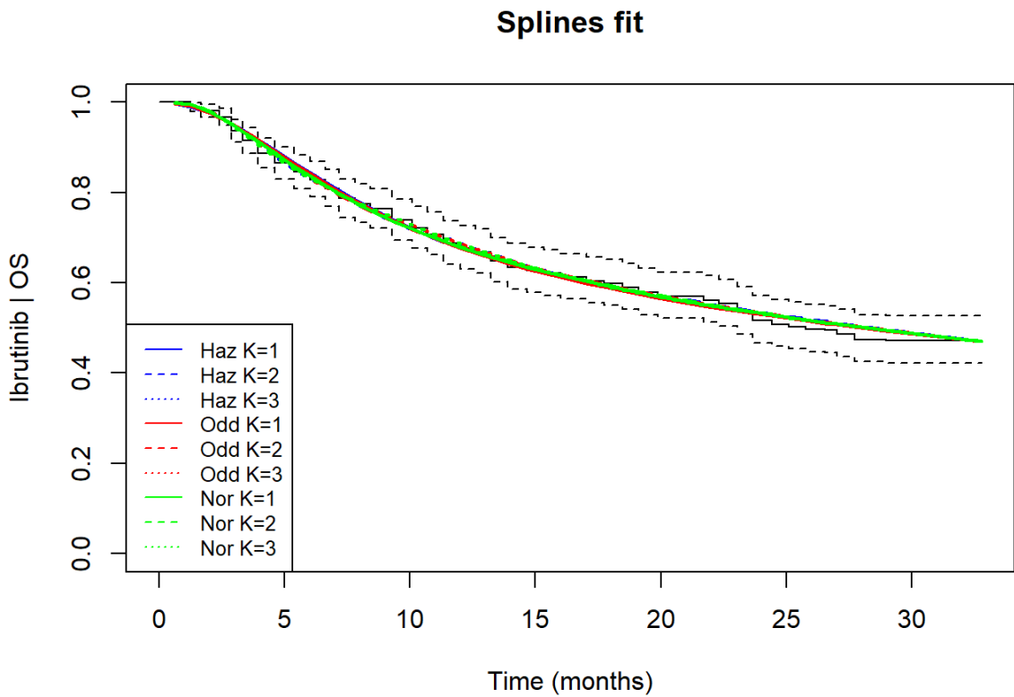
Figure 44: Spline model fit over trial length (ibrutinib OS)
