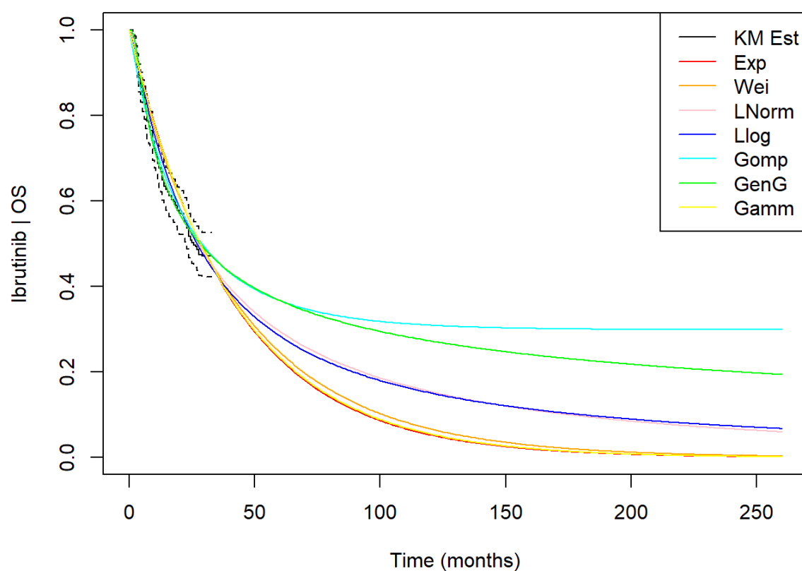
Figure 42: Parametric model fit over 20 years (ibrutinib OS)
