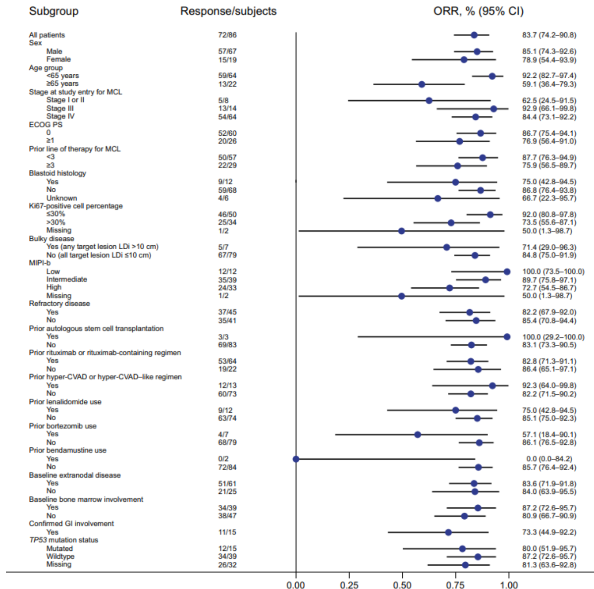
Figure 16: Forest plot of ORR by IRC assessment
