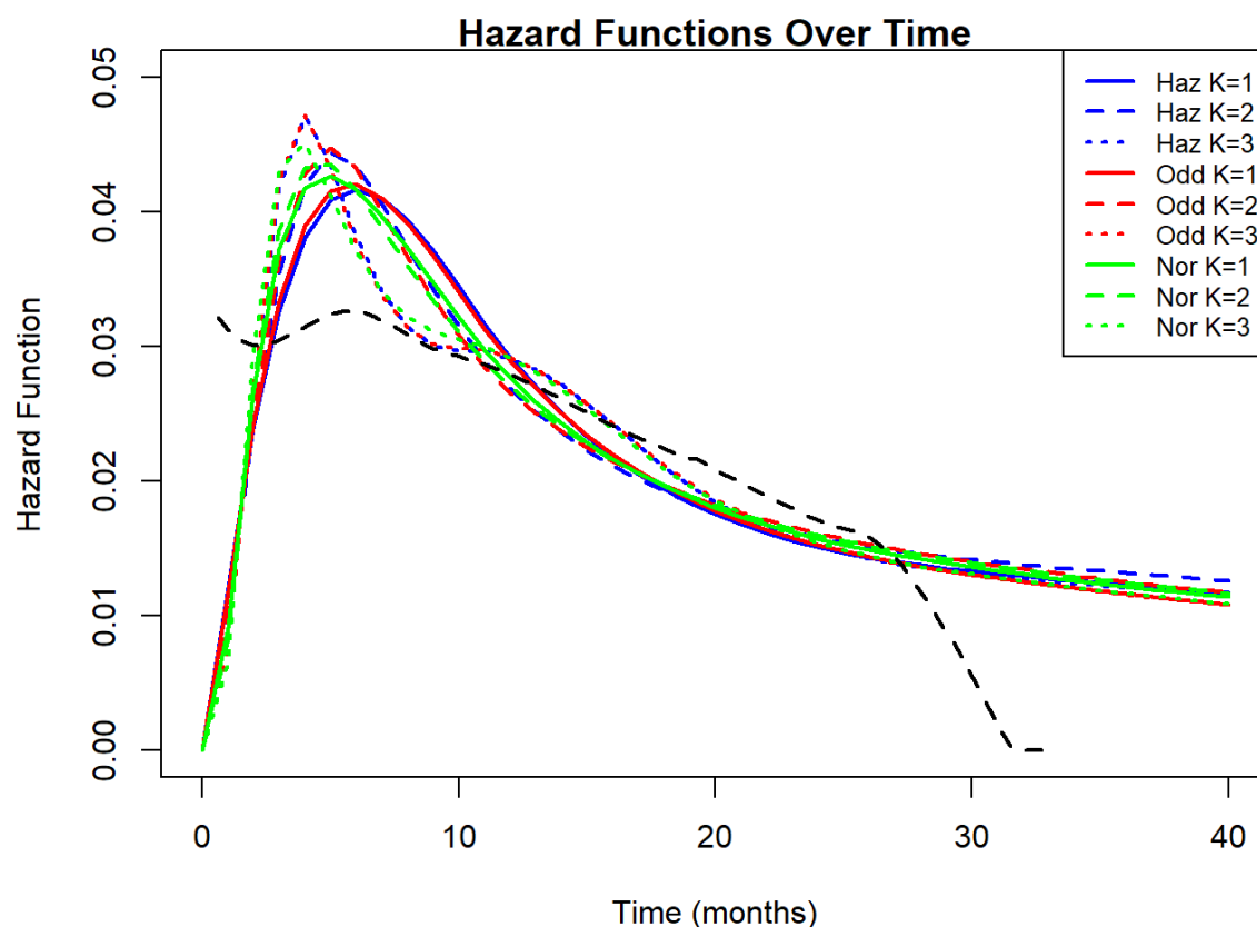
Figure 45: Spline model hazard functions with observed hazards overlaid in black (ibrutinib OS)
