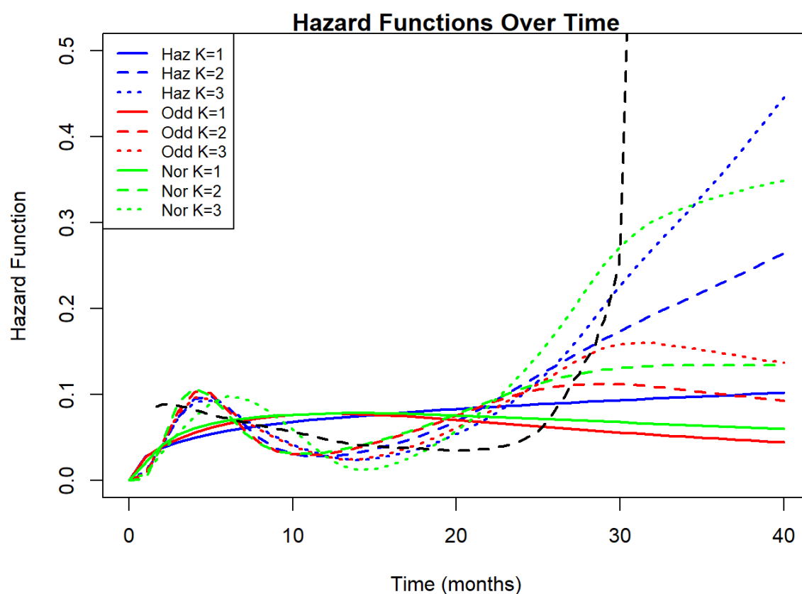
Figure 49: Spline model hazard functions with observed hazards overlaid in black (ibrutinib TTD)
