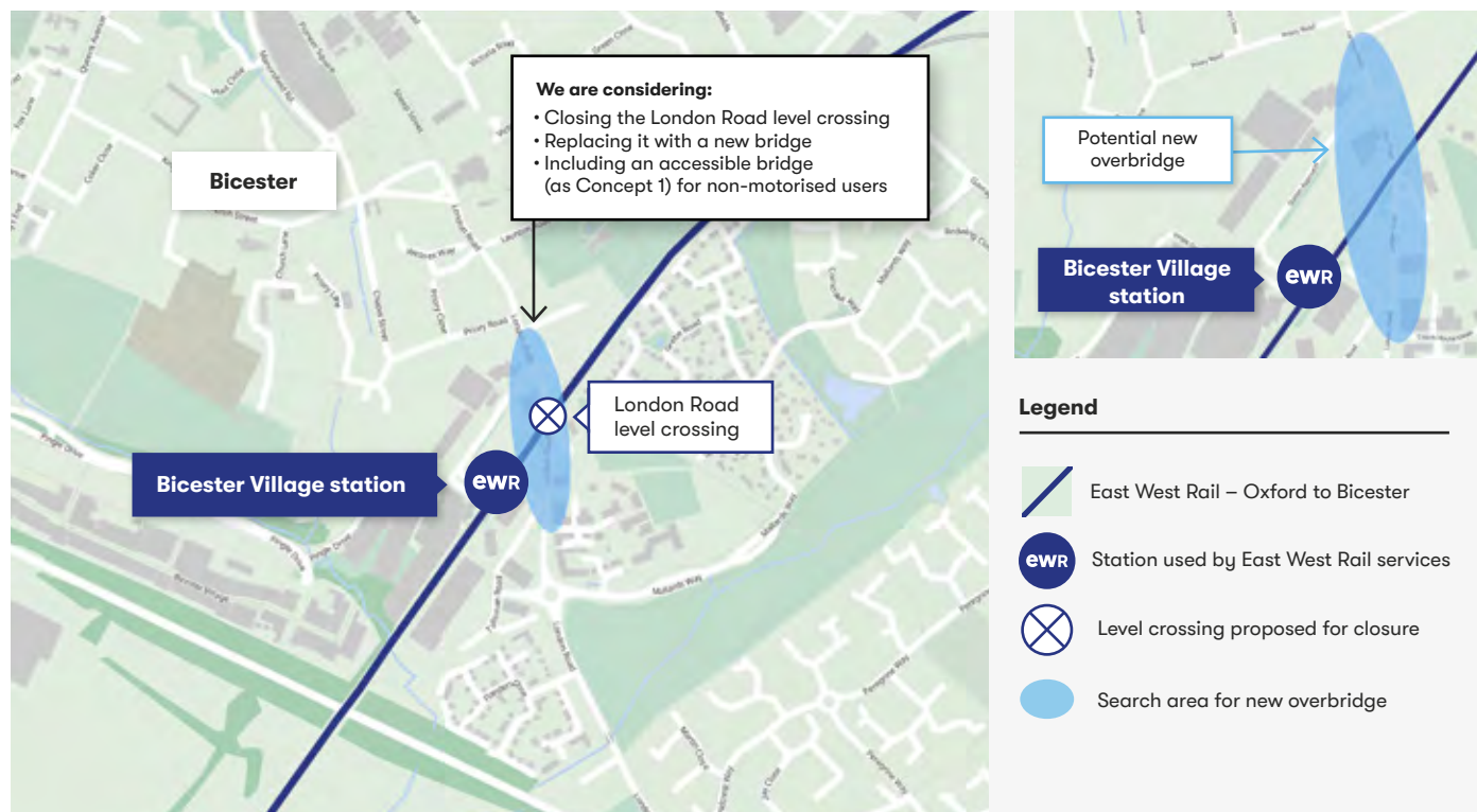
Figure: Concept 3: road bridge
