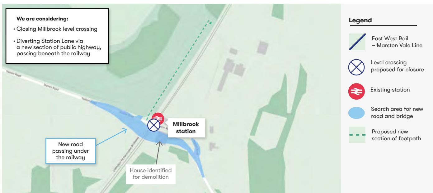
Figure: Option 2: new road underpass south west of Millbrook station
