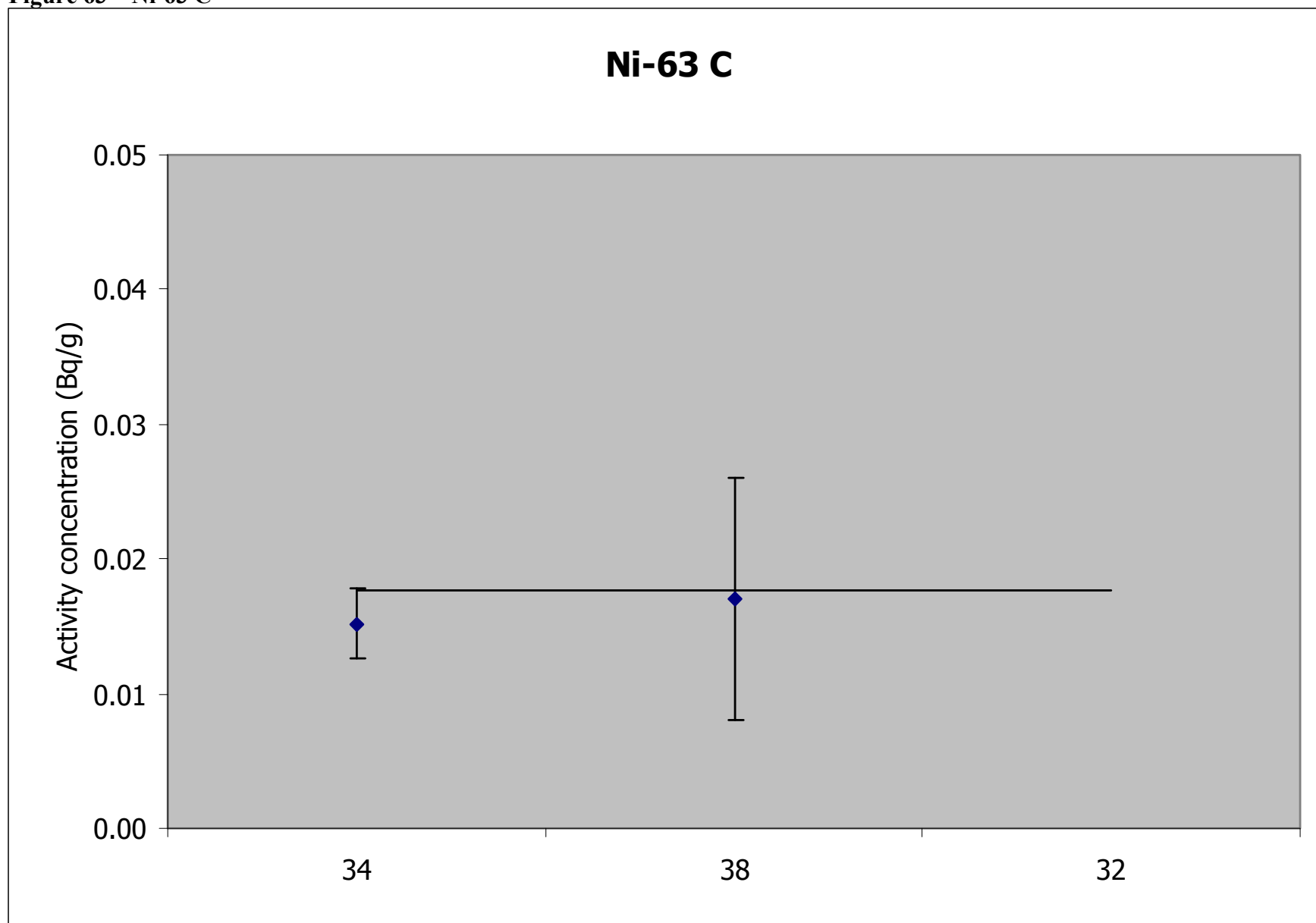
Figure 63 – Ni-63 C
