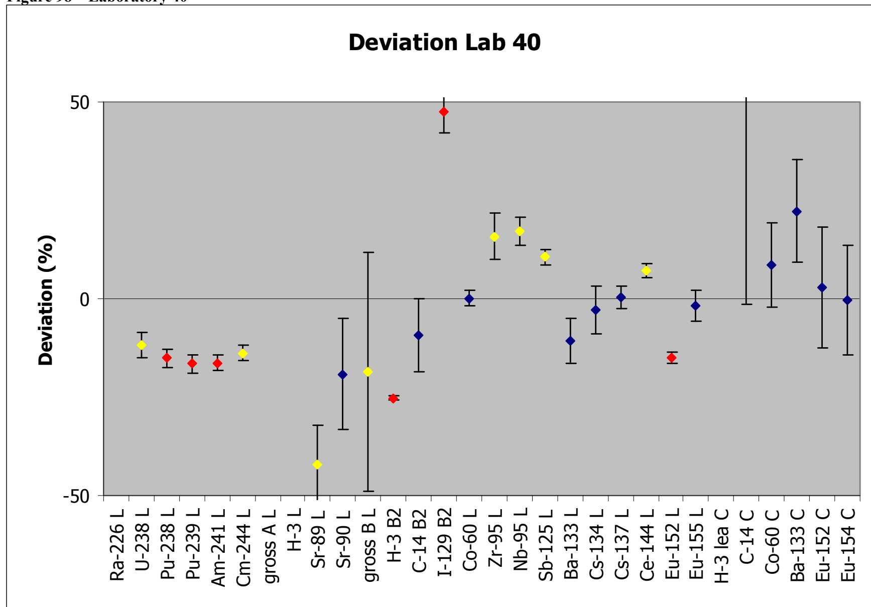
Figure 98 – Laboratory 40
