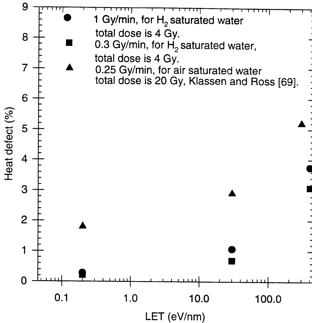
Figure 5.3: Variation of the heat defect with LET.
