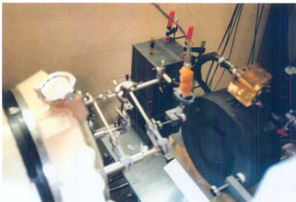
Figure 6.7: Picture of NE2561 chamber calibrated by direct comparison with the primary standard graphite calorimeter.
