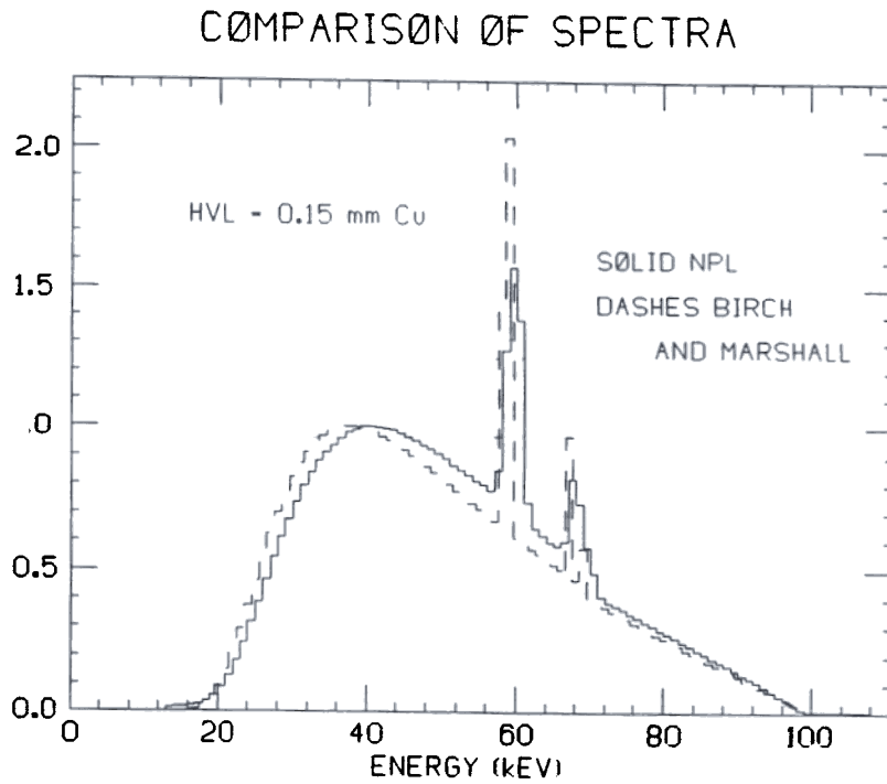
Figure 4.4a Comparison of measured NPL and computed Birch and Marshall spectra for X-rays generated at 100 kV.
