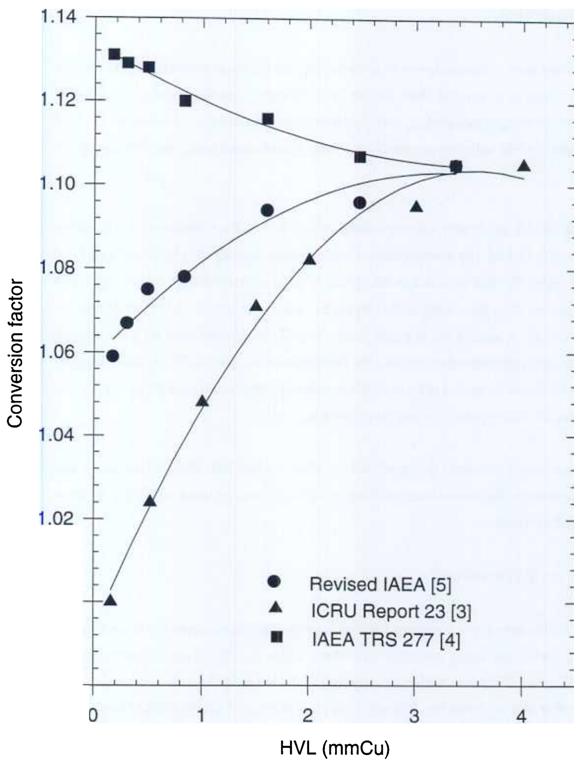
Figure 1.1 Comparison of the factors to convert the air kerma measured using an ionization chamber to absorbed dose to water at 5 cm deep in water
