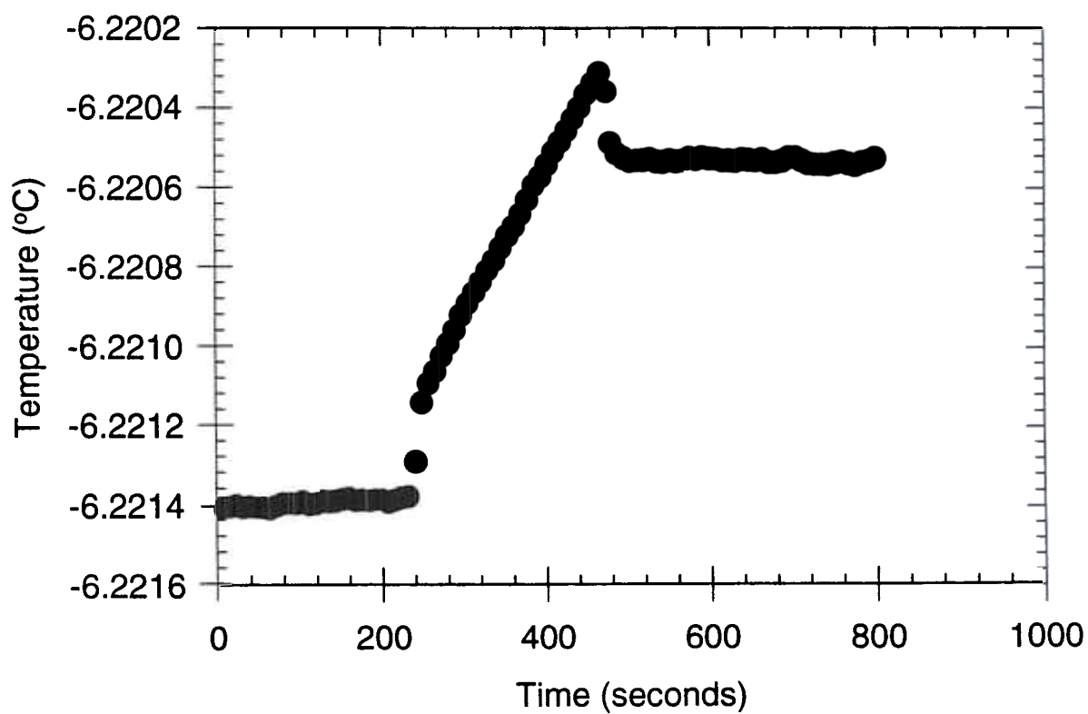
Figure 6.6: Summation of 30 ice calorimeter runs, when irradiated with ^{60}\text{Co} gamma rays.
