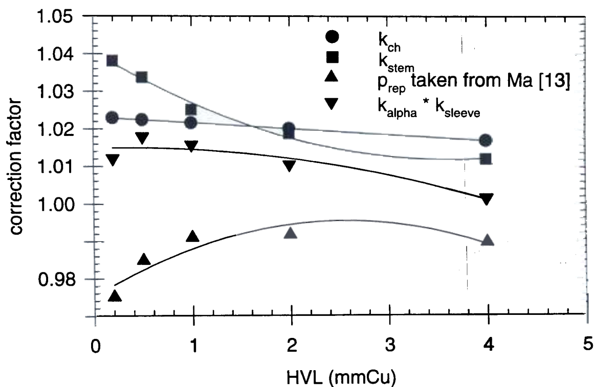
Figure 3.11: Components of k_{ch} for a NE2561 chamber, irradiated with a 10 x 10 cm field.
