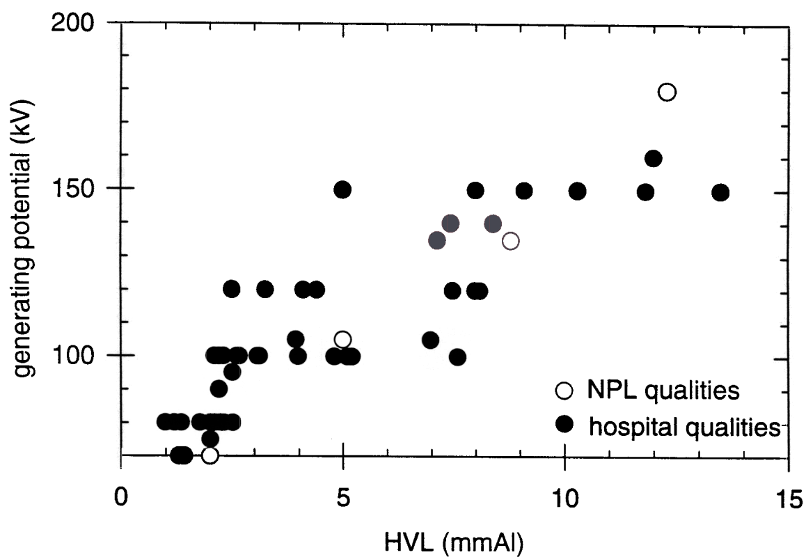
Figure 4.6: To show the variation of HVL with generating potential for 26 radiotherapy centres throughout the U.K.
