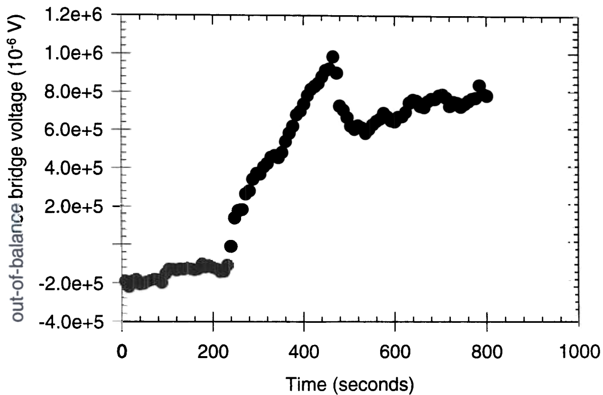
Figure 6.5: A typical ice calorimeter run using ^{60}\text{Co} gamma rays.
