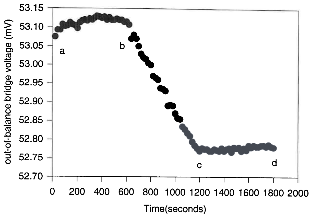
Figure 5.6: A typical water calorimeter irradiation at 3Gy/min for a total dose of 30 Gy, using Co-60 gamma rays.
