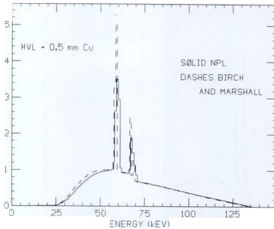
Figure 4.4c Comparison of measured NPL and computed Birch and Marshall spectra for X-rays generated at 135 kV.
