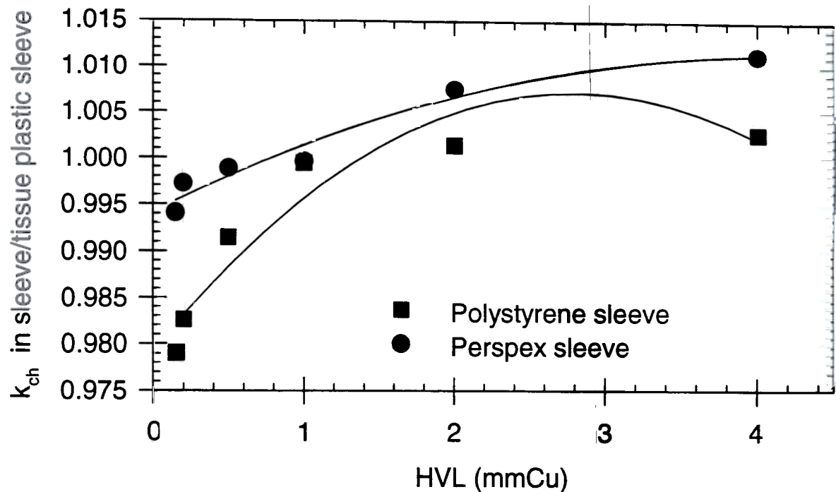
Figure 3.9a: Comparison of sleeves when a NE2561 is calibrated in air without a sleeve.
