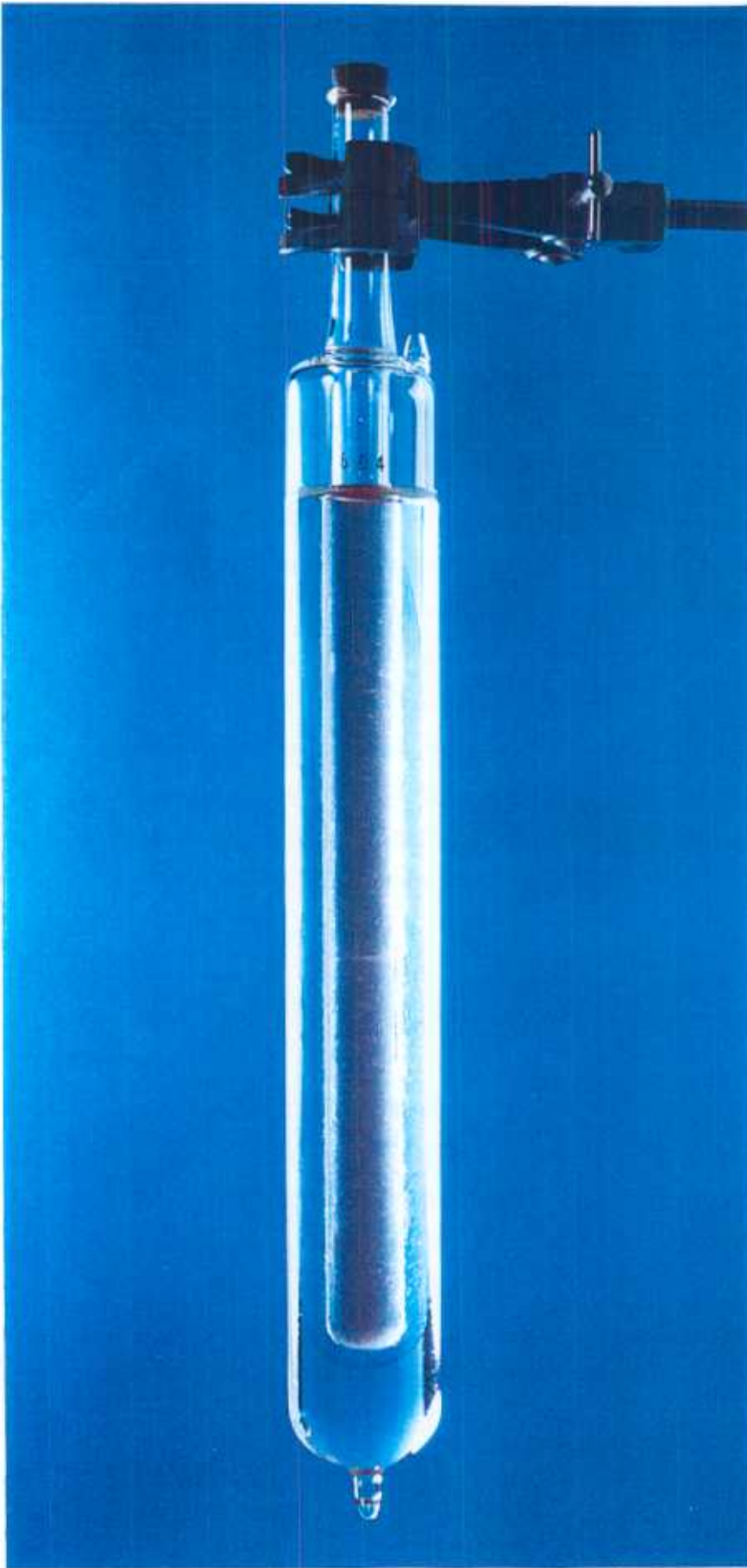
Figure 5.5 Picture of a water triple point cell
