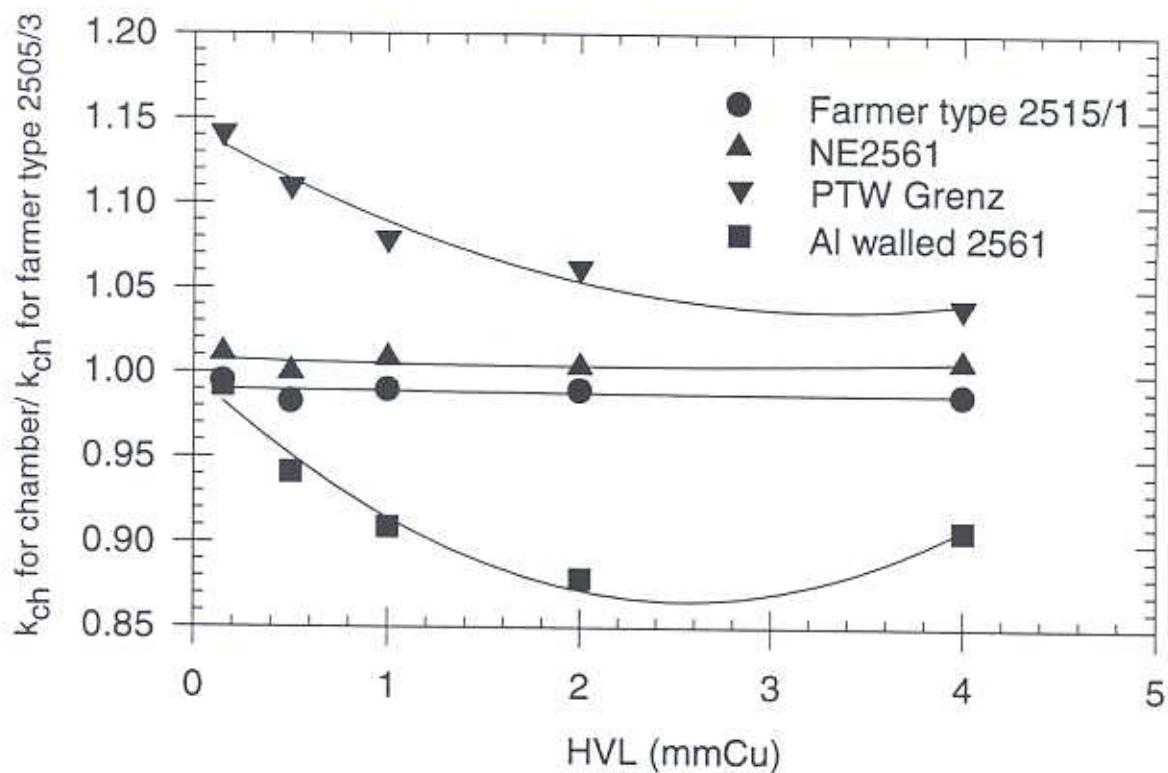
Figure 3.5: Comparison of chamber correction factors.
