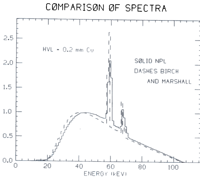
Figure 4.4b Comparison of measured NPL and computed Birch and Marshall spectra for X-rays generated at 105 kV.
