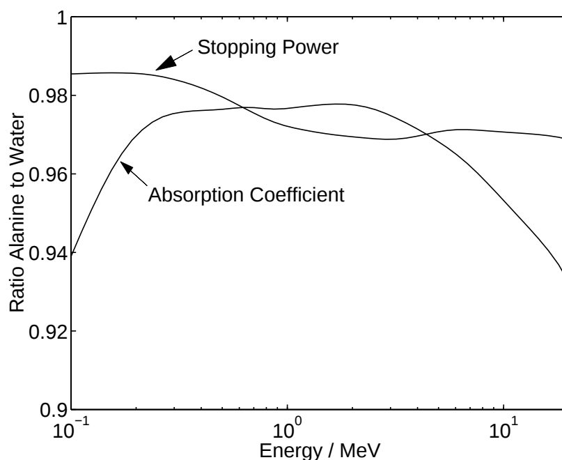
Figure 1 Ratio of alanine mass energy absorption coefficients and mass collision stopping powers to those of water, as a function of energy.
