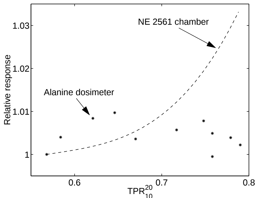
Figure 5 Relative response of alanine dosimeters and ionisation chambers in high energy photon beams
