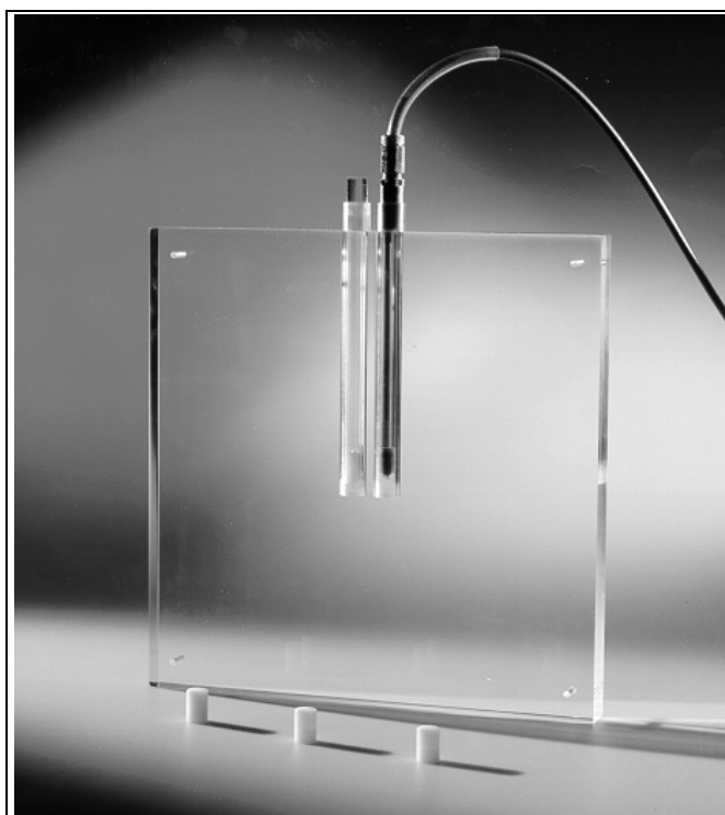
Figure 4 Phantom plate showing interchangeable locations of ionisation chamber and alanine dosimeter.
