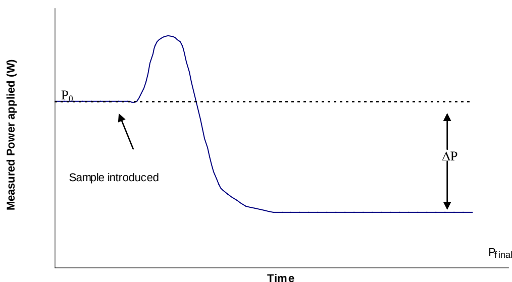
Figure 4 Isothermal Measurement
