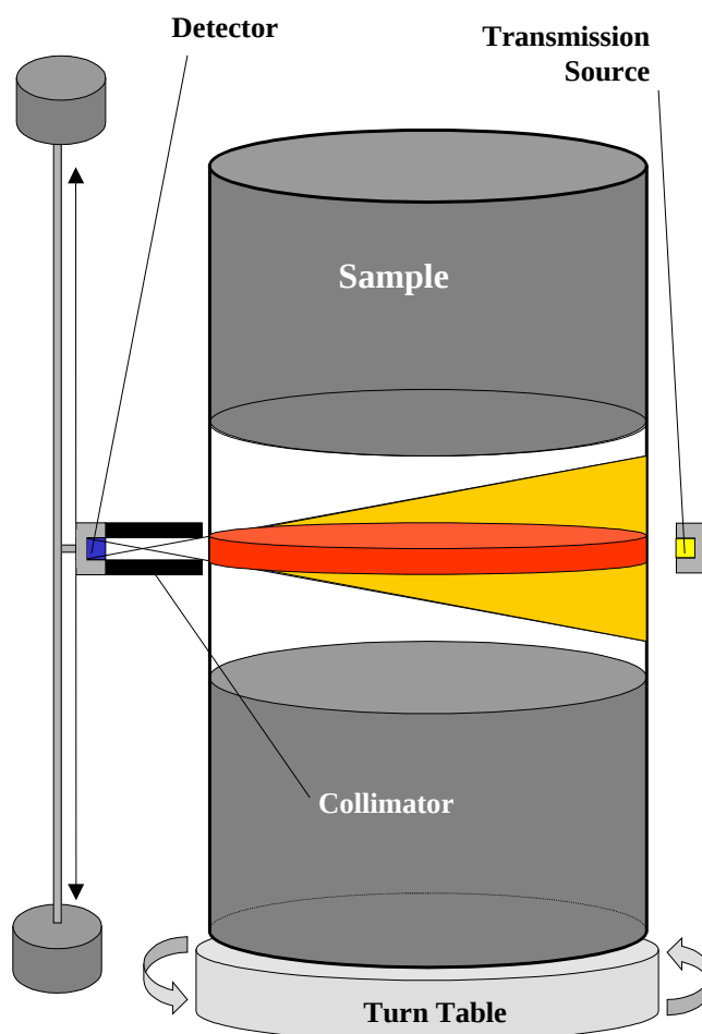
Figure 3 Principal Features of a Segmented Gamma Scanner
