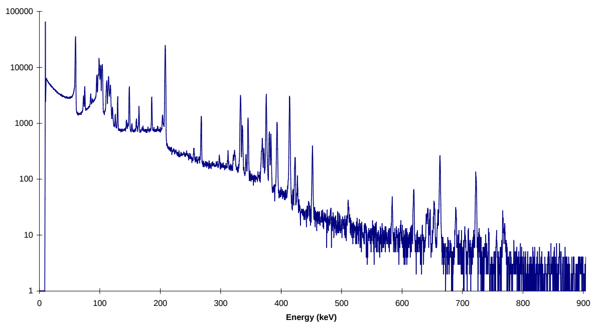
Figure 2 Typical HRGS Spectrum of Pu
