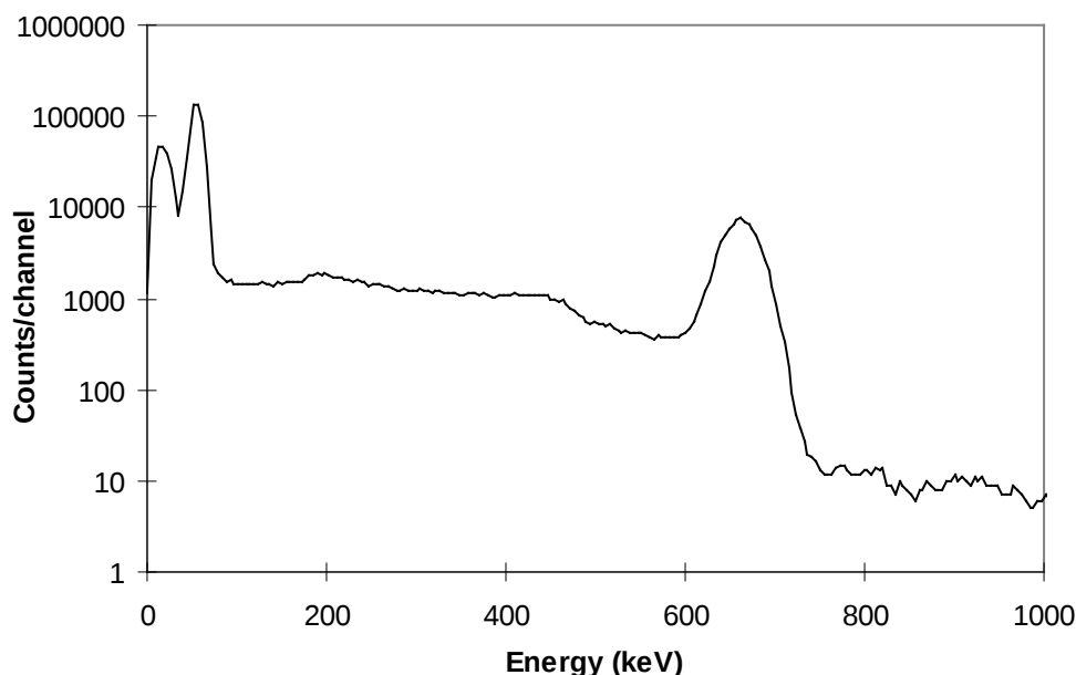
Figure 1 Typical LRGS Spectrum of ^{137}\text{Cs}
