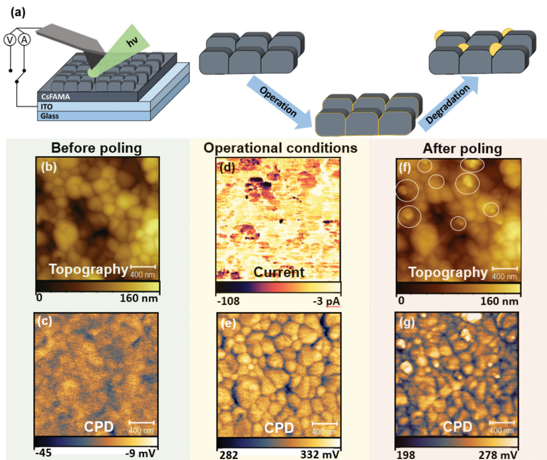
Fig. 1 Experimental setup and perovskite sample surface before and after charge injection with metal-coated AFM probe. (a) Schematic of the experimental setup used for photoconductive AFM, where current between the metalised AFM probe and the ITO substrate is recorded. Illustration of morphological evolution across the experiments. (b) AFM topography before poling; (c) SKPM map before poling (dark); (d) pc-AFM measurement at -0.5 V bias and illumination using a 532 nm laser diode at 80 \text{ mW cm}^{-2} ; (e) SKPM under illumination before tip-sample poling; (f) AFM topography after pc-AFM measurement (g) SKPM after poling (dark). Circles in (f) highlight formation of grain-like features after pc-AFM.
