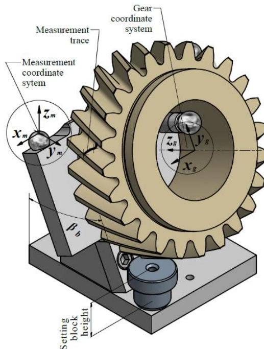
Figure 16. Example fixture to approximately align the gear surface with the measuring instrument co-ordinate system.
