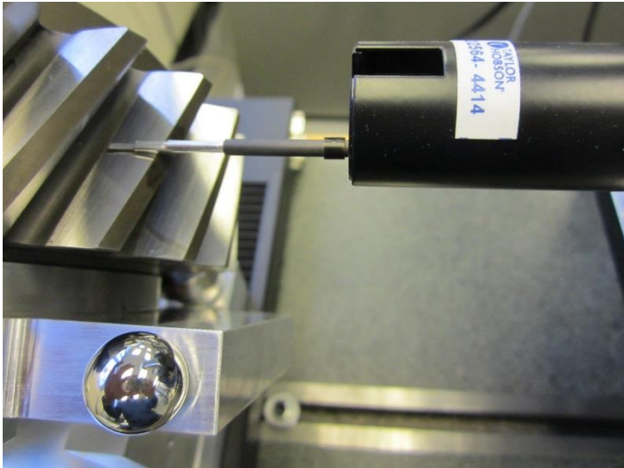
Figure 17. An alignment fixture used to locate a small test gear and ensure the contact stylus is approximately normal to the gear surface.
