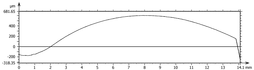
Figure 19. Illustration of one continuous profile measured with a general surface texture instrument from tooth root to tip.
