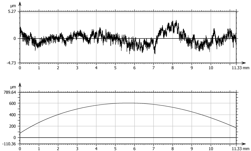
Figure 20. The residual deviations of a ground gear flank containing linear tip relief after form removal with a fifth order polynomial. Top, residual with form removed. Bottom, form has been removed.
