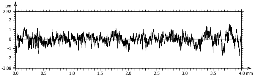
Figure 22. The roughness profile of a section of a gear flank, with an Ra of 0.41\text{ }\mu\text{m} .
