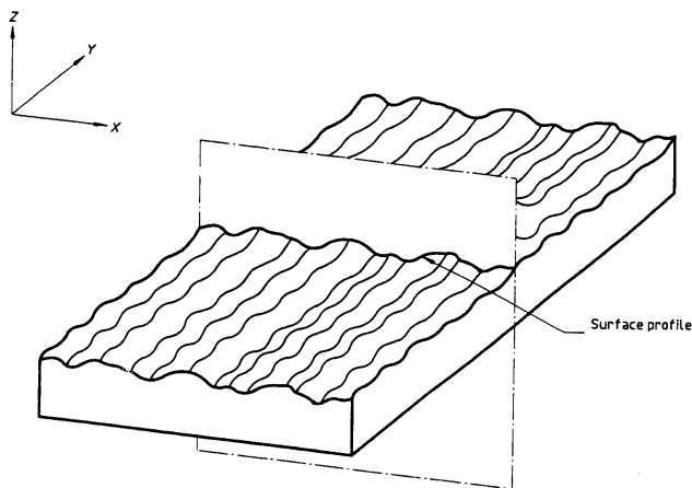
Figure 13. Surface profile and co-ordinate system defined by BS ISO 4287 [20].
