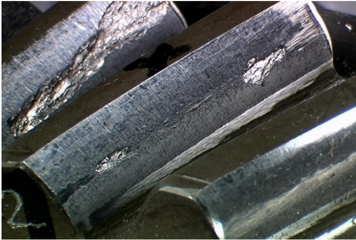
Figure 8. Macro-pitting fatigue damage on gear teeth.
