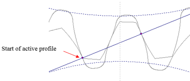
Figure 2. Gear positions at the start of active profile (part of a tooth which contacts the tooth flanks of a mating gear along the line of action). The upper gear has a higher rolling velocity than the lower gear at the start of the active profile (SAP), leading to a large sliding action.
