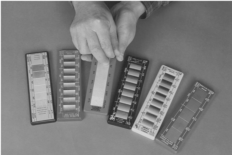
Figure 23. A standard set of comparison specimens, courtesy of Rubert & Co Ltd.
