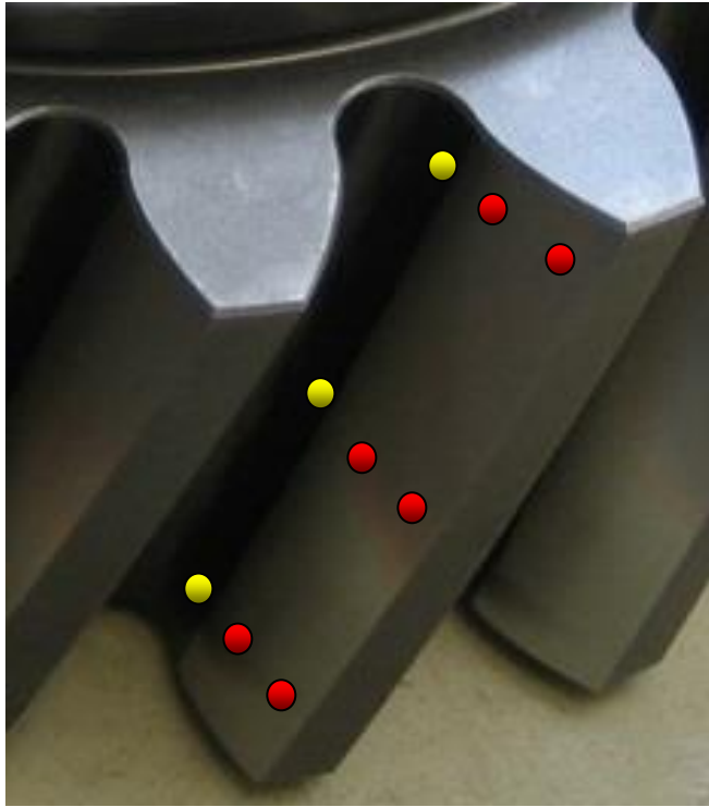
Figure 18. Measurement positions: six (red) in the active flank region and three (yellow) in root region.
