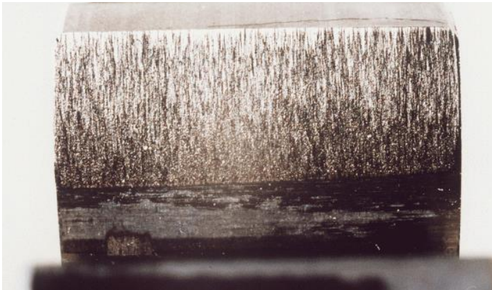
Figure 11. Scuffing (scoring) caused by lubricant failure leading to welding and sliding of the mating gear tooth flanks.
