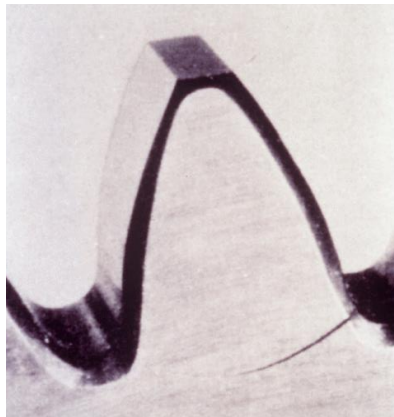
Figure 9. Gear bending fatigue failure initiated in the root fillet radius.
