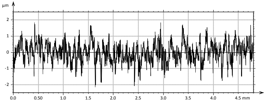
Figure 25. Example of levelled primary profile.
