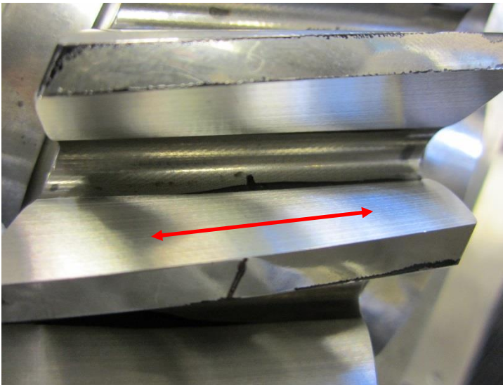
Figure 5. Grinding lay from a gear form grinding machine.
