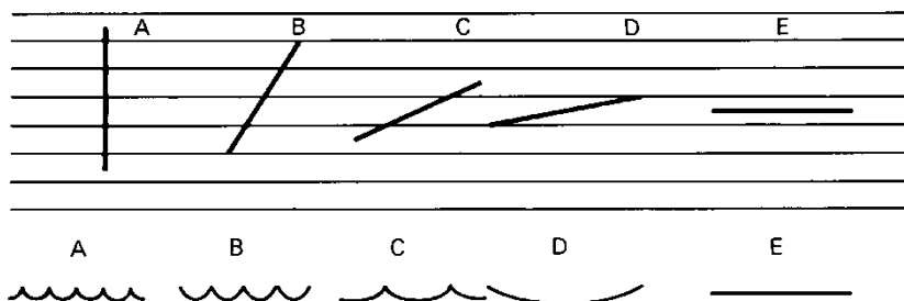
Figure 14. The effect of measuring in different directions to the surface lay, courtesy of Taylor Hobson Ltd. Note that the direction of lay runs across the page.
