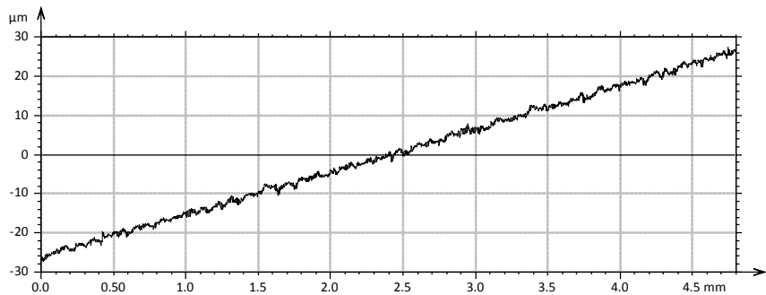
Figure 24. Example of measured profile at an angle of 12 degrees which corresponds to the maximum tilt angle incurred during the gear face/flank measurement.
