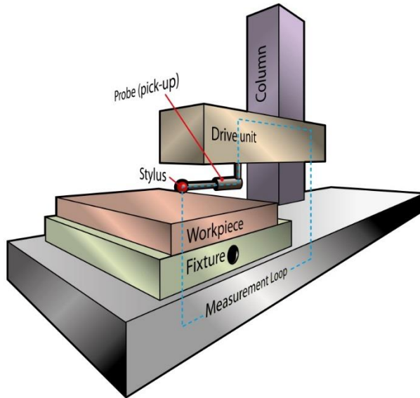
Figure 15. Elements of the typical stylus instrument, from BS EN ISO 3274 [24].
