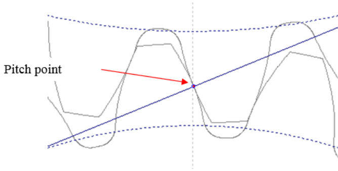
Figure 3. Gear positions at the pitch point, which lies on the line between the two gears where sliding speed is zero. The action is purely rolling as they both have the same rolling velocity at this time.
