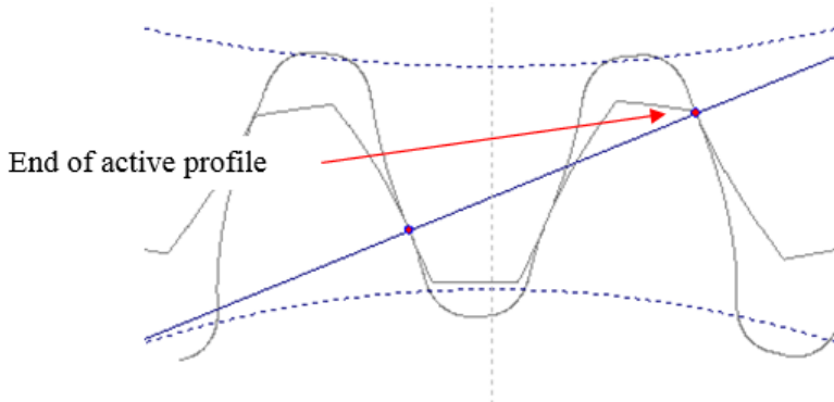
Figure 4. Gear positions at the end of active profile. The upper gear has a lower rolling velocity than the lower gear at the end of the active profile (EAP), again leading to a sliding action.
