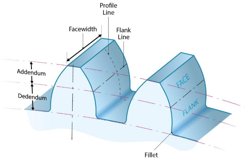
Figure 1. Gear geometry vocabulary relevant to the measurements covered by this guide.
