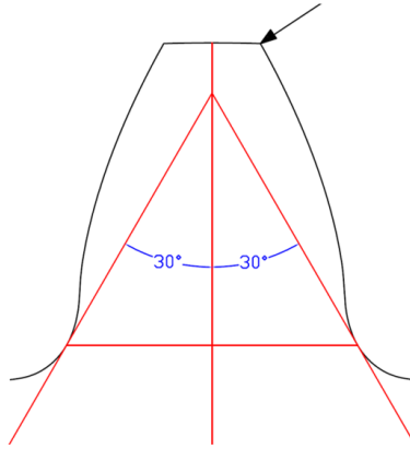
Figure 10. 30° tangent position for root fillet roughness measurement at the predicted region of maximum bending stress in BS ISO 6336-3 [16]. The arrow is the applied load.
