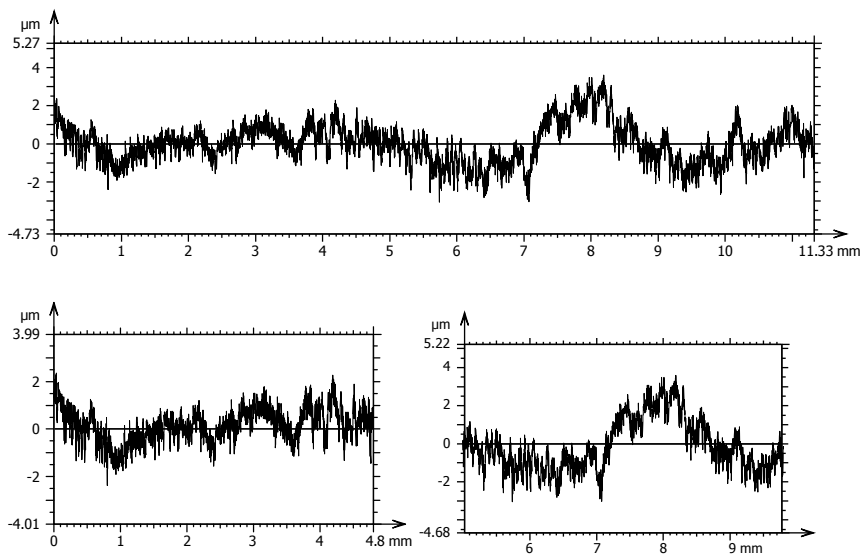
Figure 21. Multiple sections can be extracted from a single primary profile to see how roughness parameters vary along the profile. Top, residual profile with form removed. Bottom left, first section of data chosen for evaluation. Bottom right, second section of data chosen for evaluation.
