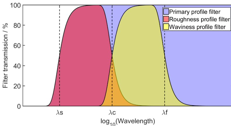
Figure 12. Example Gaussian filters for the primary, roughness and waviness profiles. The filters are based on BS ISO 4287:1997 [20] and BS EN ISO 11562:1997 [21].
