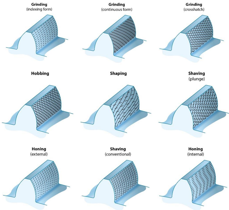
Figure 6. Common gear manufacturing processes and lay directions. Reproduced from BS ISO TR 10064-4 [3].
