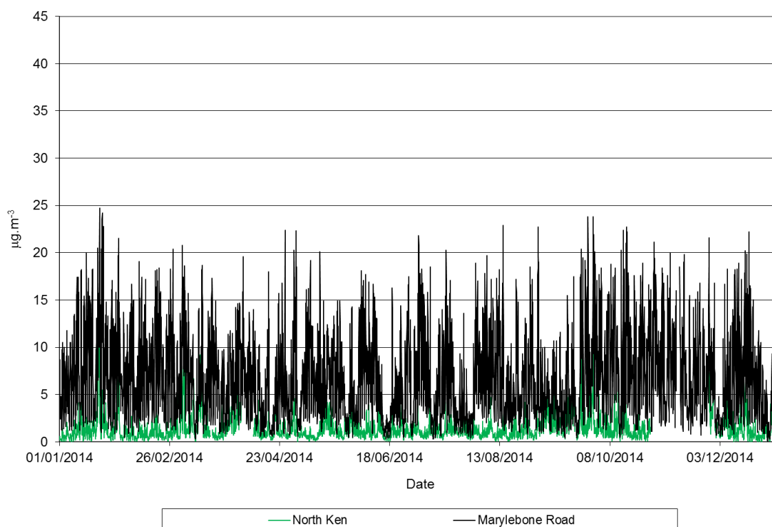
Figure 7 Black Carbon concentrations during 2014 in Southern and Eastern England
