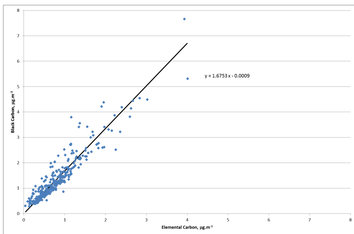
Figure 26 2014 EC and BC Measurements at North Kensington
