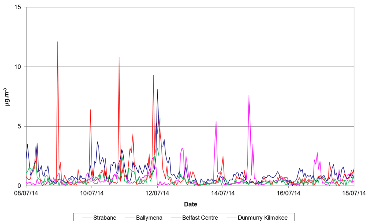
Figure 23 Black Carbon concentrations in Northern Ireland around the period of 12 th July
