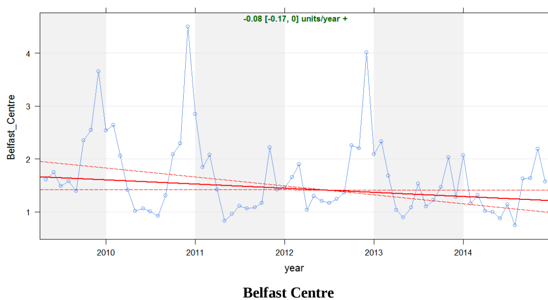
Figure 31 Black Carbon concentrations measured at urban centre sites, 2009 – 2014
