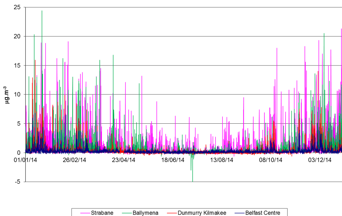
Figure 9 UV component concentrations during 2014 in Northern Ireland
