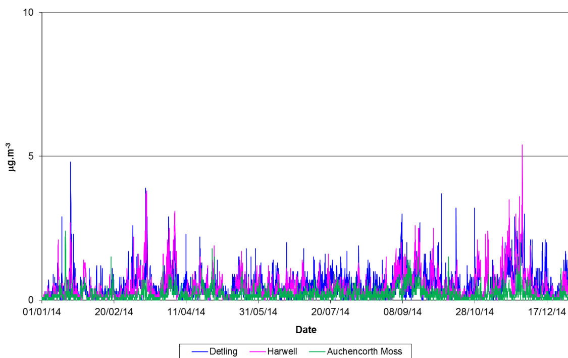
Figure 8 Black Carbon concentrations during 2014 at Rural Locations
