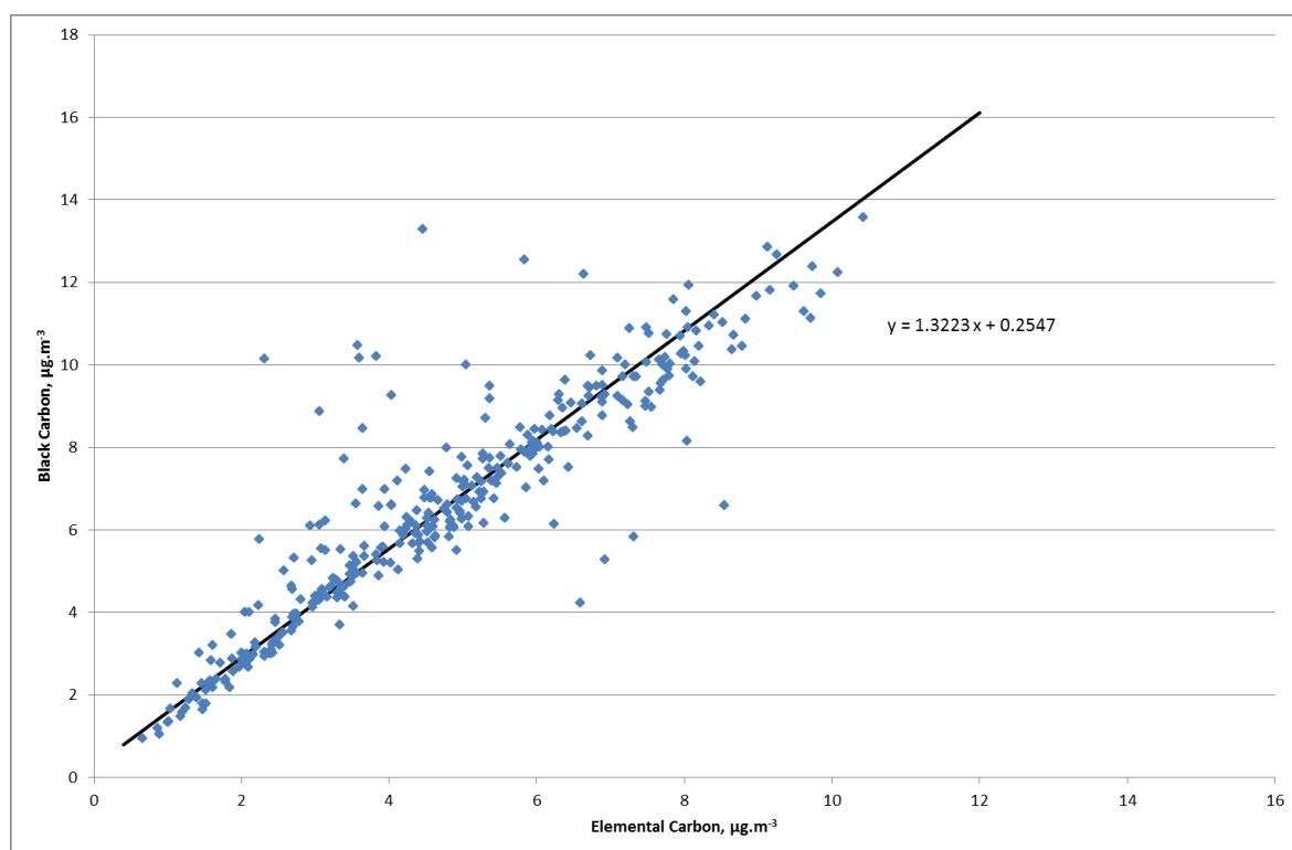
Figure 27 2014 EC and BC Measurements at Marylebone Road
