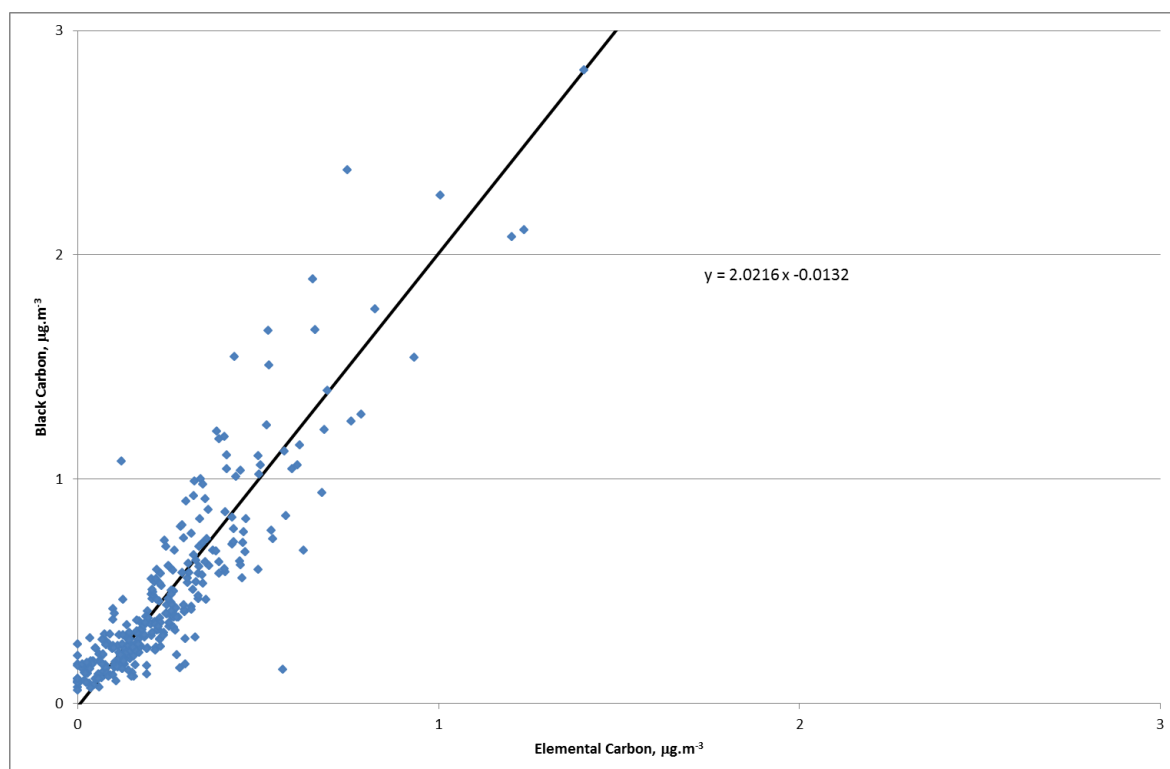
Figure 28 2014 EC and BC Measurements at Harwell
