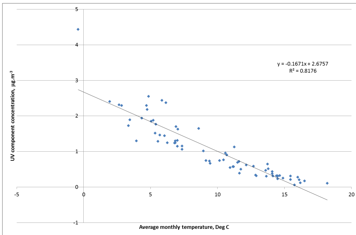
Figure 41 Scatter plot of monthly UV component concentration versus ambient temperature at Strabane over the period 2009 -2013
