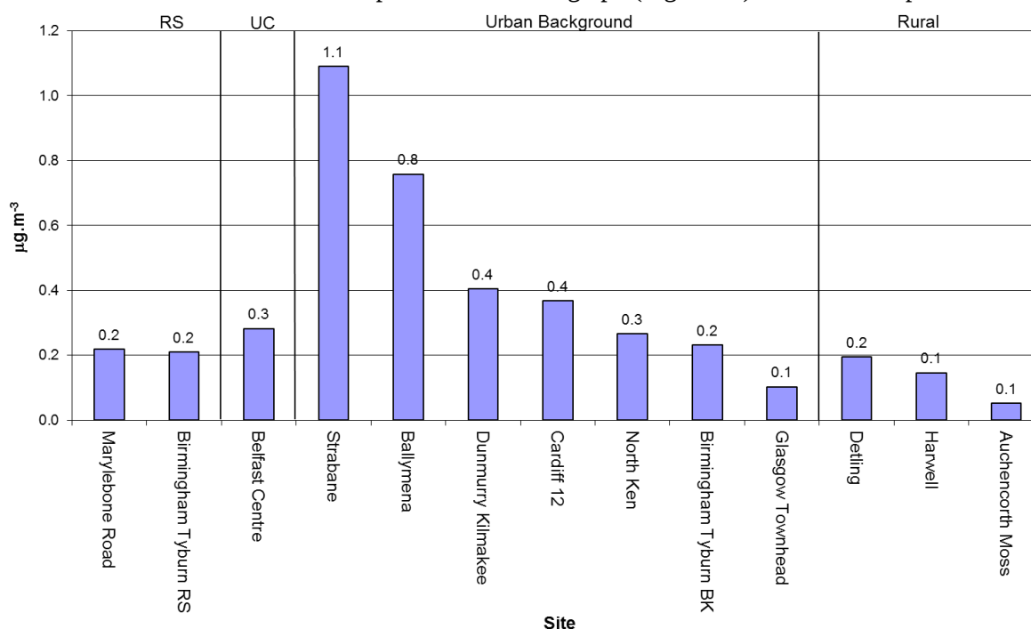
Figure 15 Annual Mean UV component Concentrations for 2014
