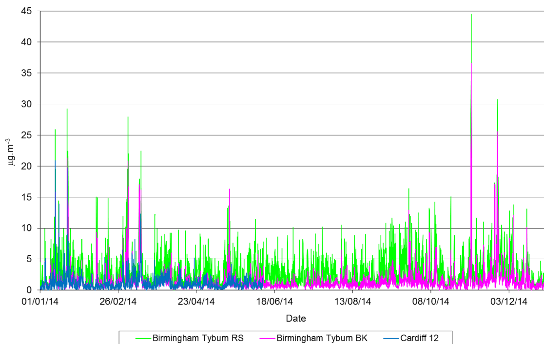
Figure 6 Black Carbon concentrations during 2014 in Wales and the Midlands
