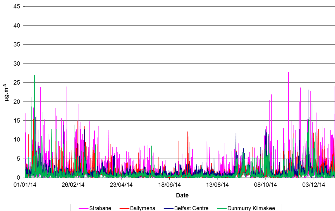
Figure 4 Black Carbon concentrations during 2014 in Northern Ireland
