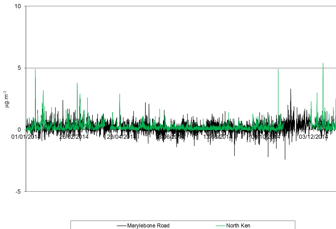
Figure 12 UV component concentrations during 2014 in Southern and Eastern England
