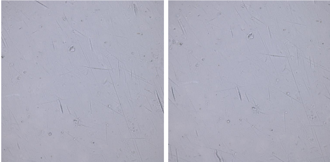
Figure 21. Rhodium plated sample before (left) and after (right) vacuum/humidity cycling.
