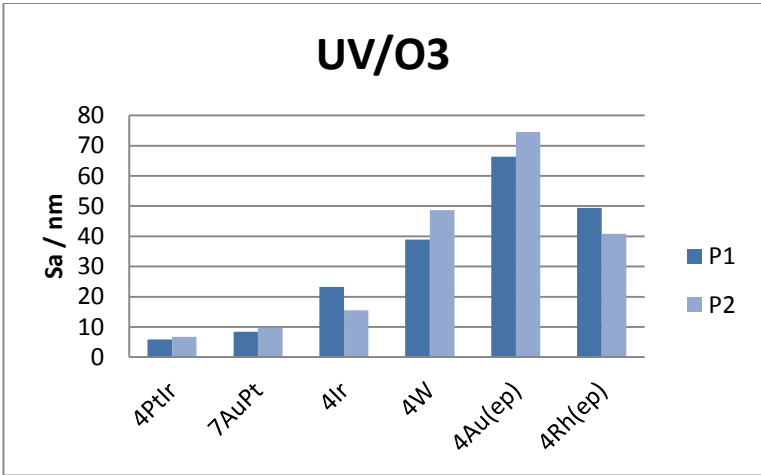
Figure 18. S_a surface roughness values for UV/Ozone cleaned samples (measurements taken at 2 positions, P1 and P2, on the sample surface).
