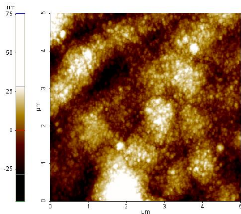
Figure 9. AFM topography image of gold-electroplated copper surface produced by Häfner, taken with a scan size of 5 \mu\text{m} \times 5 \mu\text{m} .
