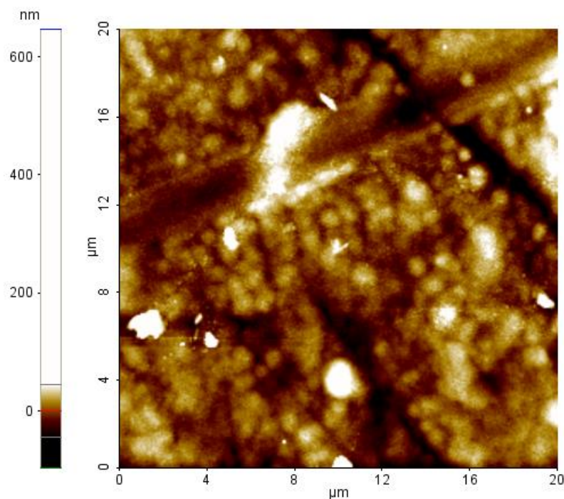
Figure 13. AFM topography image of rhodium-electroplated copper surface produced by Häfner, taken with a scan size of 20 \times 20\text{ }\mu\text{m} .
