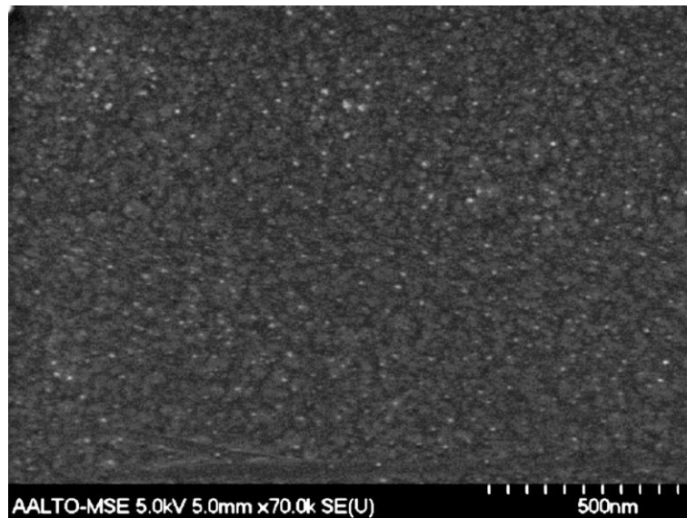
Figure 12. SEM micrograph at \times 70,000 magnification of rhodium-electroplated copper surface produced by Häfner.
