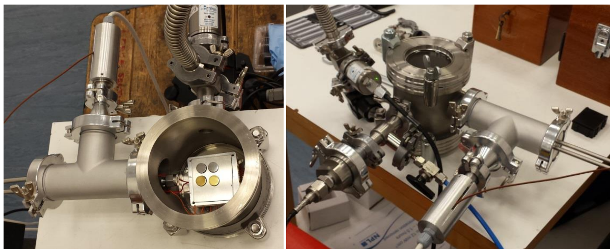
Figure 22. Apparatus used for vacuum/humidity cycling.
