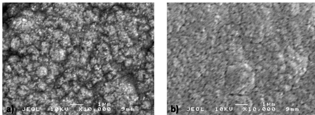
Figures 2a and 2b. ( \times 10,000 ) Scanning electron micrographs of two random locations obtained under identical scan conditions. The difference between the images demonstrates the slight variation of surface structure with position. Au plated from TSG-250 precursor solution on OFHC copper at NRC.
