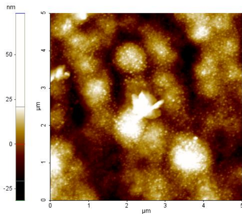
Figure 14. AFM topography image of rhodium-electroplated copper surface produced by Häfner, taken with a scan size of 5 \times 5 \mu\text{m} .
