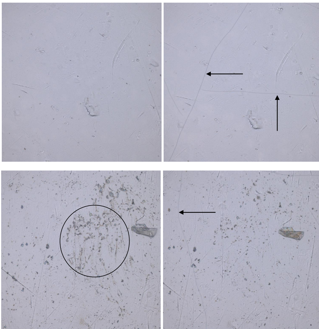
Figure 23. Rhodium plated sample before (left) and after (right) thermal cycling.
