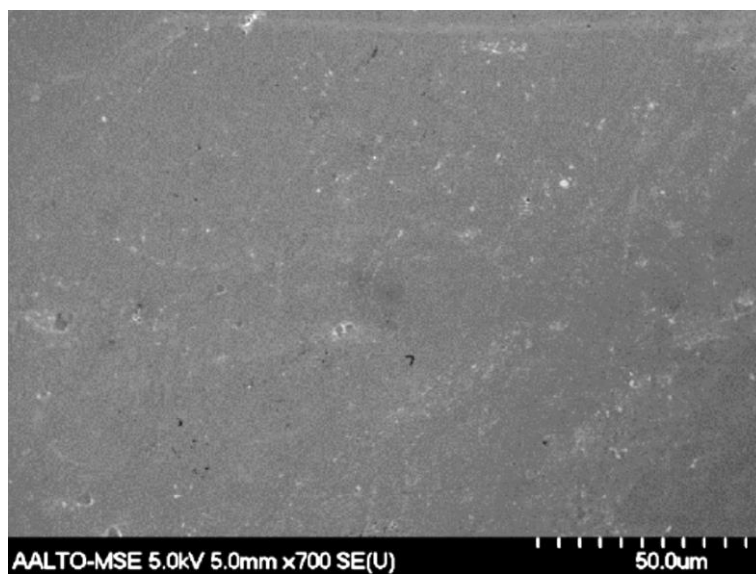
Figure 10. SEM micrograph at \times 700 magnification of rhodium-electroplated copper surface produced by Häfner.
