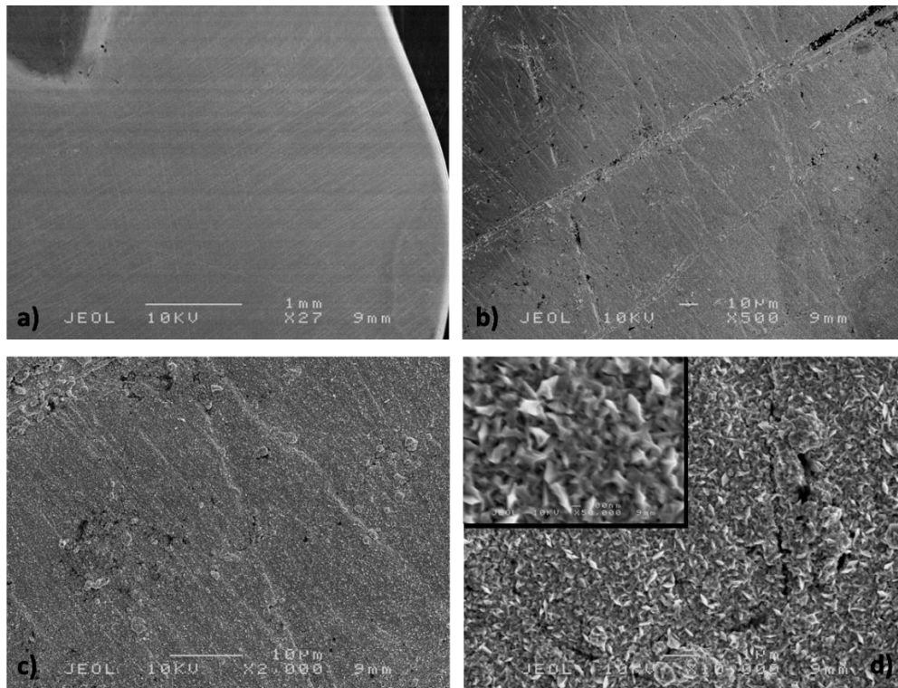
Figures 4a to 4d. Scanning electron micrographs of NRC gold electroplated OFHC copper substrates using Orotemp 24 pure gold as a precursor. The magnifications and scales are shown in the images ( \times 27 , \times 500 , \times 2,000 , \times 10,000 , \times 50,000 for figures a, b, c, d and the inset respectively).
