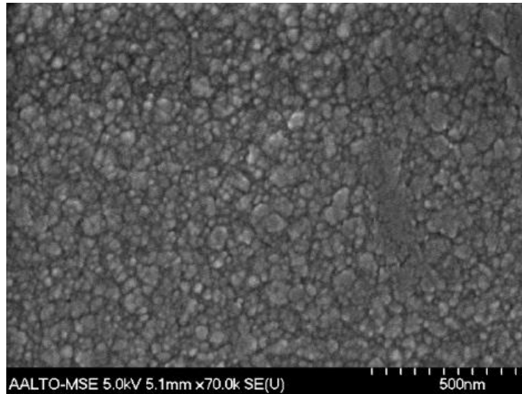
Figure 7. SEM micrograph at \times 70,000 magnification of gold electroplated copper surface produced by Häfner.
