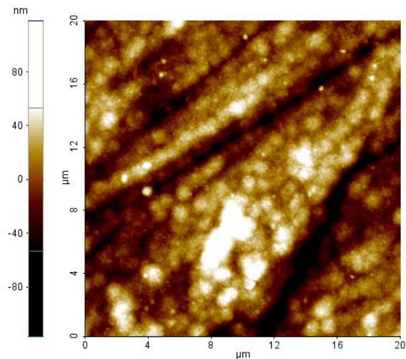
Figure 8. AFM topography image of gold-electroplated copper surface produced by Häfner, taken with a scan size of 20\text{ }\mu\text{m} \times 20\text{ }\mu\text{m} .
