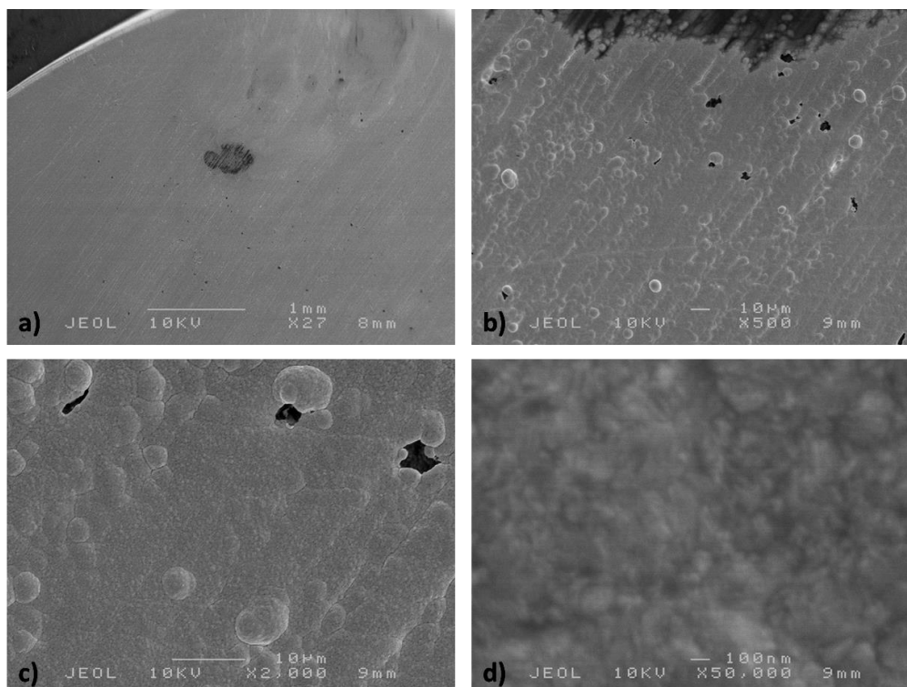
Figures 1a to 1d. SEM micrographs of NRC prepared samples demonstrating the lateral homogeneity and roughness of the gold plating formed from TSG-250 precursor solution on OFHC copper at NRC. The images a,b,c,d were each obtained at different magnifications ( \times 27 , \times 500 , \times 2,000 , \times 50,000 respectively) as indicated by the incorporated scale bars in the image.
