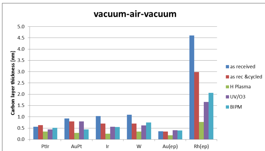
Figure 15. Carbon-layer thickness for different materials as received and after vacuum cycling and undergoing various cleaning processes.
