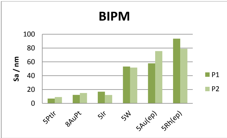
Figure 19. S_a surface roughness values for samples cleaned by nettoyage-lavage (measurements taken at 2 positions, P1 and P2, on the sample surface).
