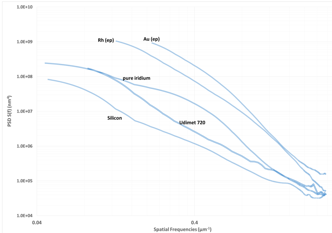
Figure 16. Laser scattering from different surfaces to measure roughness. Mean power spectral density curves for silicon, gold-electroplated copper Au(ep) and rhodium electroplated copper and Rh(ep). Comparison with iridium, silicon and Udimet 720. The PSD has dimensions of [L^4] as the scattering is two-dimensional. Specular reflection prevented measurements of the lowest spatial frequencies in some cases. See Zerrrouki et al. [1] for more details.
