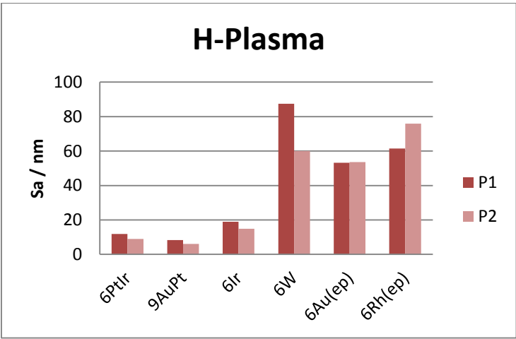
Figure 17. S_a surface roughness values for H-plasma cleaned samples (measurements taken at 2 positions, P1 and P2, on the sample surface).
