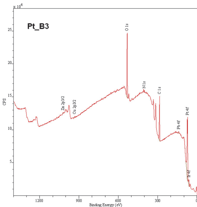
Figure 6. Survey scan of Pt-Ir sample Pt_B3 after contamination using the vacuum gauge method.
