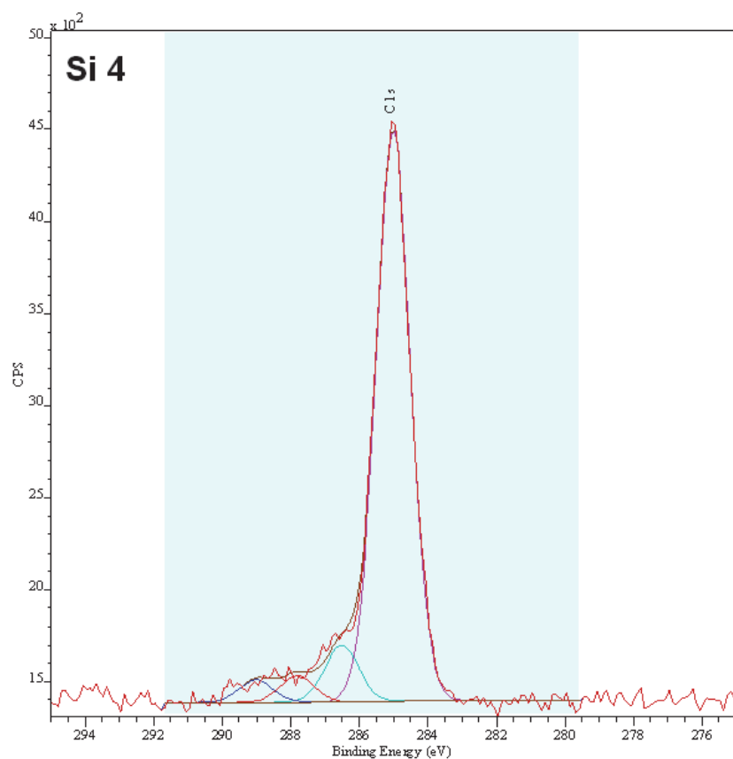
Figure 11. C1s narrow scan of silicon sample Si4.
