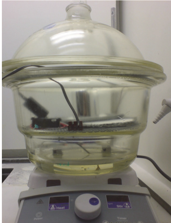
Figure 1. Apparatus used in the NPL heated oil method.
