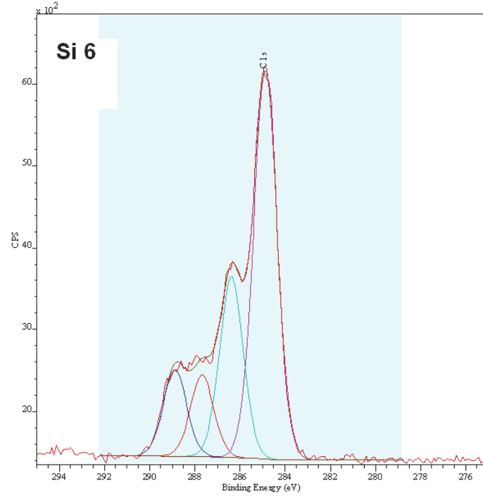
Figure 15. C 1s narrow scan of silicon sample Si6.
