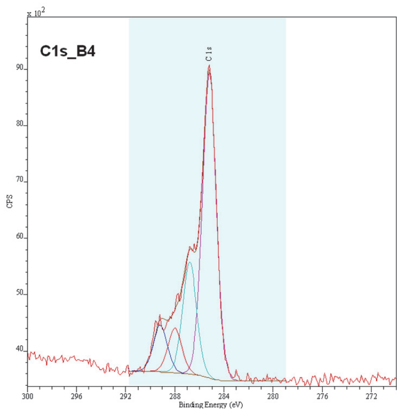
Figure 13. C 1s narrow scan of Pt-Ir sample Pt_B4.
