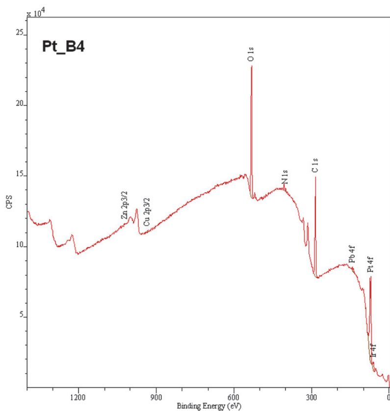
Figure 7. Survey scan of Pt-Ir sample Pt_B4 after contamination using the vacuum gauge method.
