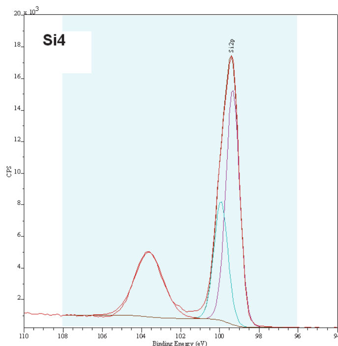
Figure 16. Si 2p narrow scan of silicon sample Si4.
