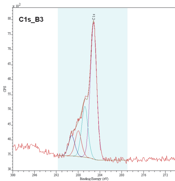
Figure 12. C1s narrow scan of Pt-Ir sample Pt_B3.
