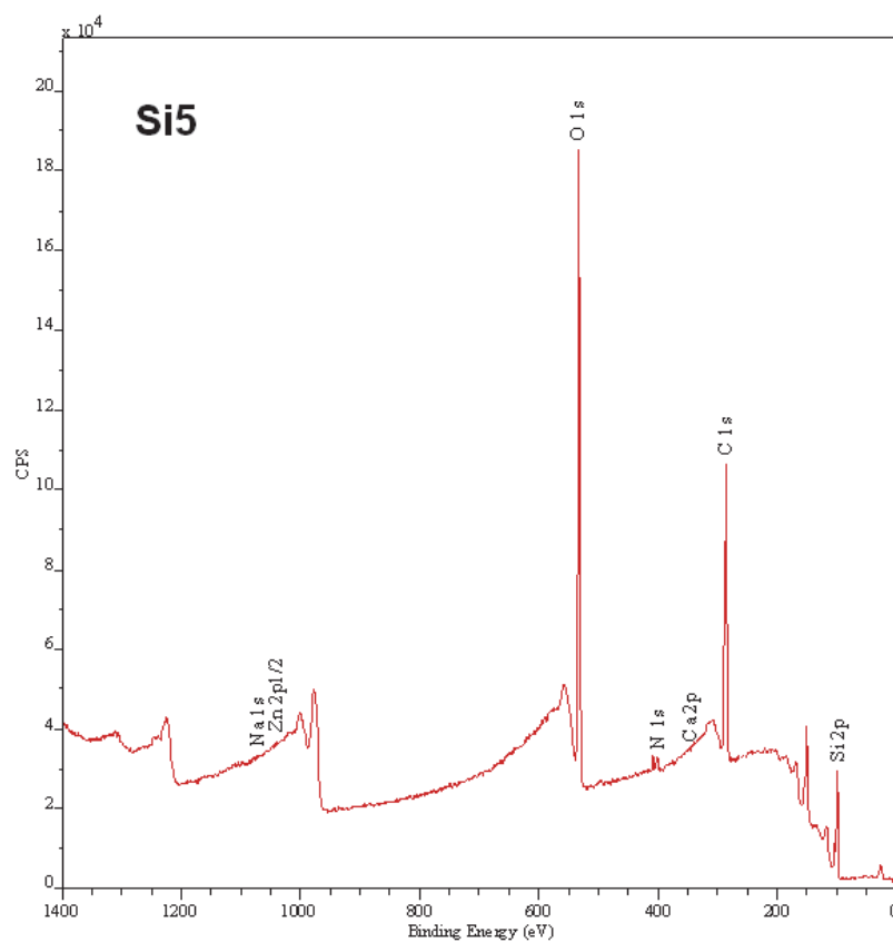
Figure 8. Survey scan of silicon sample Si5 after contamination using the vacuum gauge method.
