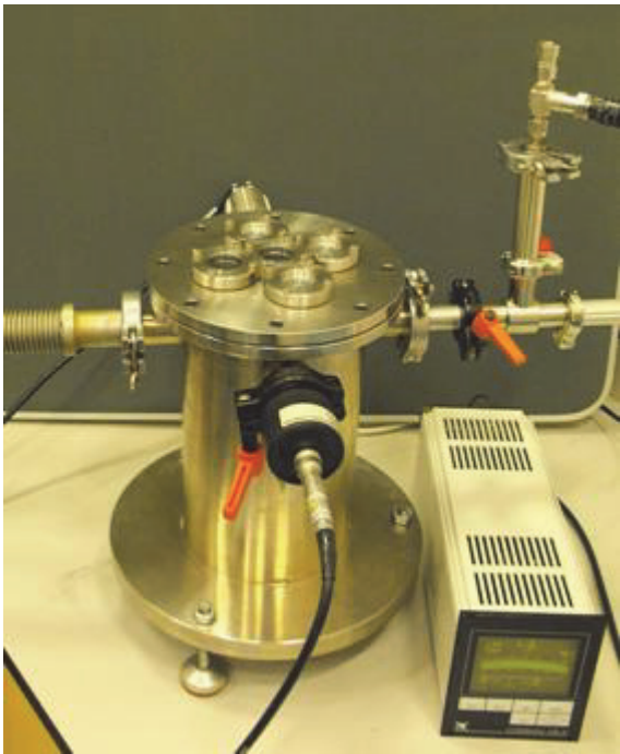
Figure 2. Apparatus used in the NPL vacuum contamination method.
