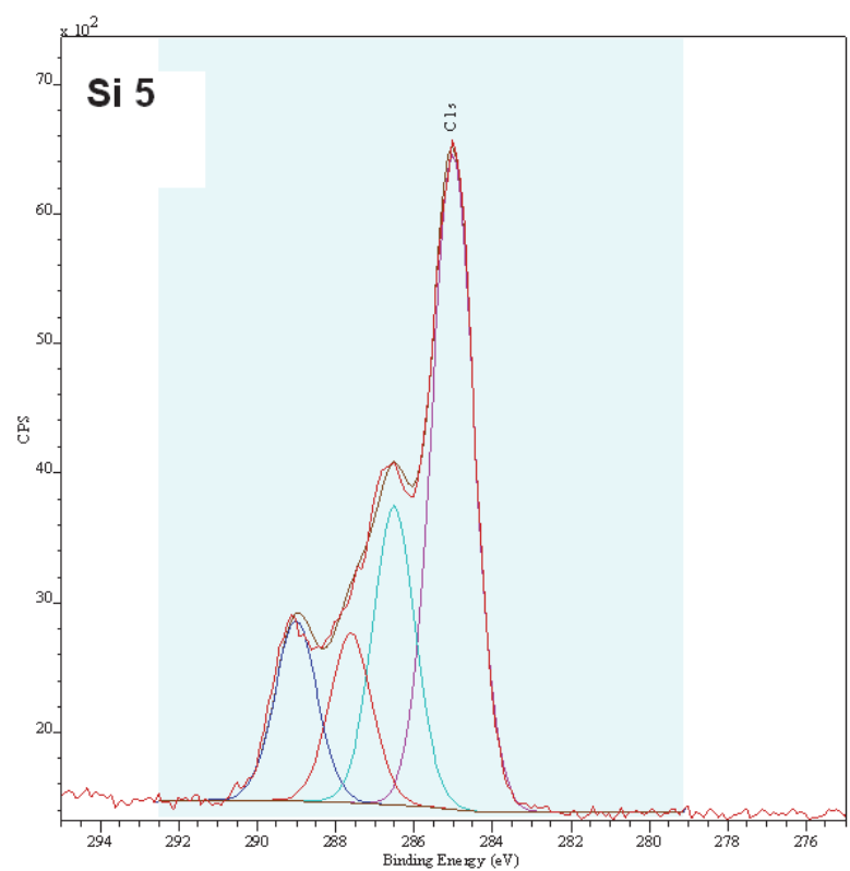
Figure 14. C 1s narrow scan of silicon sample Si5.
