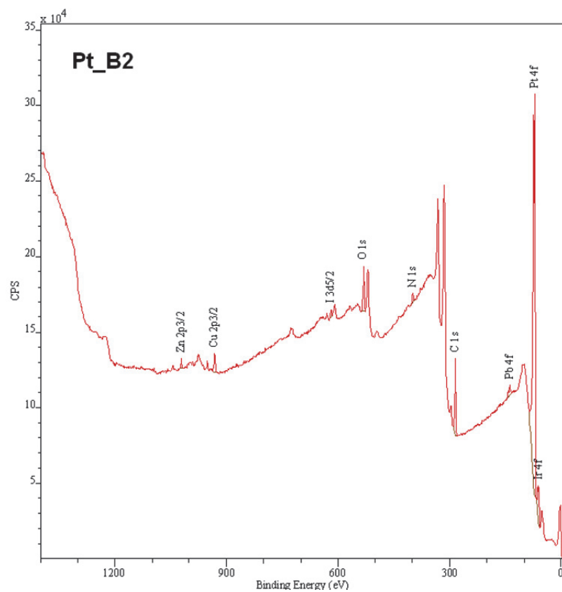
Figure 4. Survey scan of Pt-Ir sample Pt_B2.
