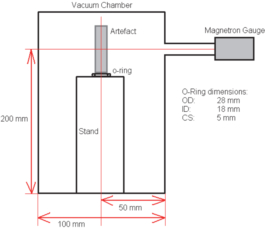
Figure 3. Schematic of the NPL vacuum contamination apparatus.
