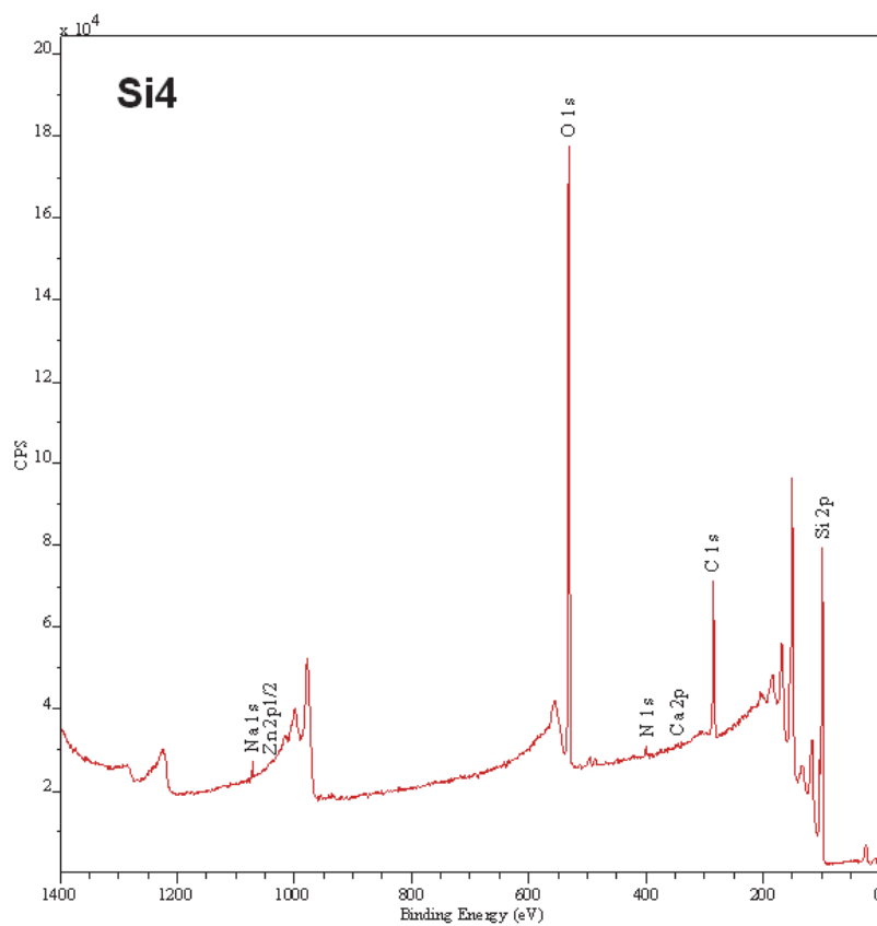
Figure 5. Survey scan of silicon sample Si4.
