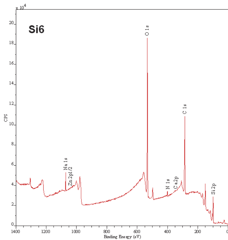
Figure 9. Survey scan of silicon sample Si6 after contamination using the vacuum gauge method.
