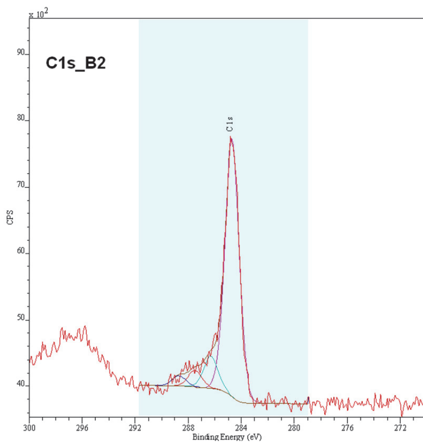
Figure 10. C 1s narrow scan of Pt-Ir sample Pt_B2.
