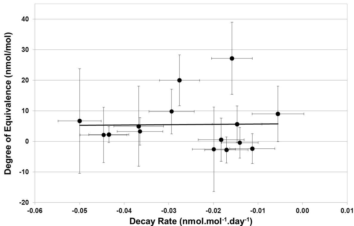
Figure 7 Degree of equivalence vs decay rate. Vertical error bars are the expanded uncertainties of the degree of equivalence. The horizontal ones are the standard errors of the decay rates.
