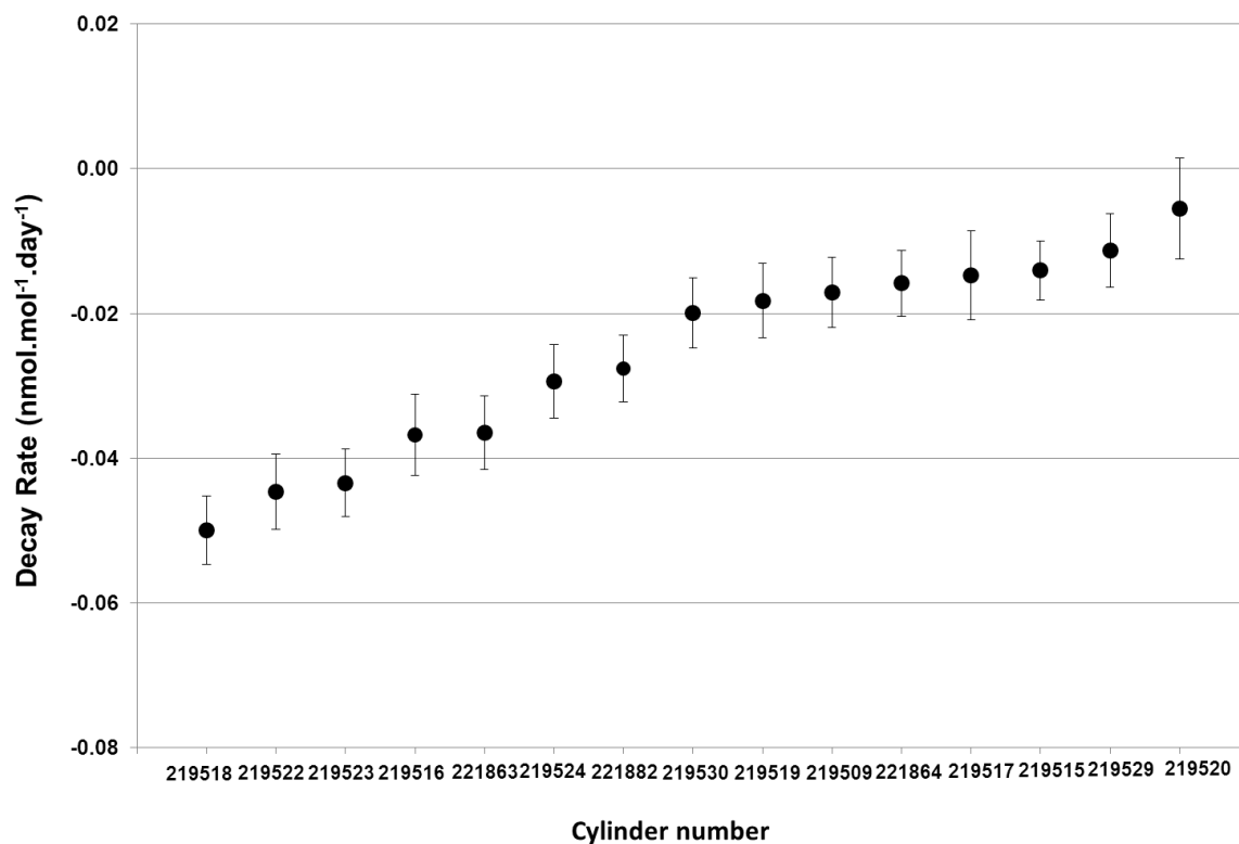
Figure 6 Estimated drifts of the travelling standards listed in Table 2 displayed in ascending order. The error bars indicate the standard errors of the gradients of the respective straight lines.
