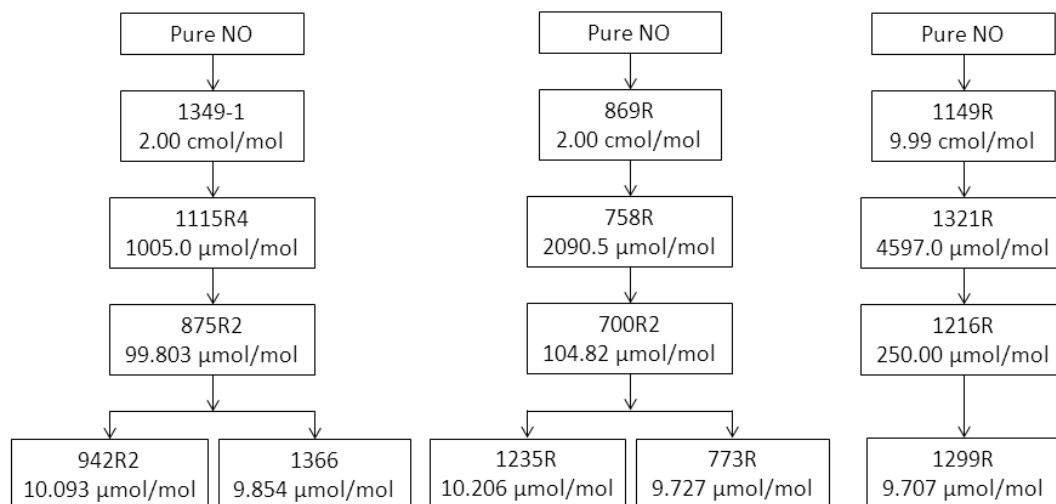
Figure 1 The hierarchy of the gravimetric standards of NO/N 2 prepared gravimetrically by the coordinating laboratory.
