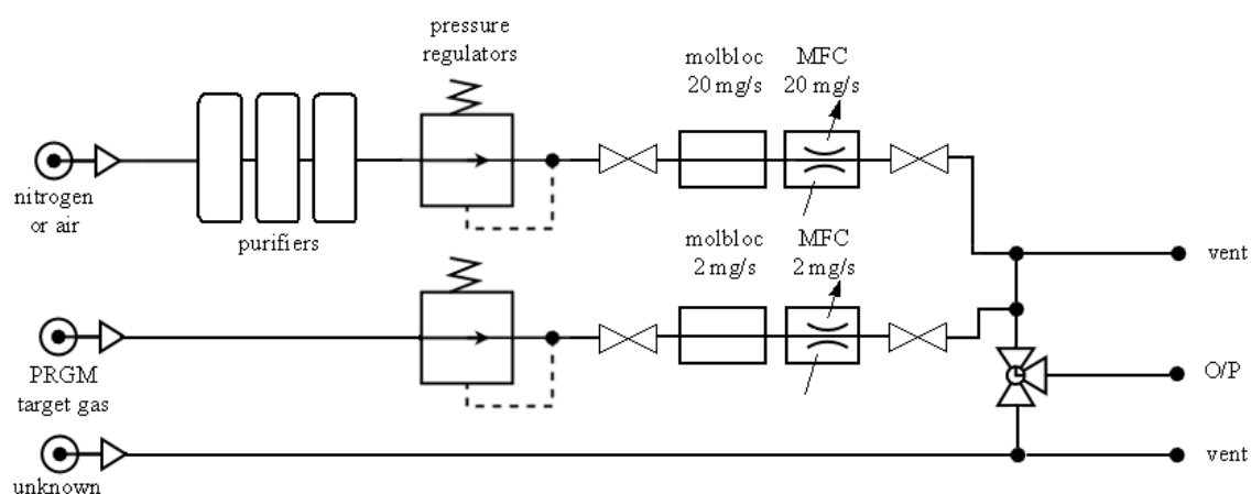
Figure 3 Schematic of the high accuracy dilution system. The output (O/P) is connected to a gas analyser. A two-way valve is used to alternate the flow of the blend and unknown to the analyser.
