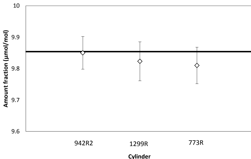
Figure 2 Validation of NPL 1366 against three PRGMs. The solid black line represents the gravimetric amount fraction of NPL 1366. The bars represent 2 standard deviations of each measurement set.
