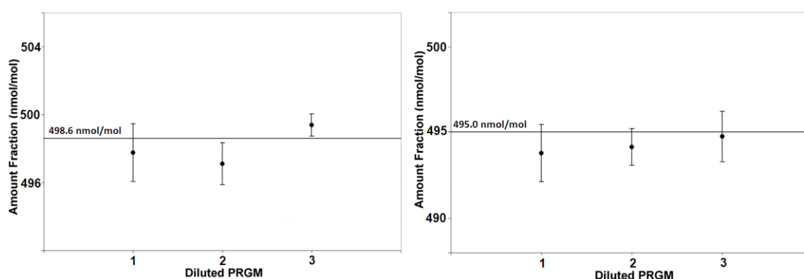
Figure 4 Validation of the dynamic dilution facility by means of the certification of two different 500 nmol/mol standards with three different PRGMs.
