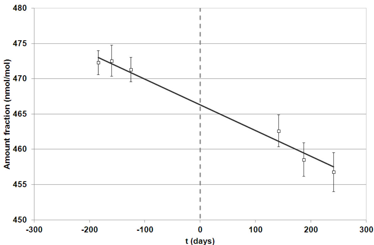
Figure 5 Example of the estimation of the drift in the amount fraction experienced in one of the travelling standards. The regression line has been fitted by ordinary least squares. The x -axis represents the time difference between measurements, taking as the reference the date when the participant carried out its measurements ( t_j=0 ). The error bars indicate the standard uncertainty.
