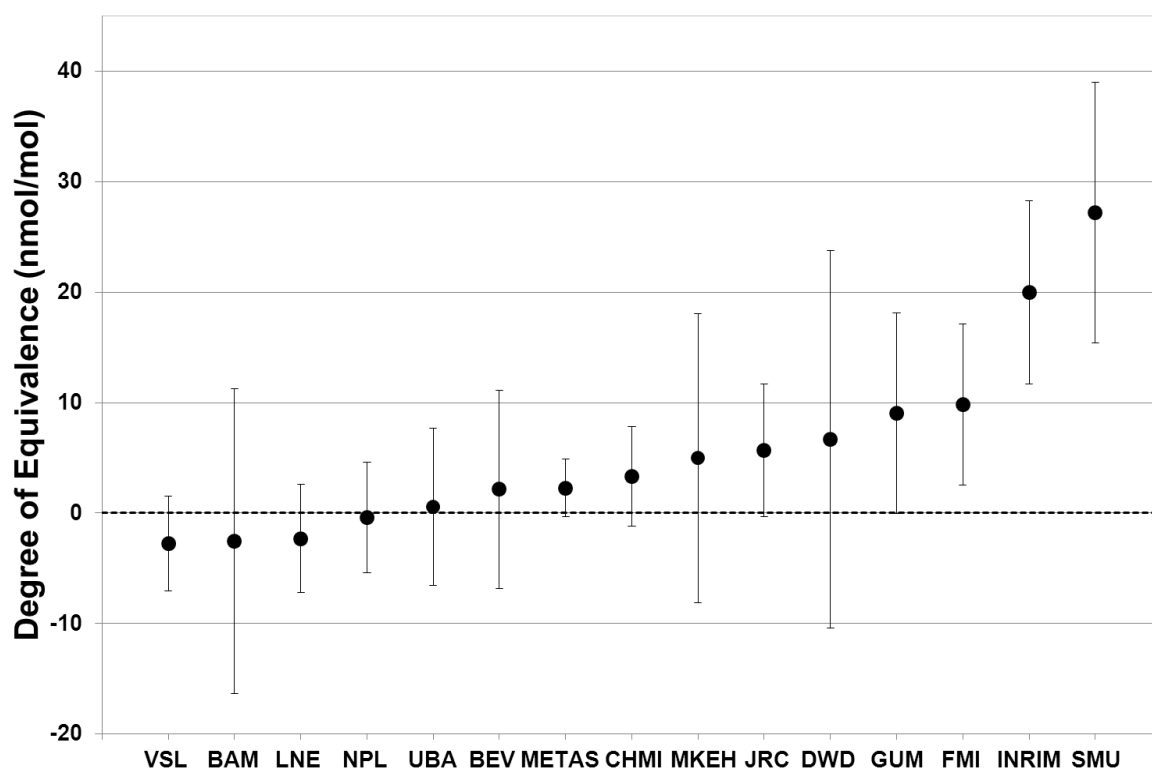
Figure 8 Degrees of equivalence of the participating laboratories. The error bars are the expanded uncertainties of the degrees of equivalence obtained from the uncertainty of the results reported by each participant and the uncertainty in the KCRV.
