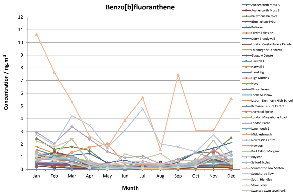
Figure 12(b): Monthly mean benzo[b]fluoranthene concentrations recorded at 'A' and 'B' stations during 2012.
