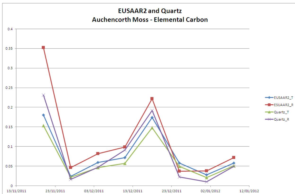
Figure 4-15 Comparison between Quartz and EUSAAR 2 for OC and EC at Auchencorth Moss
