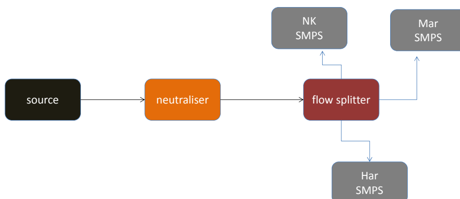
Figure 4-30 Schematic showing the parallel sampling of the three SMPS when connected to a flow splitter and fed with a single particle source (CAST-soot), conditioned with a single neutraliser.
