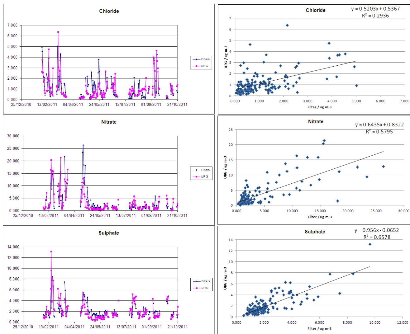
Figure 4-20 Comparison between daily filter based measurements of chloride, nitrate and sulphate and daily average concentration from the URG analyser at North Kensington.
