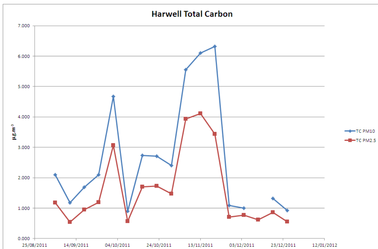
Figure 4-12 Comparison between PM 2.5 weekly TC and PM 10 averaged weekly TC measurements at Harwell.
