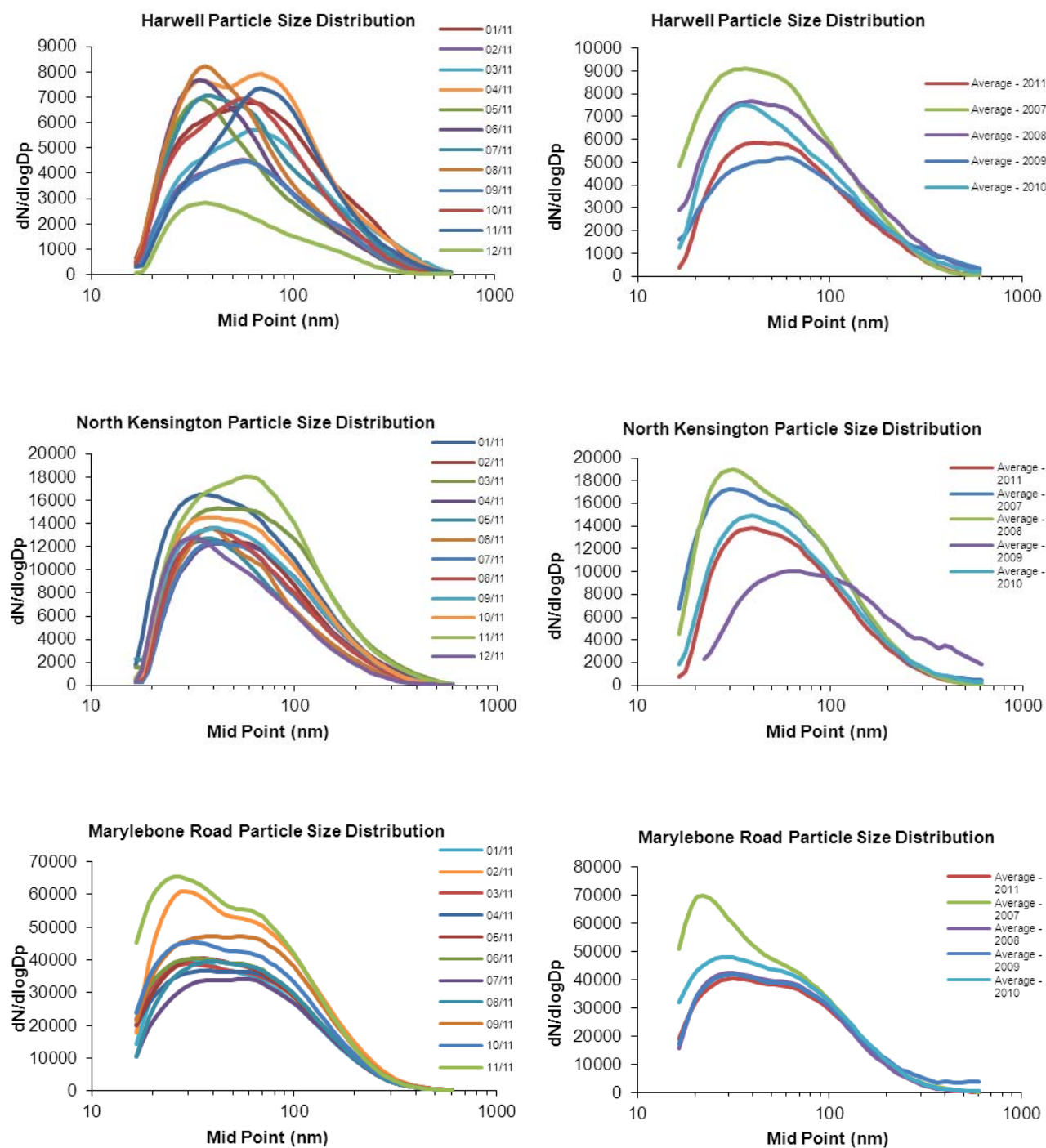
Figure 4-25 Monthly averaged particle size distributions at the Network sites during 2011 [left-hand panels] and comparison of the 2007, 2008, 2009, 2010 and 2011 annual-averaged size distributions [right-hand panels].
