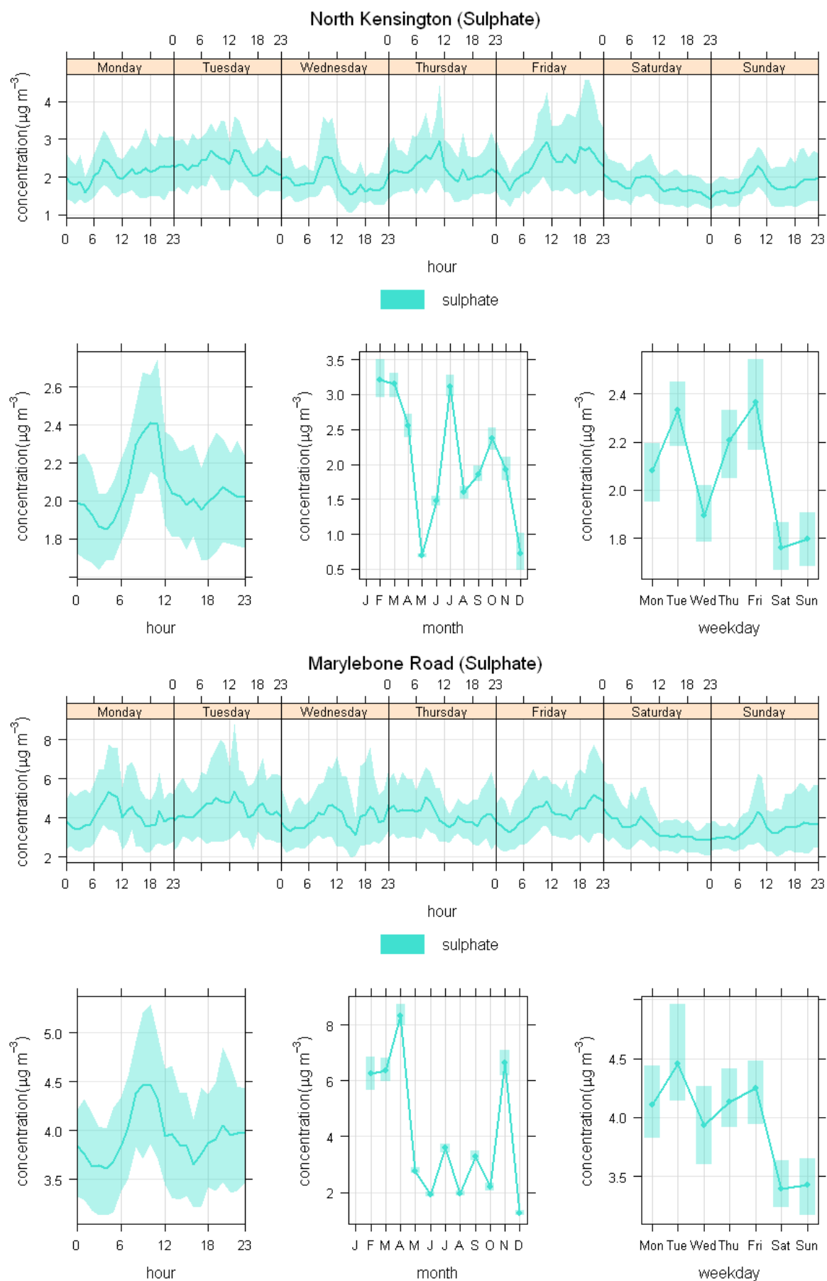
Figure 4-53 Sulphate profiles at the London sites in 2011
