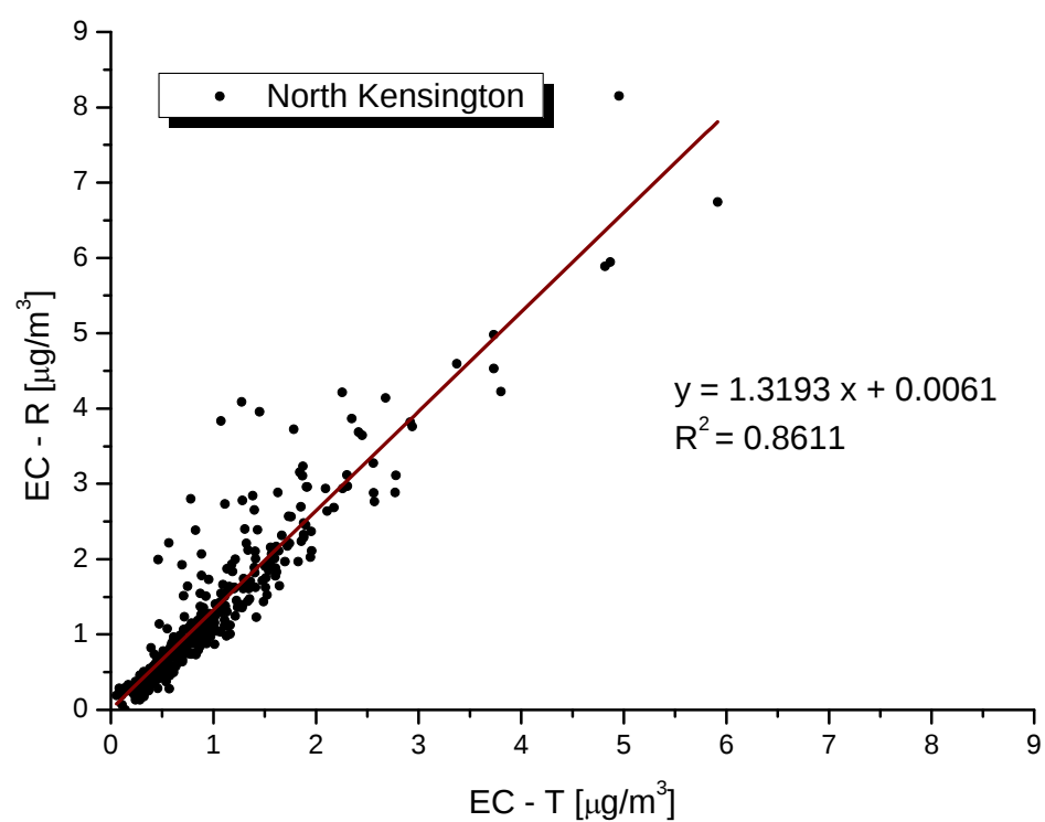
Figure 4-6 Scatter plots of OC and EC measurements for TOT and TOR methods at North Kensington
