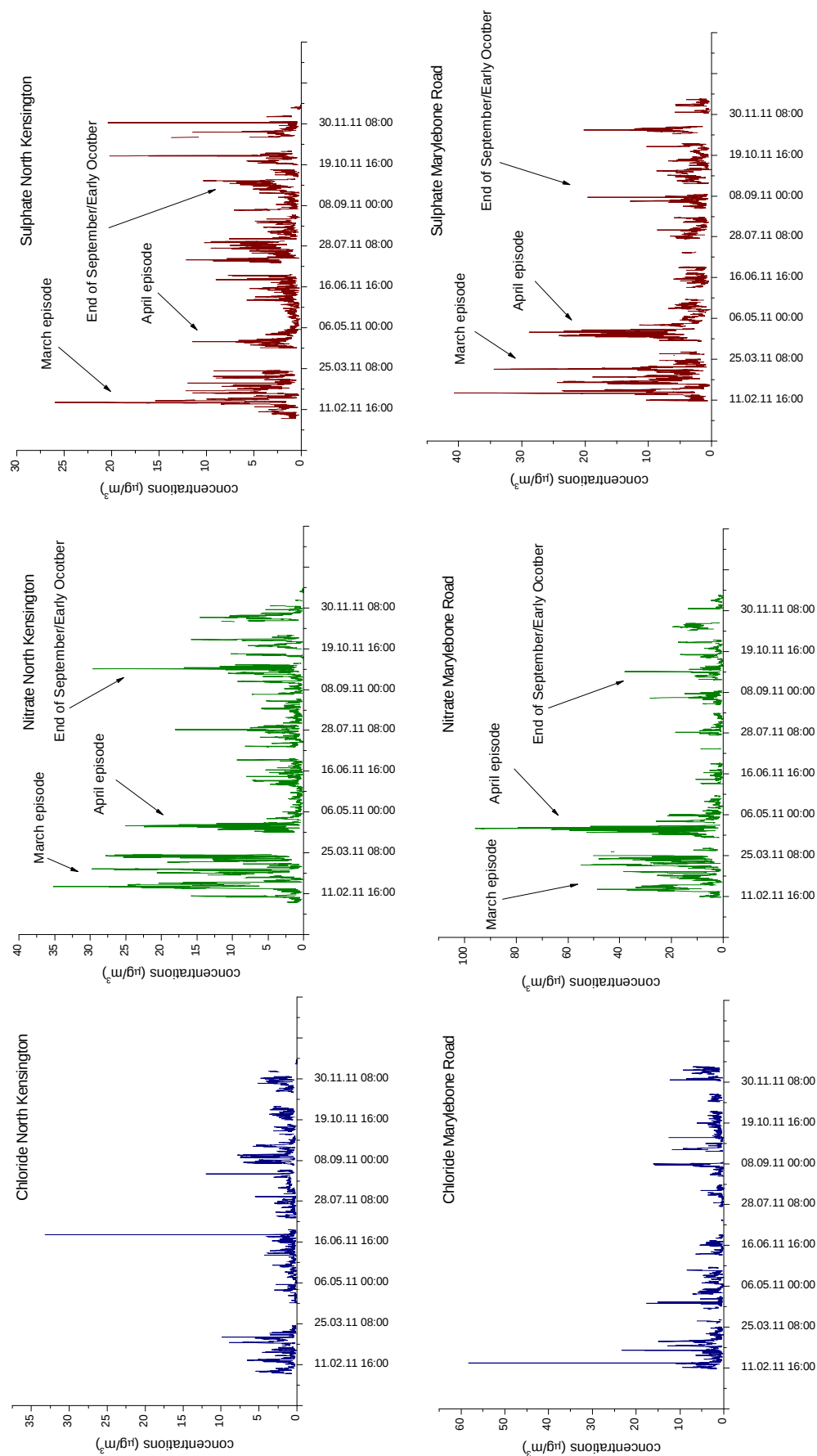
Figure 4-17 Anion concentration at the London sites in 2011
