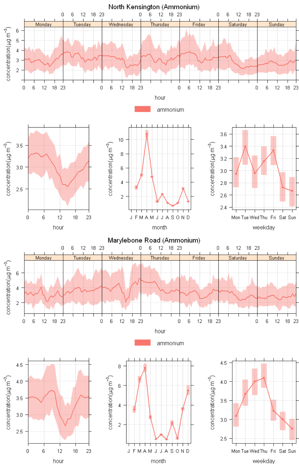
Figure 4-48 Ammonium profiles at the London sites in 2011
