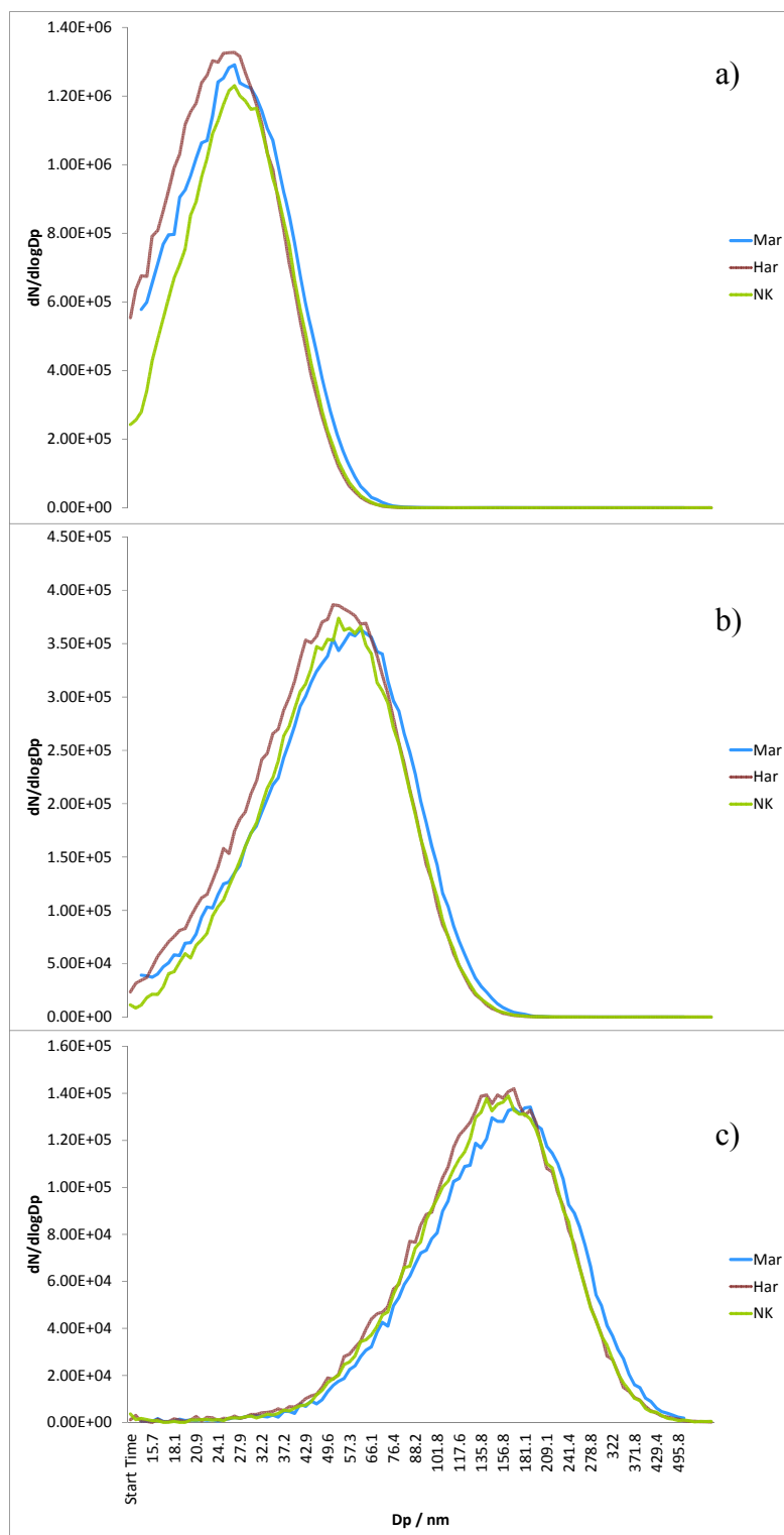
Figure 4-32 SMPS scans of the three site instruments when fed with CAST generated particles at nominal diameters of a) 26 nm, b) 55 nm and c) 156 nm.
