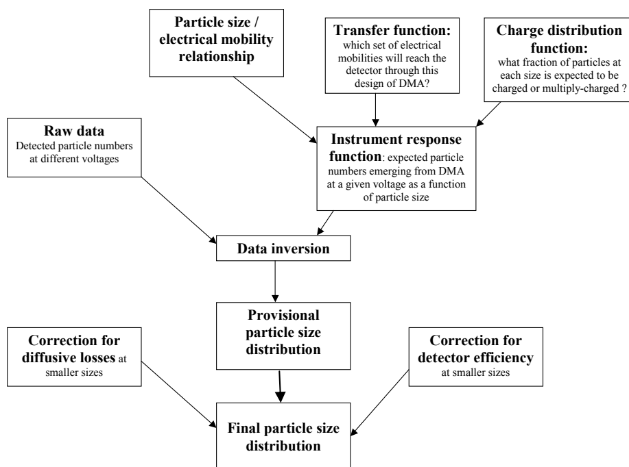
Figure 4-23 Schematic of the internal data processing of SMPS instrument in the Network
