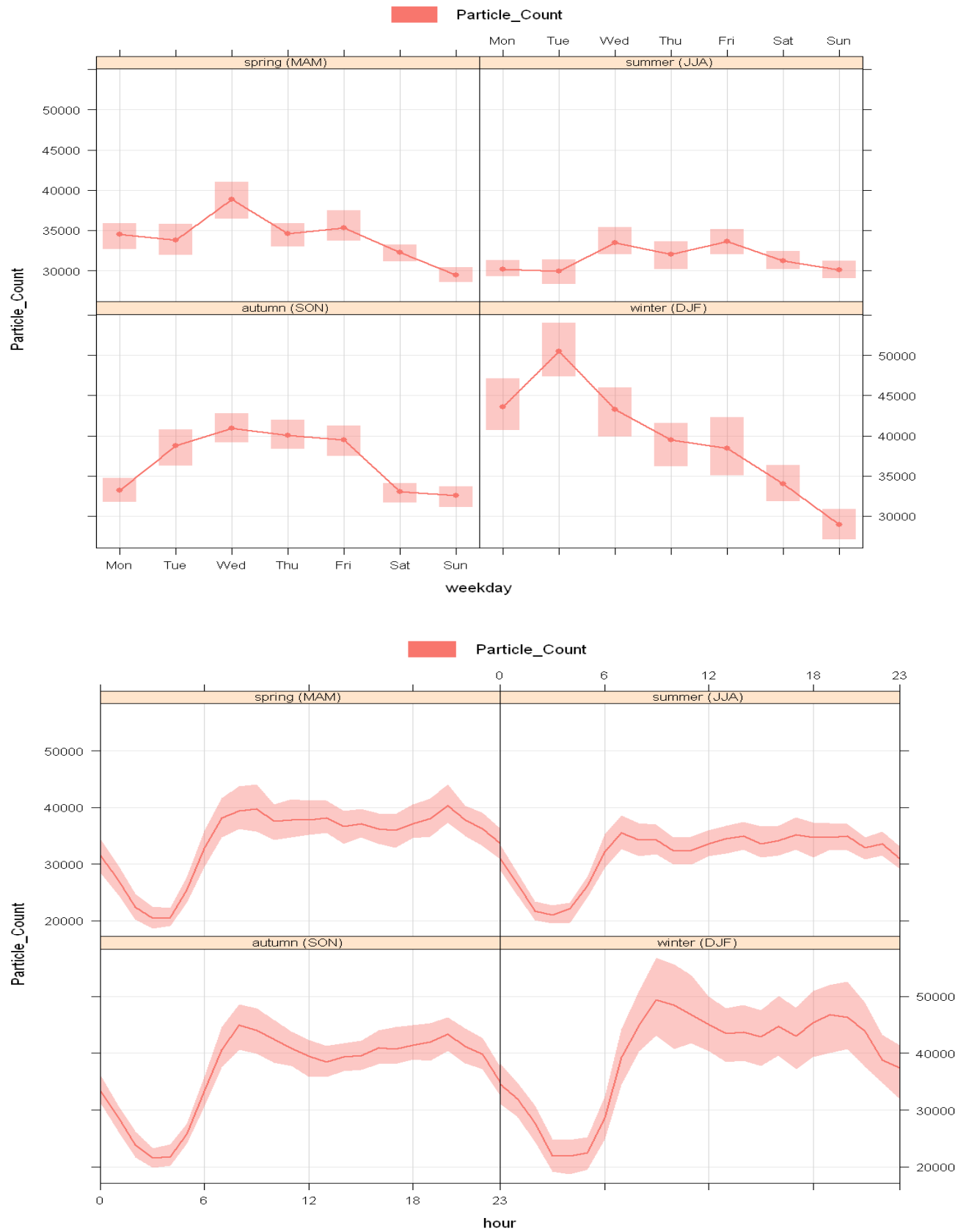
Figure 4-44 Seasonal weekly and diurnal trends for Marylebone Road CPC measurements
