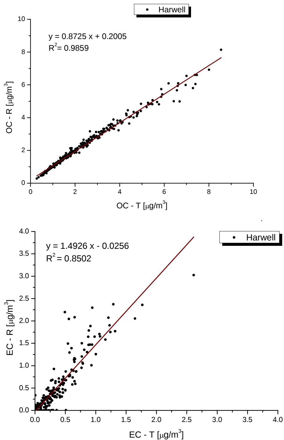
Figure 4-5 Scatter plots of OC and EC measurements for TOT and TOR methods at Harwell
