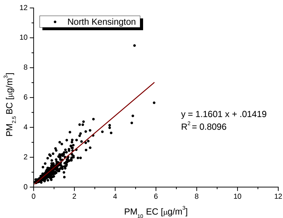
Figure 4-9 Comparison between \text{PM}_{2.5} \text{ BC} and \text{PM}_{10} \text{ EC} (T) at North Kensington in 2011
