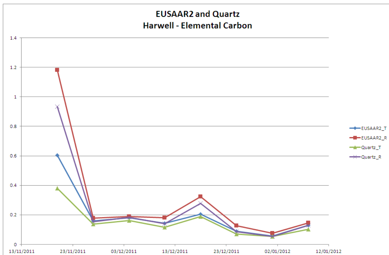
Figure 4-13 Comparison between Quartz and EUSAAR 2 protocols at Harwell for OC and EC
