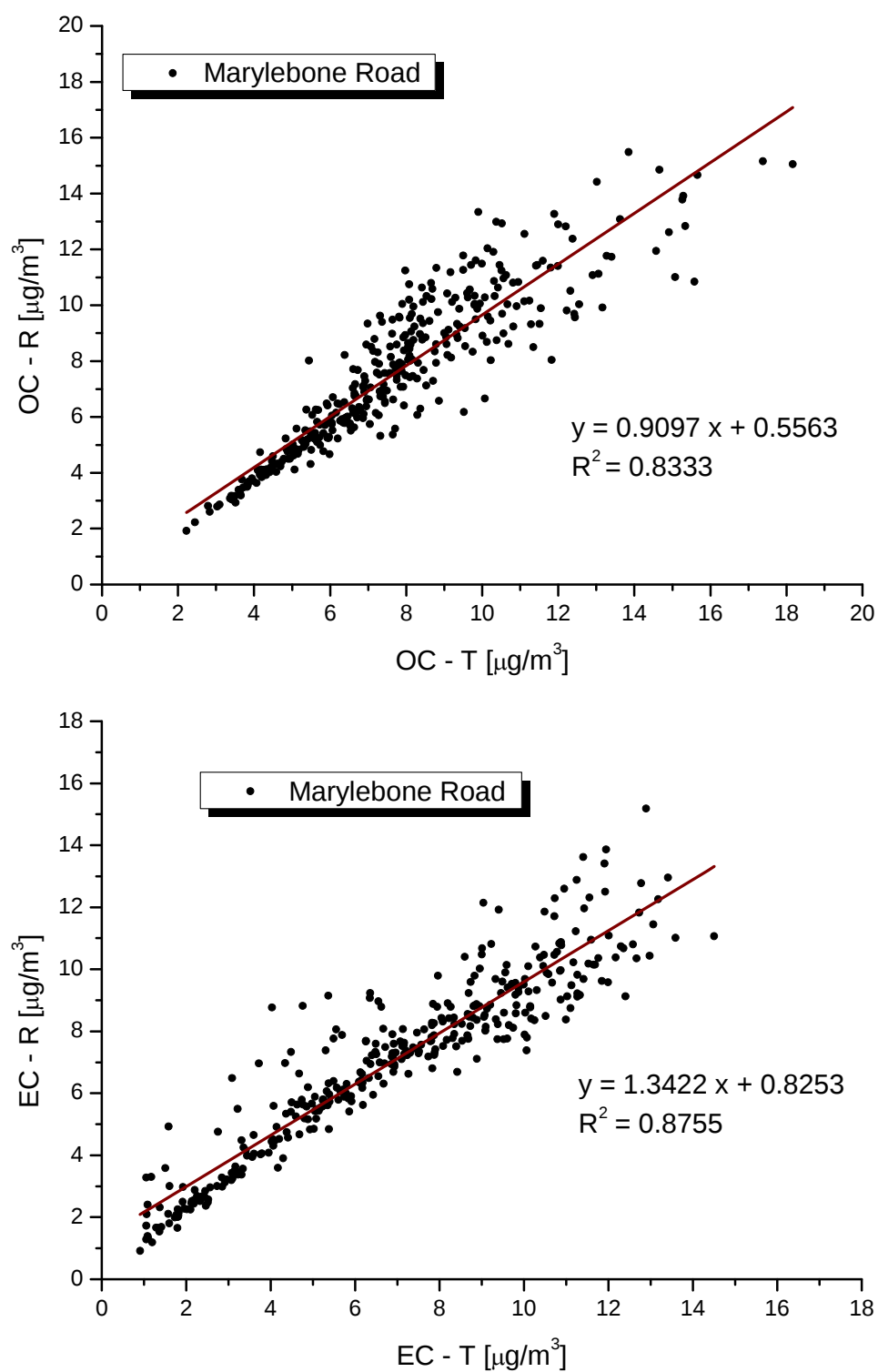
Figure 4-7 Scatter plots of OC and EC measurements for TOT and TOR methods at Marylebone Road
