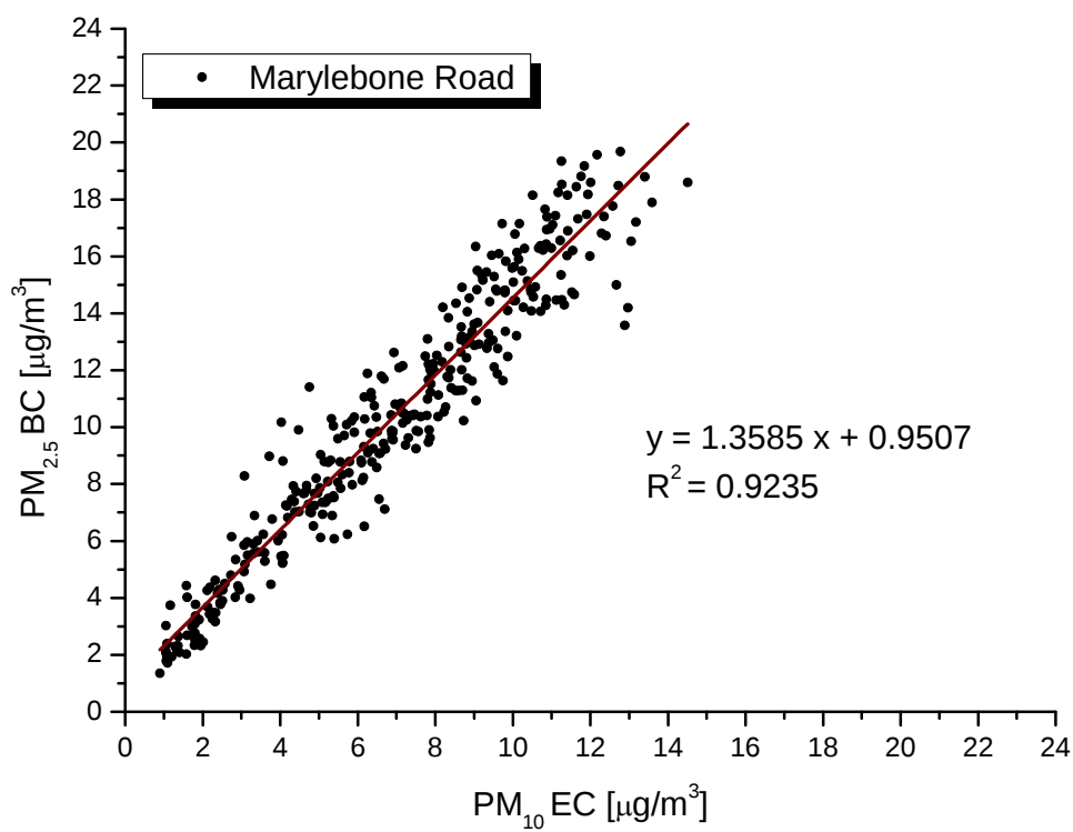
Figure 4-10 Comparison between \text{PM}_{2.5} \text{ BC} and \text{PM}_{10} \text{ EC} (T) at Marylebone Road in 2011
