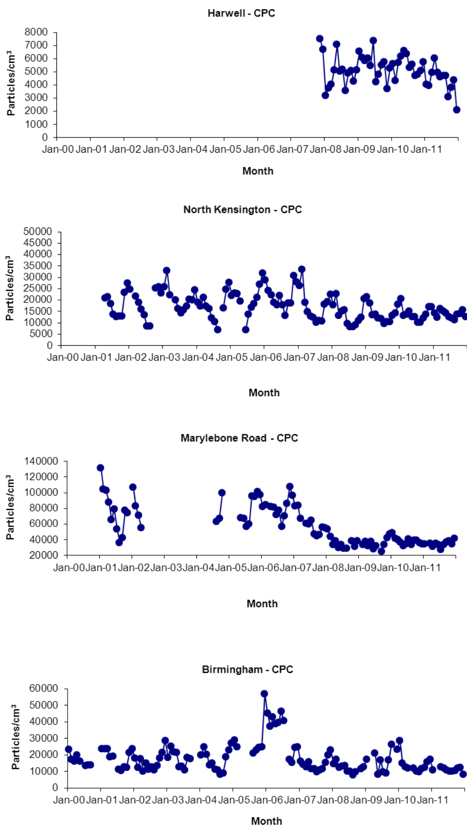
Figure 4-35 Monthly trends for CPC counts at the Network sites
