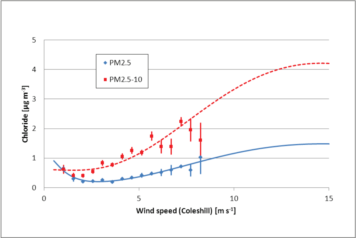
Figure 6-4: Midland sites - fine and coarse chloride
