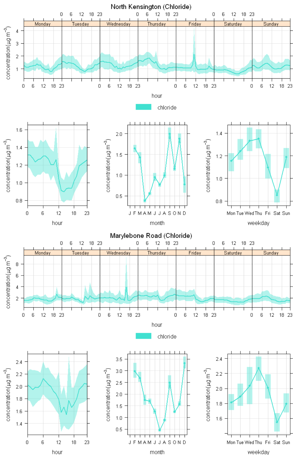
Figure 4-52 Chloride profiles at the London sites in 2011
