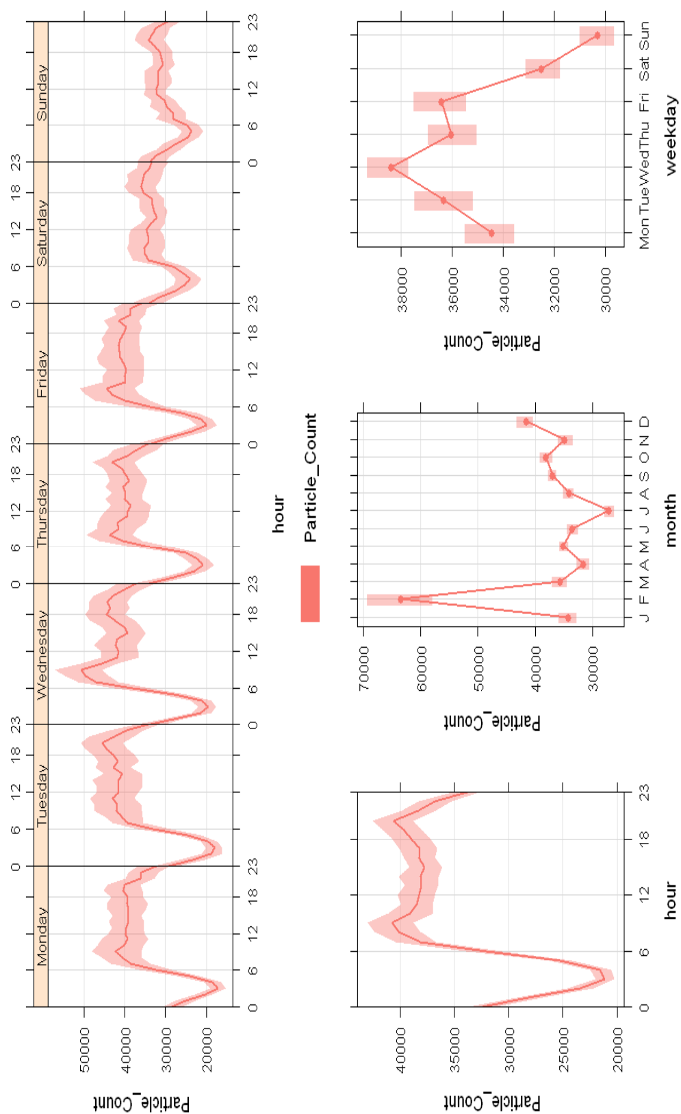
Figure 4-43 Diurnal and weekly trends for Marylebone Road CPC measurements
