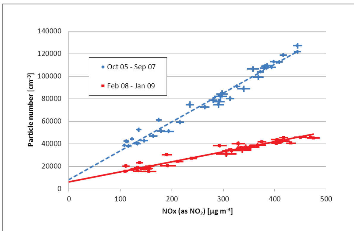
Figure 6-2 Particle number v NOx at Marylebone Road (Data sorted by 10° wind direction)
