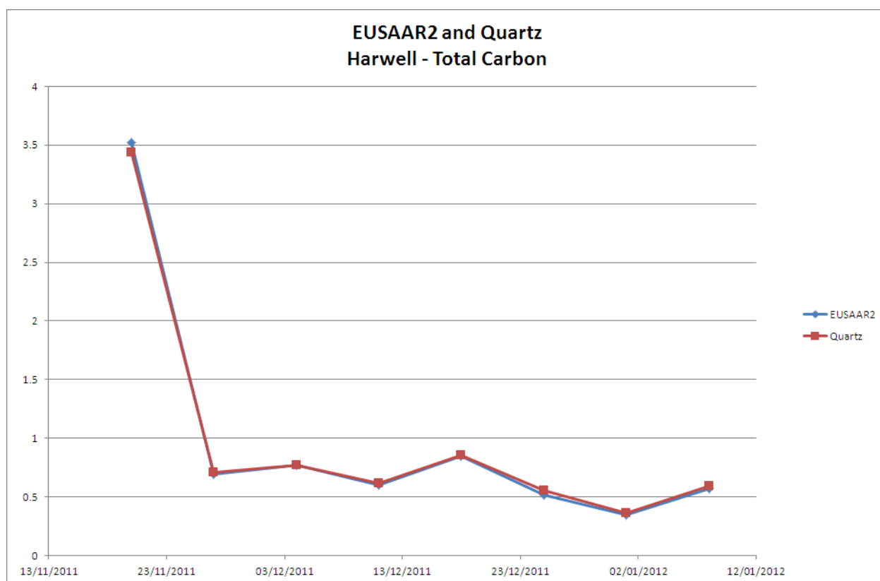
Figure 4-14 Comparison between Quartz and EUSAAR 2 protocols for TC at Harwell
