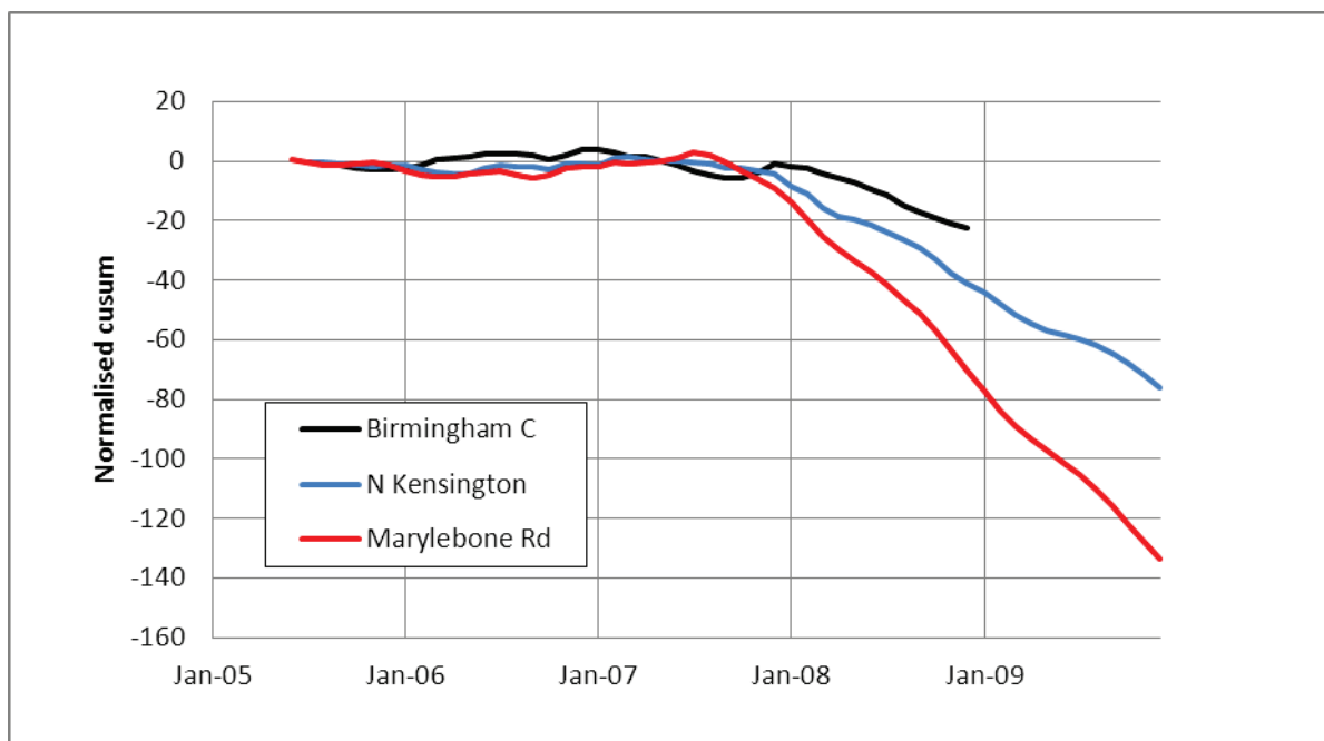
Figure 6-1 Normalised monthly cumulative sums of particle number concentration difference
