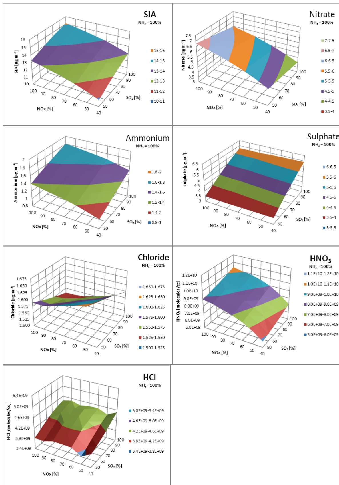
Figure 6-5: Effect of emission reductions in UK and Europe, NH 3 = 100%
