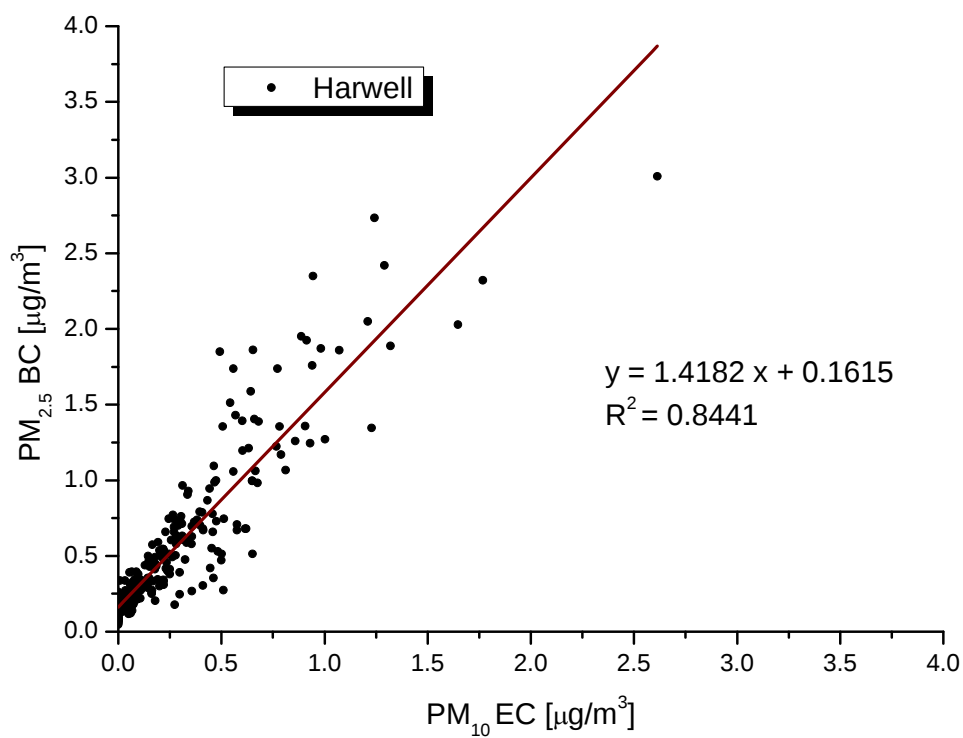
Figure 4-8 Comparison between \text{PM}_{2.5} \text{ BC} and \text{PM}_{10} \text{ EC} (T) at Harwell in 2011
