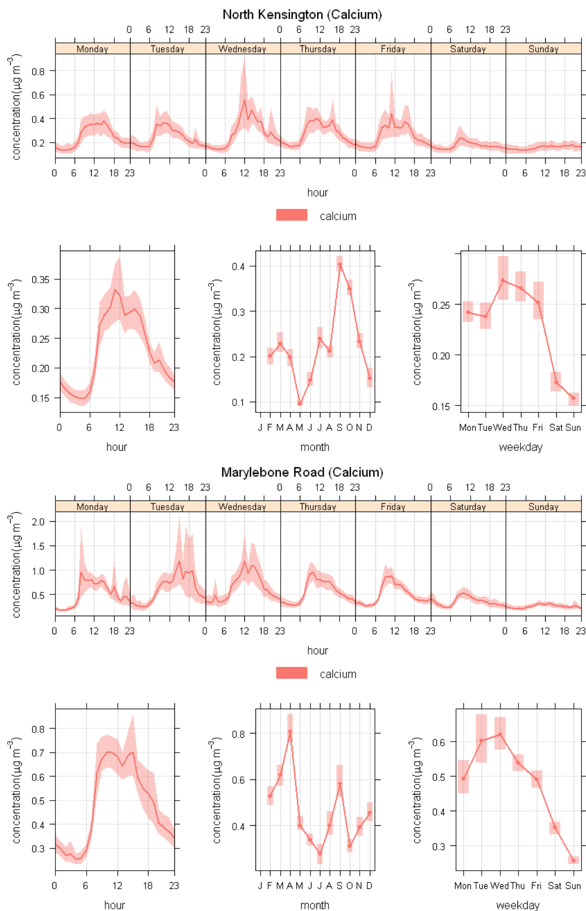
Figure 4-51 Calcium profiles at the London sites in 2011
