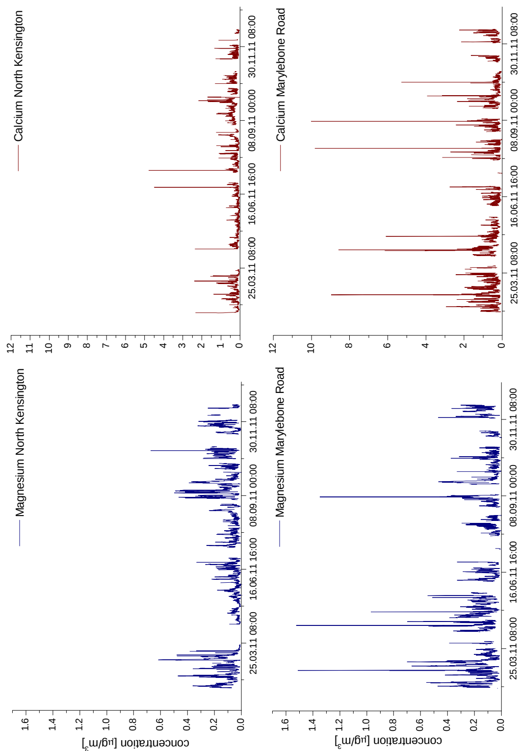
Figure 4-19 Magnesium and calcium concentrations at the two London sites in 2011
