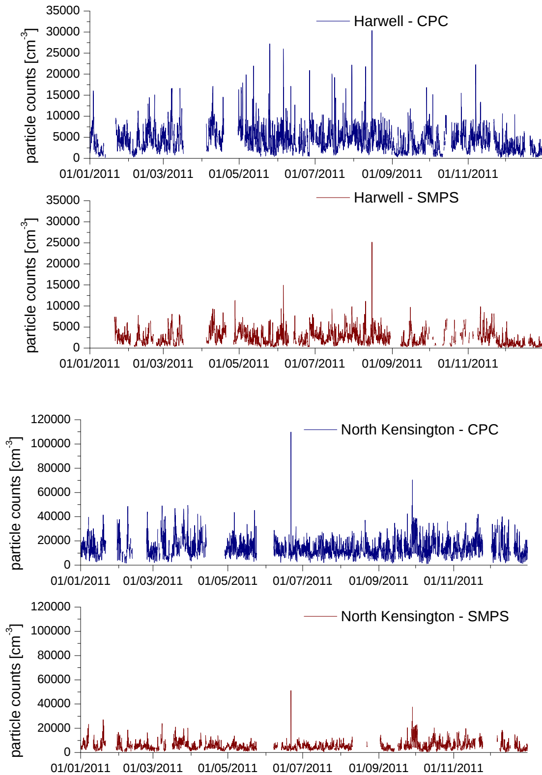
Figure 4-26 CPC and SMPS time series at Harwell and North Kensington sites in 2011
