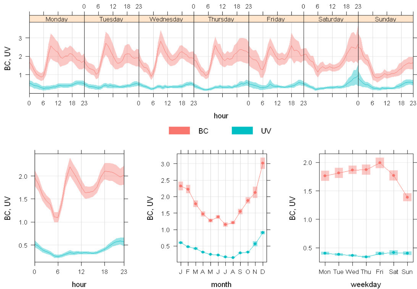
Figure 17 Urban Background Sites
