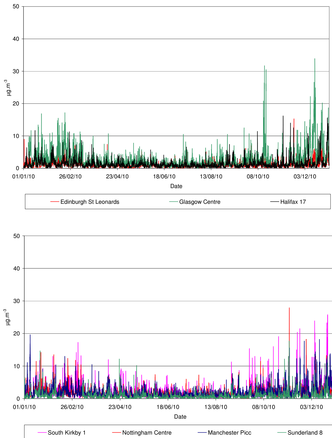
Figure 5 + 6 Black Carbon concentrations during 2010 in Scotland and Northern England
