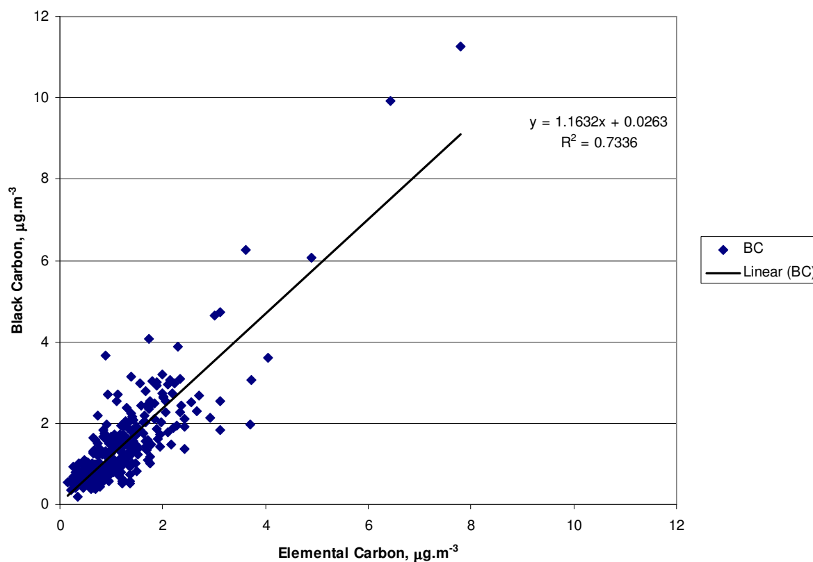
Figure 21 2010 EC and BC Measurements at North Kensington
