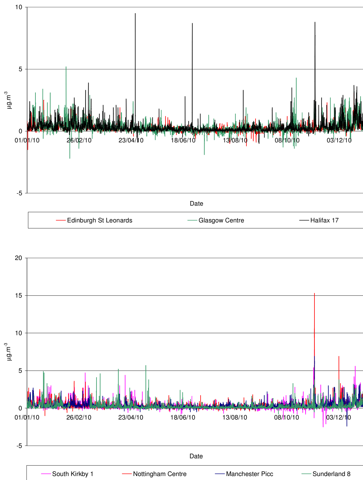
Figure 10+11 UV component concentrations during 2010 in Scotland and Northern England
