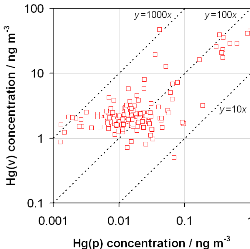
Figure 9. The relationship between monthly particulate [ \text{Hg(p)} ] and total gaseous [ \text{Hg(v)} ] mercury measurements during 2009 where these are made together. The dotted diagonal lines represent the locus of points for which the total gaseous mercury concentration ( y ) are 10, 100 and 1000 times greater than the measured particulate phase mercury concentrations ( x ), as indicated.
