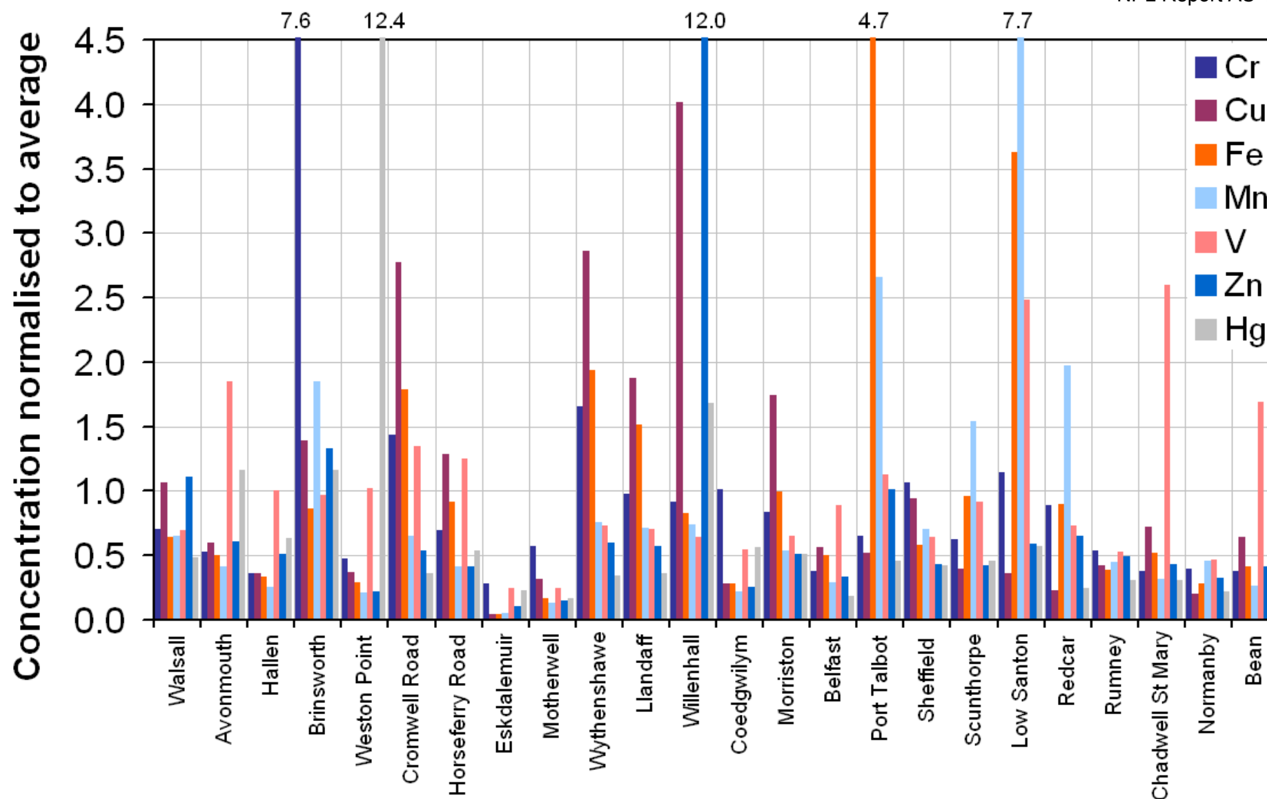
Figure 8. A summary of the annual mean measured concentrations of the non-directional metals at all sites on the UK Heavy Metals Monitoring Network in 2009, normalised to the UK annual average concentration for the relevant element. Bars that are off-scale have their values indicated at the top of the chart. Hg refers to particulate phase mercury.
