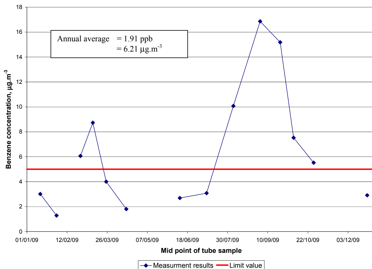
Figure 9 Time series of benzene concentrations measured by the Derby Spondon pump box
