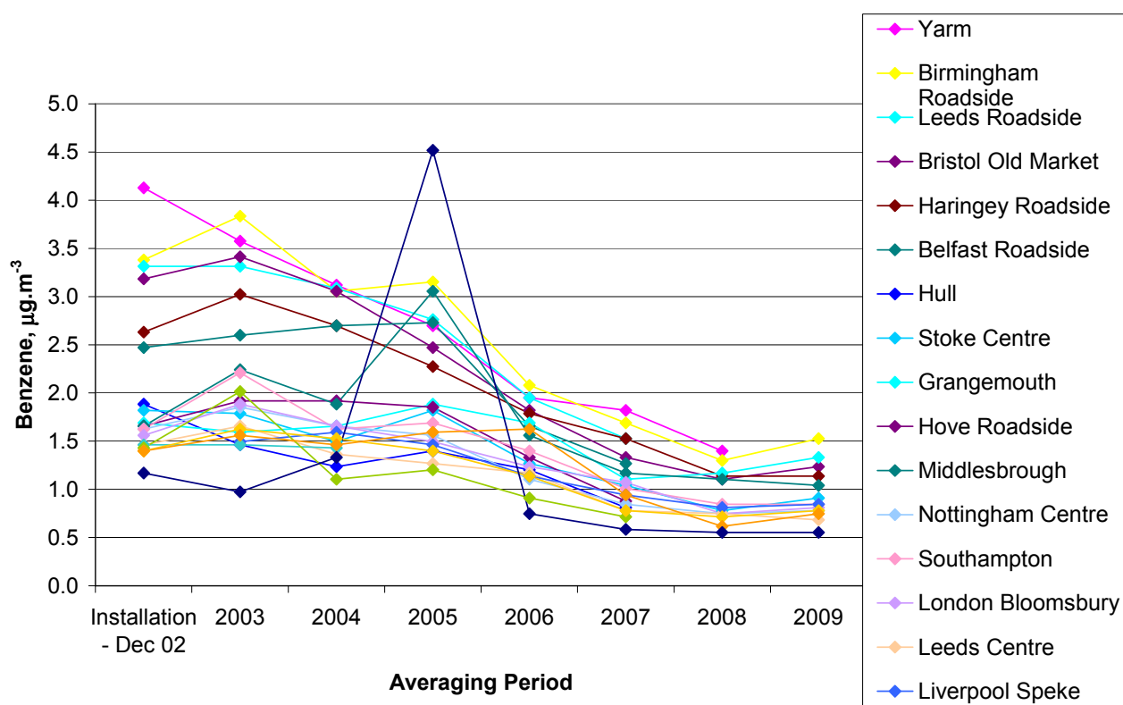
Figure 2 : Recent annual average benzene concentrations at "high concentration" sites
