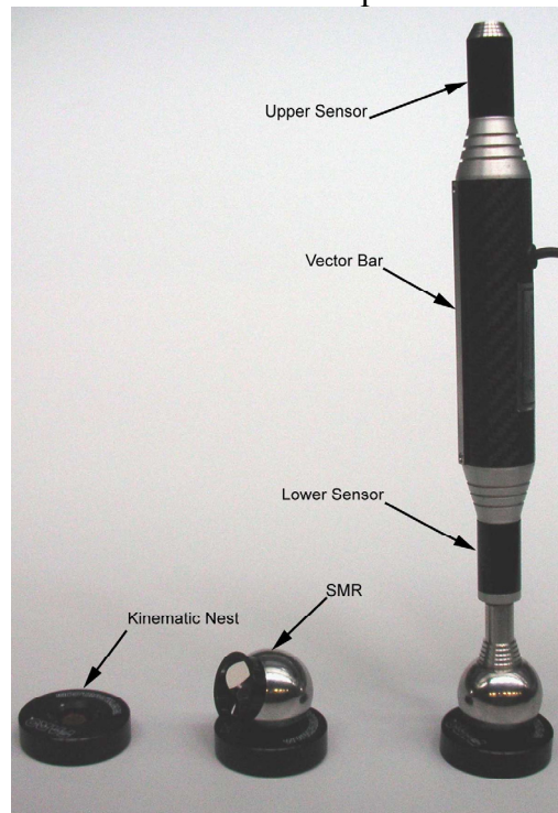
Figure 2, iGPS Vector Bar comprising two receivers in-line with a probe ball.
