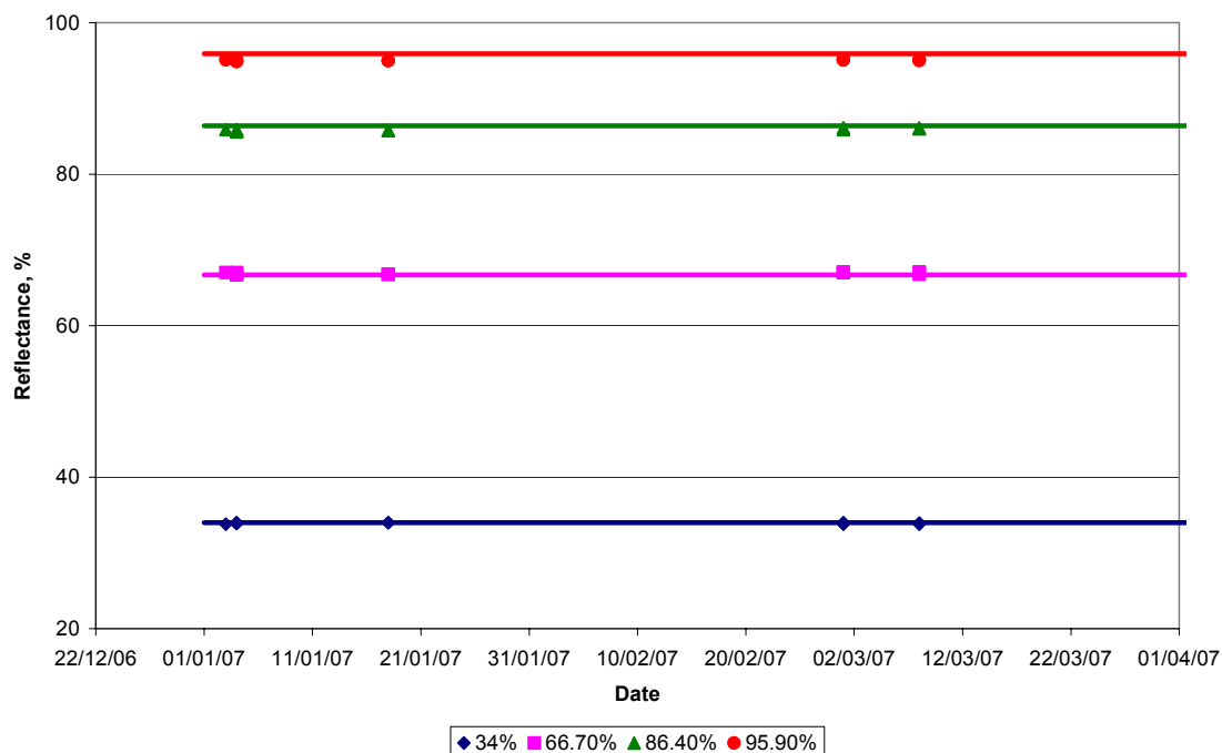
Chart 2 Calibration history of NPL Reflectometer
