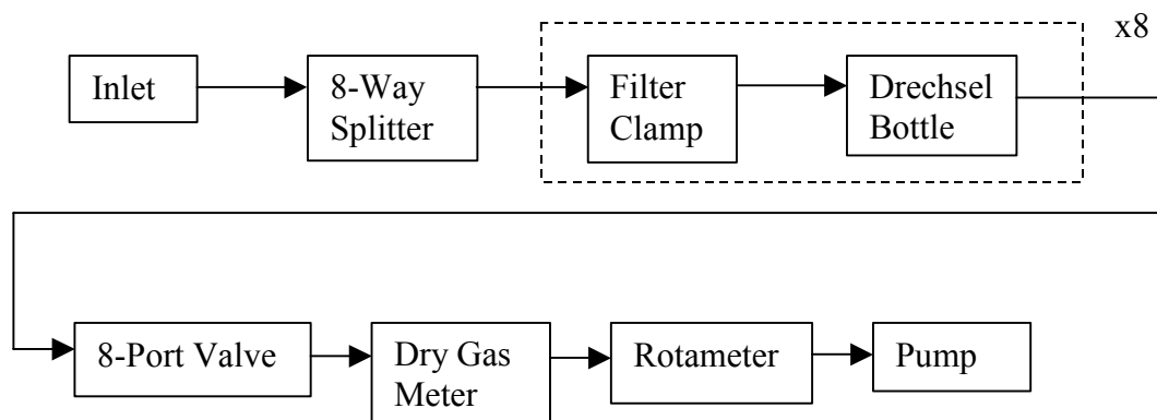
Figure 1 Schematic Outline of a Black Smoke Sampler
