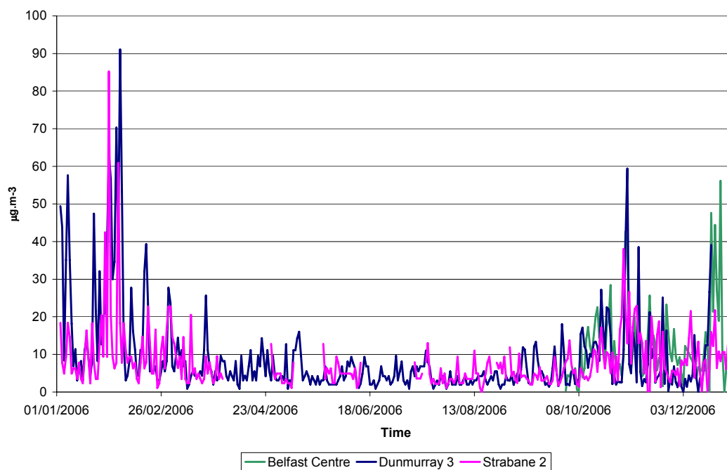
Chart 3 Black Smoke concentrations during 2006 in Northern Ireland
