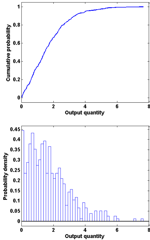
Figure 7.1: An approximation (top) obtained using a Monte Carlo method, with 500 trials, to the distribution function for the output quantity Y , where Y = X^2 and X has expectation 1.2 and standard deviation 0.5 and is assigned a Gaussian distribution. A histogram (below) of the values used to produce the (approximate) distribution function. It constitutes a discrete, scaled approximation to the PDF for Y .
