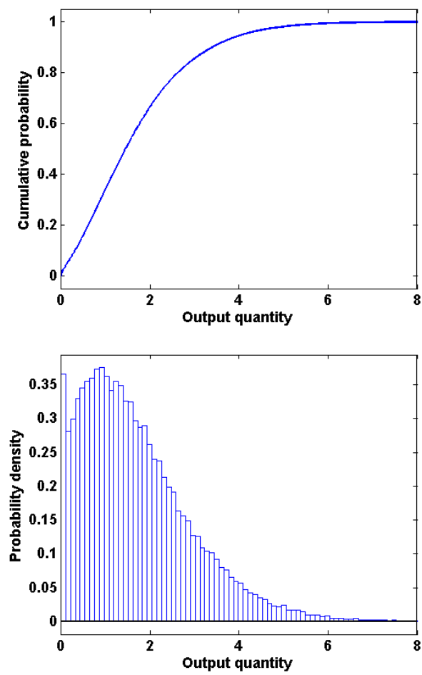
Figure 7.2: As Figure 7.1 but based on 50 000 Monte Carlo trials.
