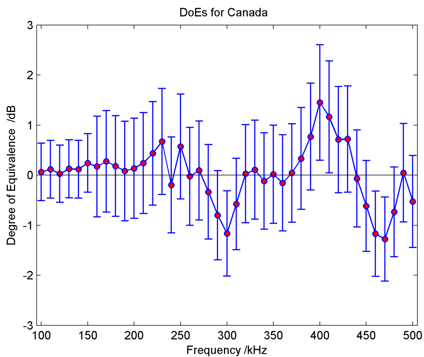
Figure G12. Combined Degrees of Equivalence for Canada in the frequency range 100 kHz to 500 kHz. Error bars indicate expanded uncertainties for a coverage factor of k=2 .
