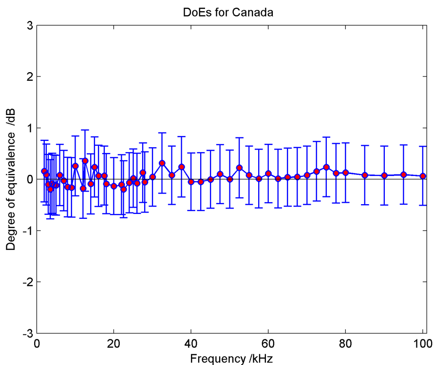
Figure G11. Combined Degrees of Equivalence for Canada in the frequency range 1 kHz to 100 kHz. Error bars indicate expanded uncertainties for a coverage factor of k=2 .
