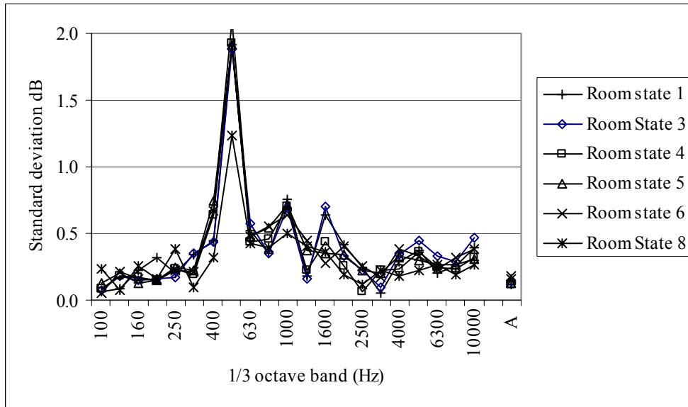
Figure 21. Standard Deviations determined from 4 repeat sound power determinations for the Box in rooms that qualified for broadband noise sources
