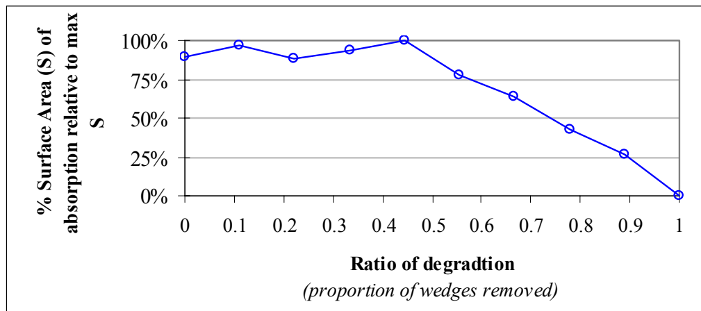
Figure 10. Exposed wedge surface area within the room
