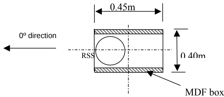
Figure 3. Plan view of section of 'box' source
