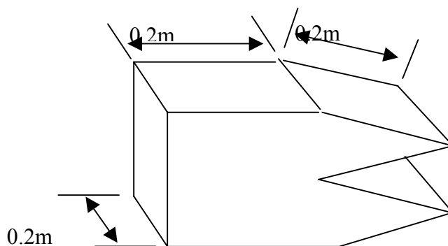
Figure A.1.1 Dimensions of acoustically absorbent wedges
