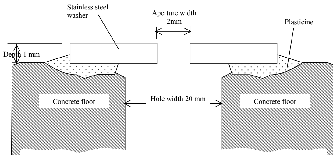
Figure 2. Cavity source aperture
