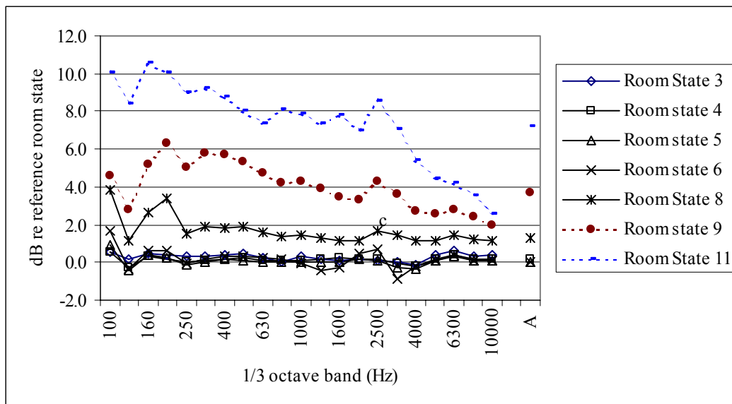
Figure 28. Level differences, \Delta L determined for the RSS in rooms that qualified for broadband noise sources
