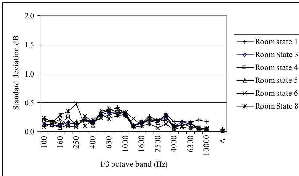
Figure 22. Standard Deviations determined from 4 repeat sound power determinations for the RSS in rooms that qualified for broadband noise sources
