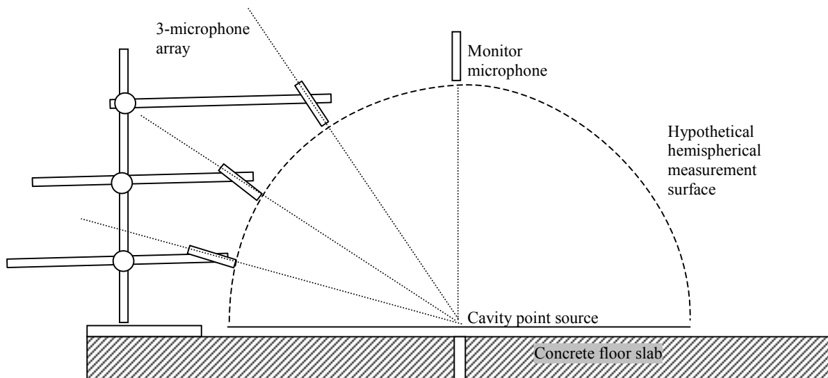
Figure 6. Microphone array set-up.
