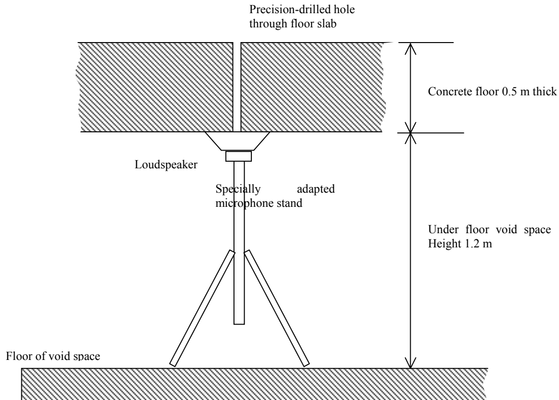
Figure 1. Cavity source configuration
