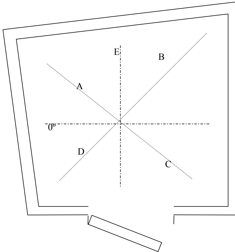
Figure 8. Plan view of hemi-anechoic room showing directions for the radial lines
