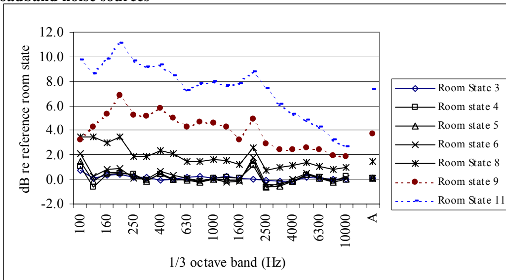
Figure 27. Level differences, \Delta L determined for the Box source in rooms that qualified for broadband noise sources
