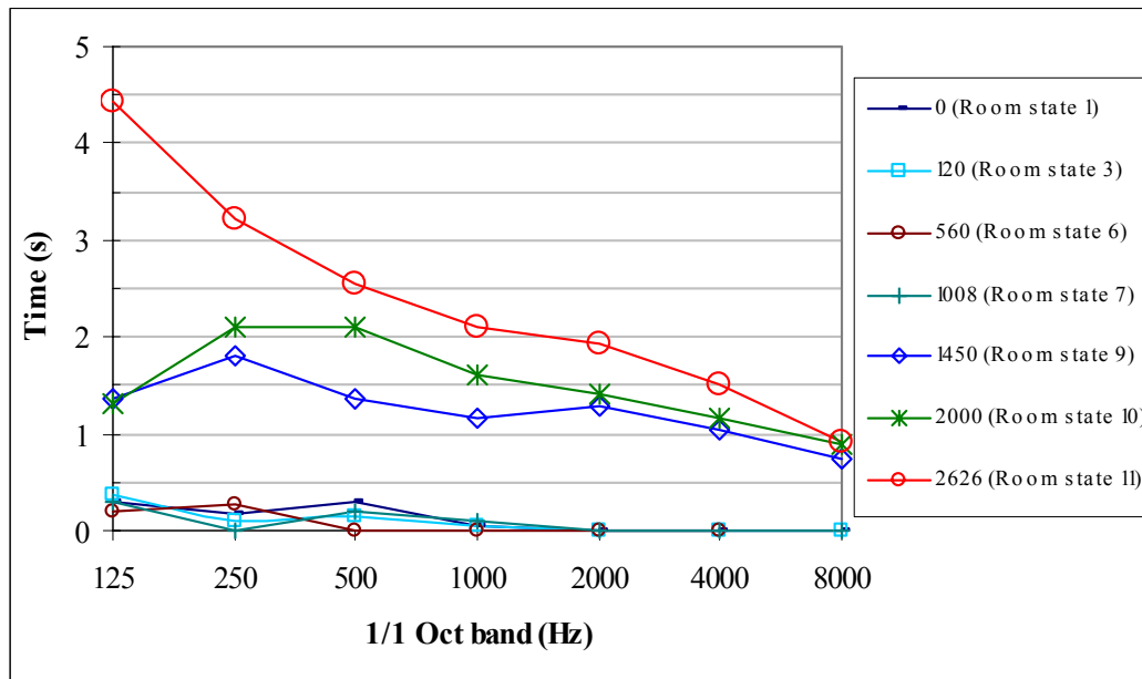
Figure 17. Reverberation time measurement results
