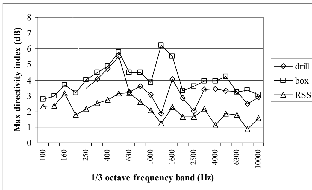
Figure 5. Directivity characteristics of selected noise sources
