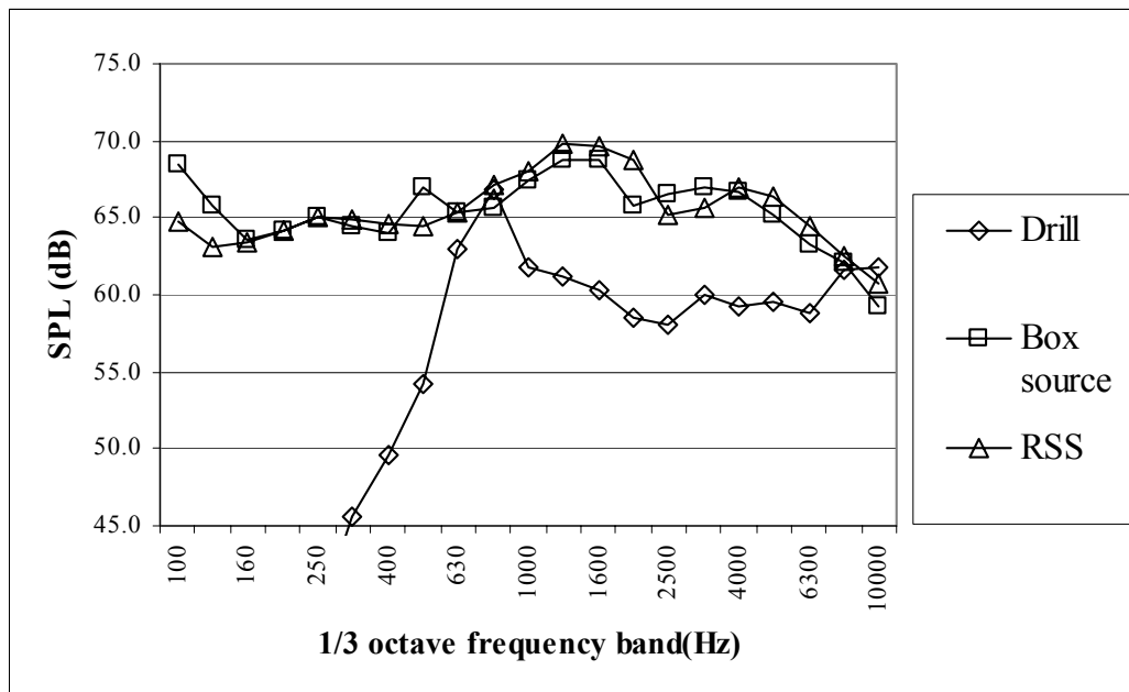
Figure 4. Frequency spectra of selected machines determined under hemi-anechoic conditions
