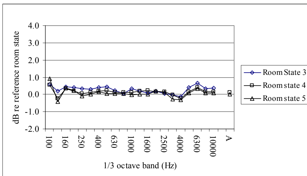
Figure 25. Level differences, \Delta L determined for the RSS in rooms that qualified for tonal noise sources
