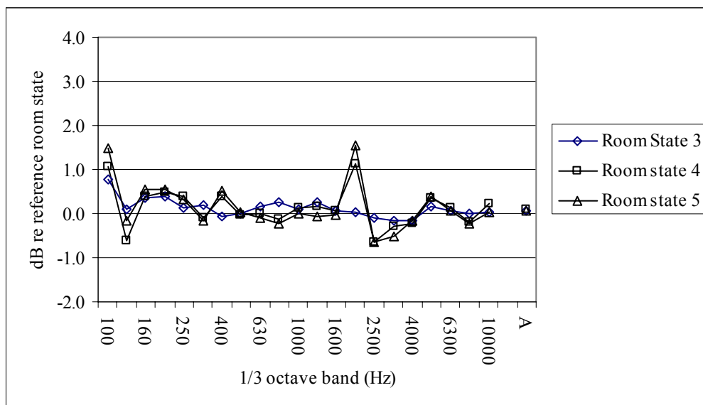
Figure 24. Level differences, \Delta L determined for the Box source in rooms that qualified for tonal noise sources
