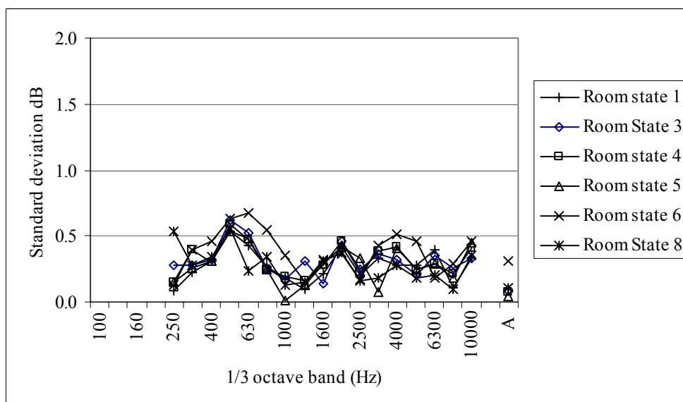
Figure 20. Standard Deviations determined from 4 repeat sound power determinations for the Drill in rooms that qualified for broadband noise sources
