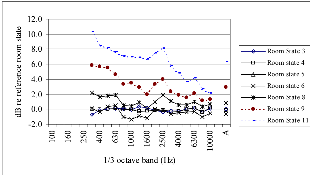
Figure 26. Level differences, \Delta L determined for the Drill in rooms that qualified for broadband noise sources
