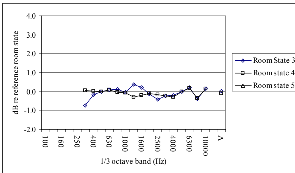
Figure 23. Level differences, \Delta_L determined for the Drill in rooms that qualified for tonal noise sources
