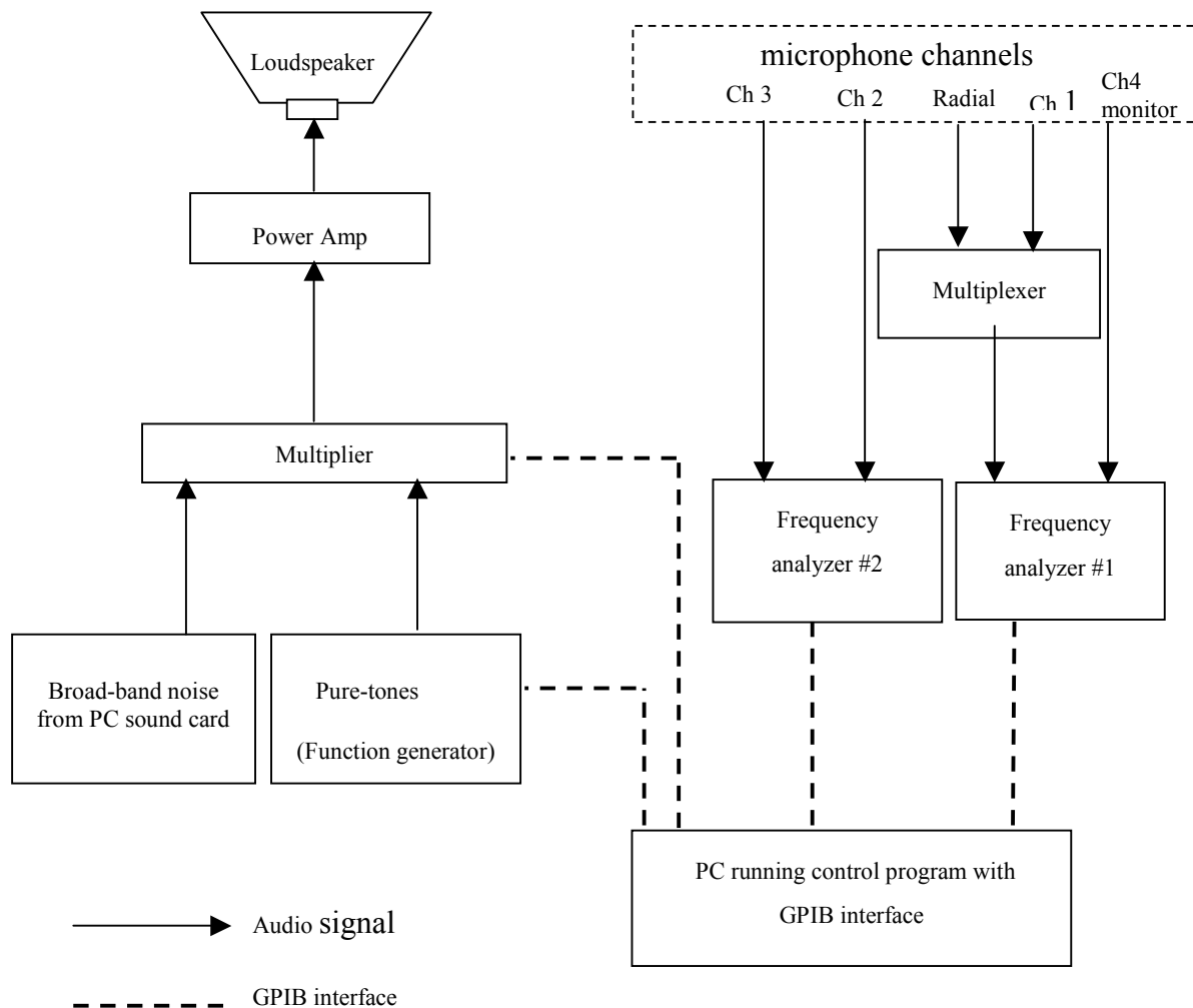
Figure 7. Schematic diagram of measurement system
