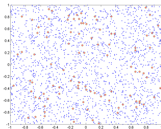
Figure 28: xy -coordinates of a subset of the interferometric data (Figure 17). The RBF centres are marked with an 'o'.
