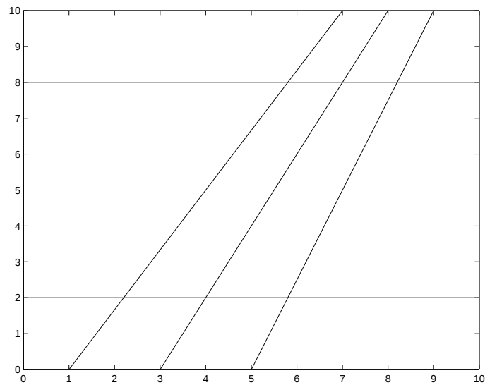
Figure 14: Knot-lines used in the representation of a tensor product spline surface approximation.
