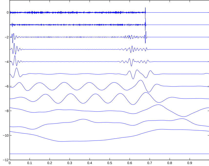
Figure 12: A Multi Resolution Analysis representation of the wavelet coefficients from the NDWT based on the Symmlet 6 wavelet. The horizontal axis corresponds to the position in the signal and the vertical axis to the scale or frequency. Note that here the vertical axis is inverted so the high frequencies are at the top of the figure.
