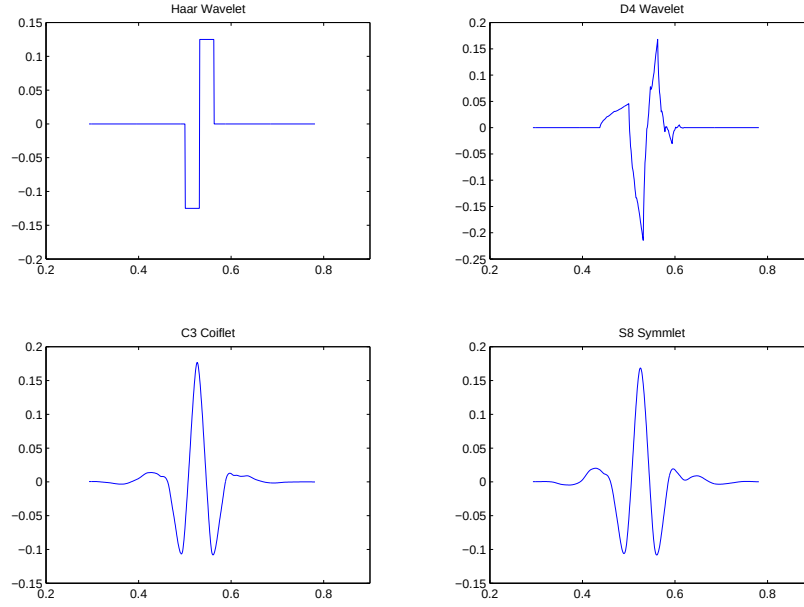
Figure 13: Examples of 4 types of wavelets: the Haar (DB1), the Daubechies 4 wavelet (DB4), Coiflet (C3), and Symmet (S8).
