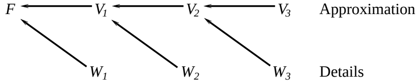
Figure 3: Schematic reconstruction of the function F from the 3-level decomposition. The approximation space V_3 and the detail spaces W_1, W_2, W_3 are all that are required.
