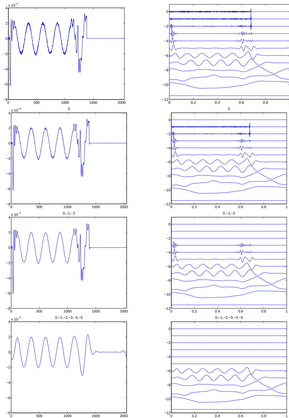
Figure 26: Taking out fine scales (high frequencies) to obtain an extended sine wave.
