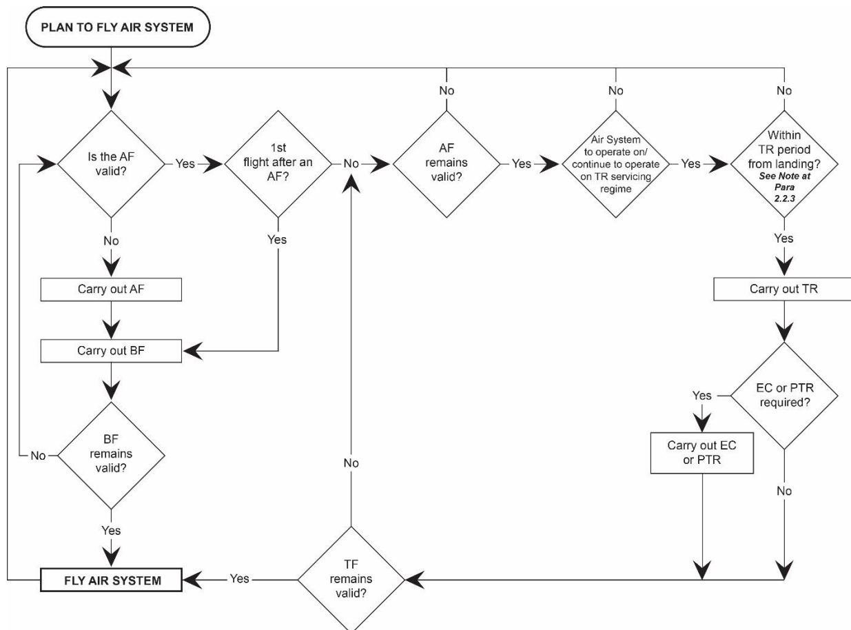
► Figure 1. Process for Maintaining Valid Flight Servicing ◀
