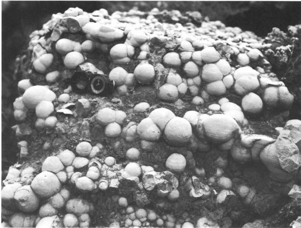
Figure 3.20: Mutually interfering subspherical calcite concretions ('cannon-balls') in a matrix of fine-grained dolomite. Note the parallel bedding traces preserved on the surface of some of the concretions. Loose specimen from floor of Southwick Quarry. Reproduced by permission of the Director, British Geological Survey: NERC copyright reserved (NL 130).
