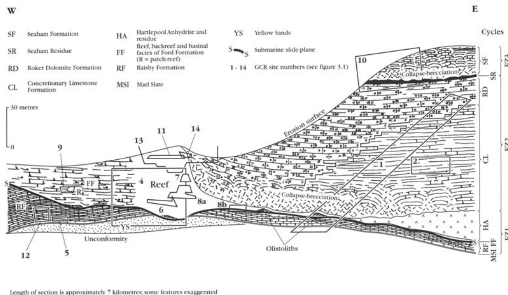
Figure 3.2: Approximate stratigraphical position of GCR marine Permian sites in the northern part of the Durham Province of north-east England (diagrammatic). Some sites in the southern part of the Durham Province cannot be accommodated on this line of section and have been omitted. The Hartlepool Anhydrite would not normally be present so close to the present coastline but is included for the sake of completeness. The biostrome is the Hesleden Dene Stromatolite Biostrome.
