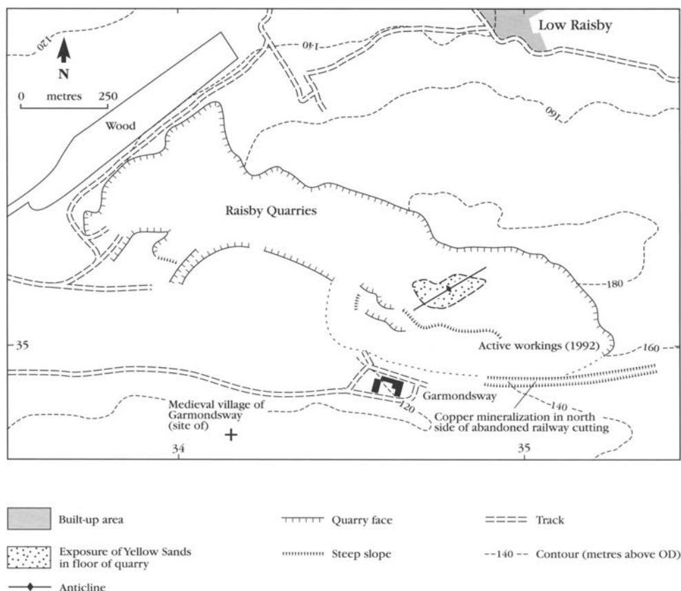
Figure 3.61: Raisby Quarries: the north face in the east is the type locality of the Raisby Formation (Smith et al., 1986).
