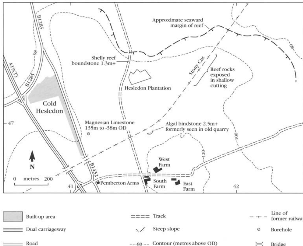
Figure 3.42: Location of Stony Cut, Cold Hesledon.
