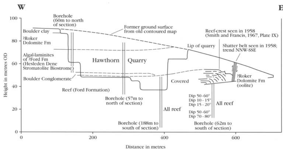
Figure 3.47: Section across Hawthorn Quarry, showing the relationships of the main geological features. The line of section is shown in Figure 3.46.
