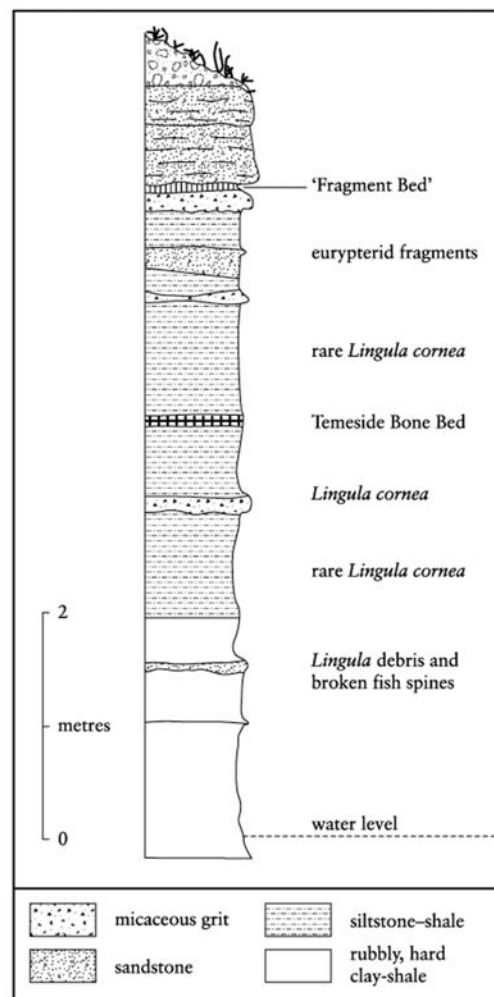
Figure 3.16: Stratigraphical section at Temeside. (After Elles and Slater, 1906).
