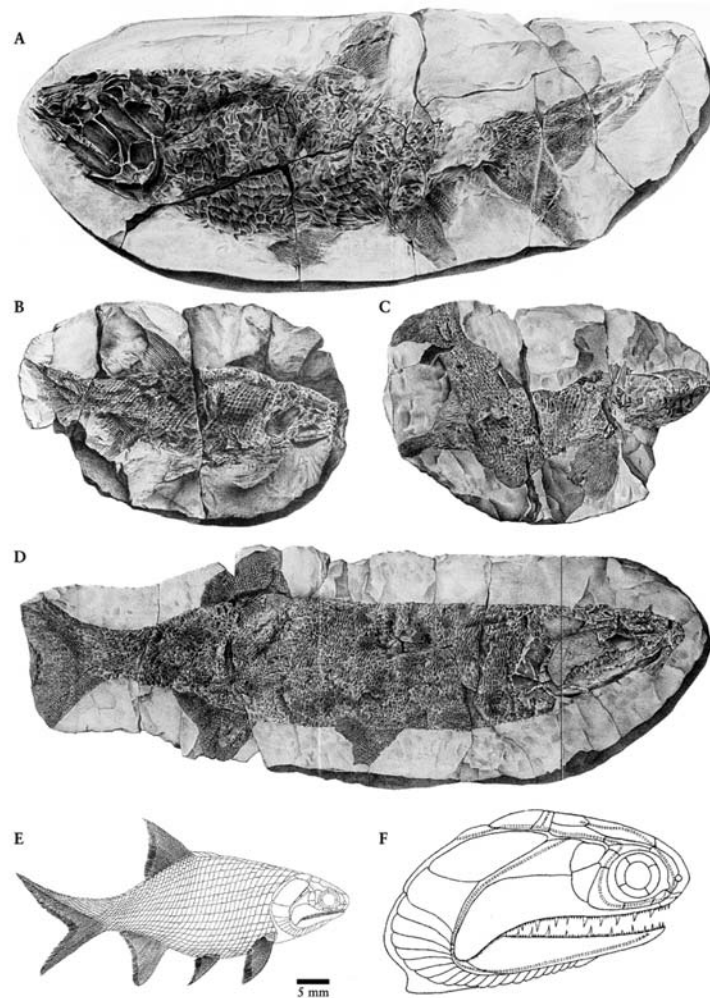
Figure 9.14: Actinopterygians in nodules from the Wardie Shale, Wardie, (A)–(D) are all c. \times 0.66 . (A) Cosmoptychius striatus Agassiz, specimen in nodule; (B) Elonichthys robisoni Hibbert; (C) Rhadinichthys ferrox Traquair; (D) Nematoptychius greenocki Traquair; (E) Gonatodus punctatus Agassiz, restoration from Gardiner (1967a); (F) Nematoptychius greenocki Traquair, restoration of the head by Gardiner (1963), c. \times 0.5 .
