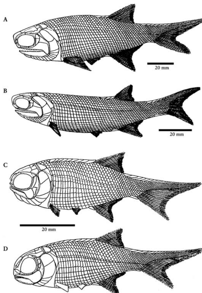
Figure 9.17: Some of the relatively more common Glencartholm actinopterygians: restorations in lateral view by Moy-Thomas and Bradley Dyne (1938). (A) Rhadinichthys fusiformis Traquair; (B) R. canobensis Tranquair; (C) Canobius ramsayi Traquair; (D) C. elegantulus Traquair.
