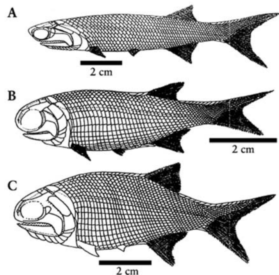
Figure 9.18: Glencartholm actinopterygians: restorations in lateral view by Moy-Thomas and Bradley Dyne (1938). (A) Cycloptychius concentricus Traquair; (B) Mesopoma politum Traquair; (C) Mesopoma crassum Traquair.
