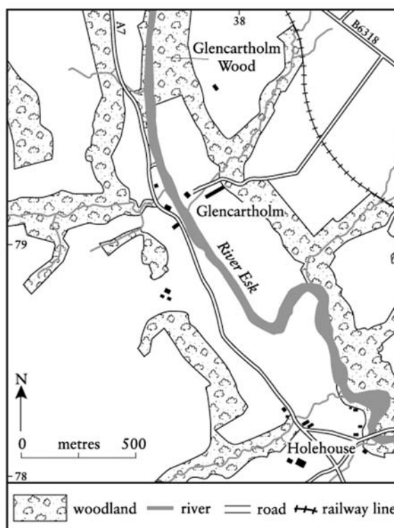
Figure 9.16: Sketch map of the Glencartholm GCR site, Berwickshire.
