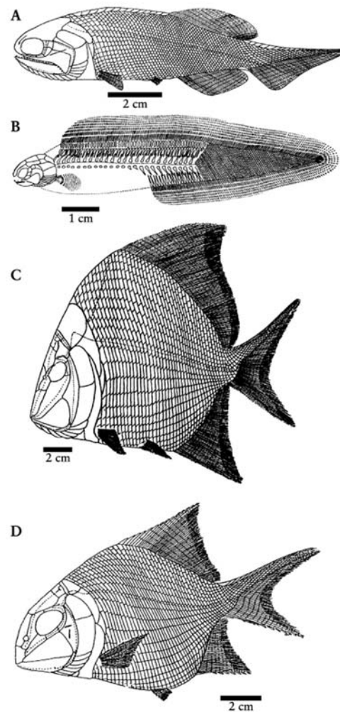
Figure 9.19: Glencartholm actinopterygians: restorations in lateral view by Moy-Thomas and Bradley Dyne (1938). (A) Holurus parki Traquair; (B) the elongated Tarrasius problematicus Traquair, once thought to be a crossopterygian (after Moy-Thomas, 1937b); (C) Platysomus superbus Traquair; (D) Cheirodopsis geikiei Traquair. (C) and (D) are typical deep-bodied actinopterygians.
