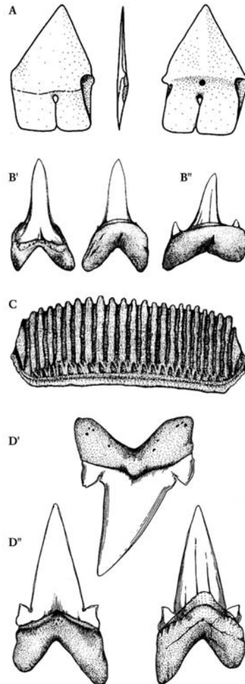
Figure 14.7: Fossil fishes from the London Clay at Bognor Regis. (A) labial, mesial and lingual views of Isistius triangularis (Probst), lower lateral tooth (after Capetta, 1987), \times 9 ; (B) Isurolamna affinis (Casier): (B') anterior tooth, labial and lingual views \times 2 ; (B'') antero-lateral tooth, labial view \times 2 ; (C) Myliobatis dixonii Agassiz median tooth, basal view, \times 2 ; (D) Otodus obliquus Agassiz: (D') upper lateral tooth labial view \times 1 ; (D'') lower anterior tooth, lingual and labial views, \times 1 . (B)–(D) from Kemp et al., 1990).
