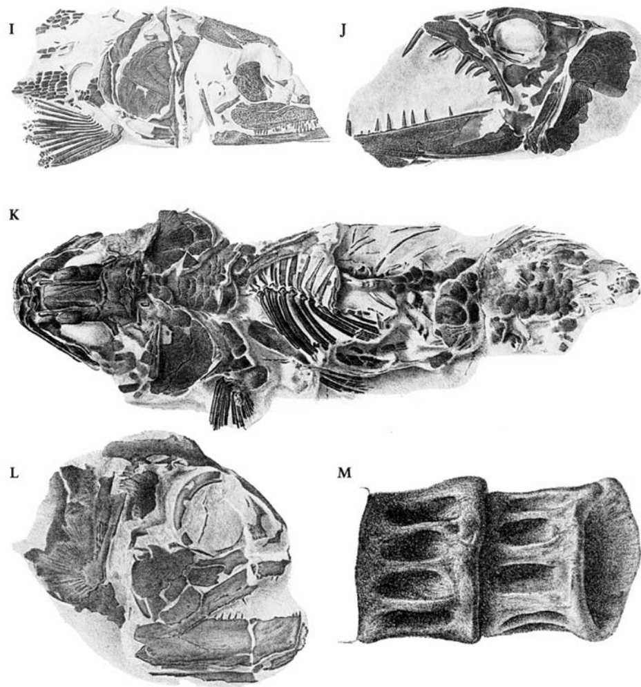
Figure 13.13: Fossil fishes from Burham Blue Bell Hill Pits (all from Woodward, 1895a): (A) Cantioscyllium decipiens Woodward, anterior part of the skeleton; hy, hyoid arch; md, mandible; pct, pectoral arch; pq, palato-quadrates, \times 0.75 ; (B), (C) Scylliorhinus antiquus (= Scyllium antiquum ) Agassiz, teeth in labial and lingual views, \times 4.0 and \times 0.5 respectively; (D) Scylliorhinus antiquus (= Scyllium antiquum ) Agassiz, dermal denticles, c. \times 10 ; (E) Ischyodus incisus Newton, left mandibular dental plate; outer, inner and upper views, \times 1.5 ; (F), (G) Pachyrhizodus basalis Dixon; (F) part of the right premaxilla with teeth, \times 1 ; (G) right dentary in lower and inner aspects, \times 0.25 ; (H) Pachyrhizodus dibleyi Woodward, left maxilla in outer view, \times 0.3 . (I) Neorhombolepis excelsus Woodward (from Kent), imperfect head and anterior abdominal region ( N. punctatus ) Woodward, (known from scales in Burnham area), \times 0.6 ; (J) Enchodus pulchellus Woodward, holotype (NHM P.1703) left-hand side of the head and opercular area, \times 0.9 ; (K) Sardinioides illustrans Woodward, holotype (NHM P.3977) imperfect crushed specimen in ventral view, \times 0.6 ; (L) Ichthyodectes tenuidens Woodward, right side of head and jaw, \times 1 ; (M) Ichthyodectes sp., two vertebral centra, \times 1 .
