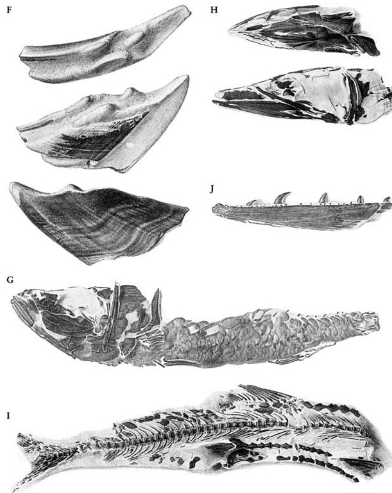
Figure 13.19: Fossil fishes from the Chalk of the Lewes area (after Woodward, 1895b). All distorted head and jaw parts; (A), (A') Apateodus striatus Woodward, distorted head, right and left lateral views, both are c. \times 1.0 ; (B) Hoplopteryx lewesiensis Woodward, restoration \times 0.5 ; (C) Thrissopater megalops Woodward, head with left pectoral arch, \times 0.6 ; (D) Tomognathus mordax Dixon, imperfect skull and left mandible, \times 1 ; (E) Elasmodectes willetti Newton, right side of head and part of trunk, \times 0.8 . (F) Edaphodon agassizi (Buckland), left mandibular dental plate in labial, lingual and upper views, \times 1 ; (G) Aulolepis typus Agassiz, incomplete head and trunk in left lateral view, \times 3 ; (H)–(J) Cimolichthys lewesiensis Leidy: (H) head and opercular region in dorsal and left lateral views \times 0.35 , (I) damaged trunk and tail parts \times 0.35 , (J) labial aspect of left dentary \times 0.9 . (K) Macropoma mantelli Agassiz, crushed skull in right lateral view, \times 0.6 ; (L) Enchodus lewisiensis Mantell, head and anterior part of trunk in lateral view, \times 0.9 ; (M), (N) Halec eupterginus (Dixon): (M) head and abdominal region in lateral view, \times 0.9 , (N) head in lateral view, \times 1 .
