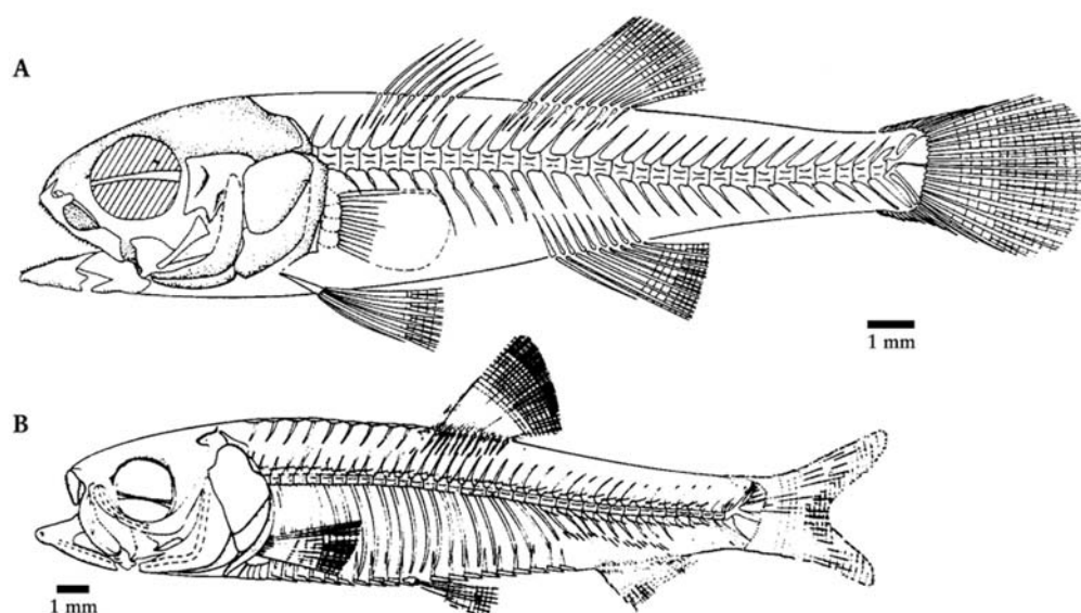
Figure 14.16: Fossils from the Osborne Beds at King's Quay, Isle of Wight (after Gaudant and Quayle, 1988, © The Natural History Museum, London): (A) reconstruction of Potamoschistus (?) cf. bleicheri (Sauvage); (B) reconstruction of Vectichthys vectensis (Newton).
