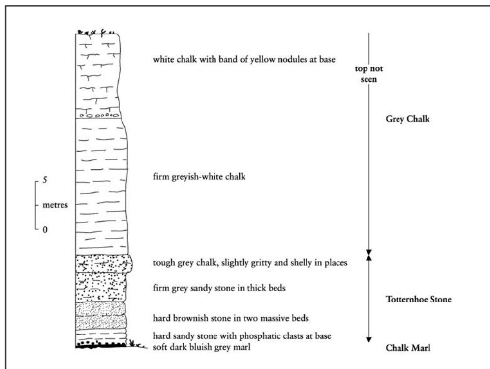
Figure 13.14: Totternhoe Chalk stratigraphical log (after P.J. Smart).
