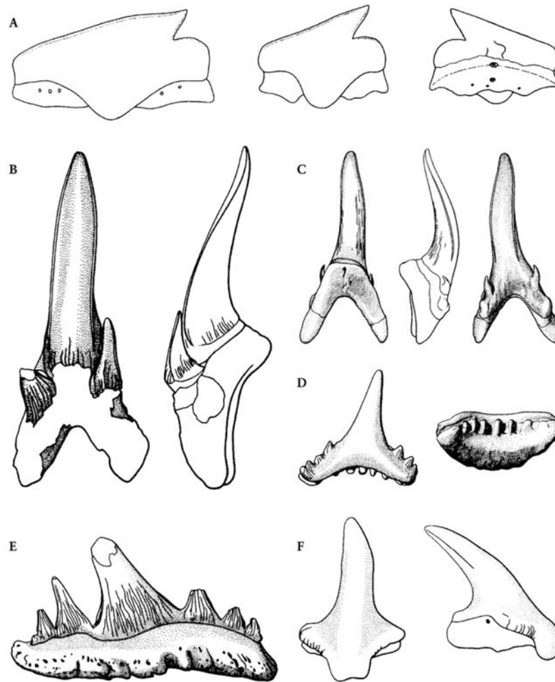
Figure 13.15: Fossil chondrichthyan teeth genera from the Chalk at Totternhoe (after Cappetta, 1987). (A) Protosqualus sp., \times 24 ; (B) Leptostyrax sp., \times 1.25 in distal view; (C) Synodontaspis ( Carcharias ) striatula , \times 2 in distal view; (D) Synechodus sp. \times 5 ; (E) Paraorthacodus sp., \times 4 ; (F) Squatirhina sp., \times 10 , in labial and distal views.
