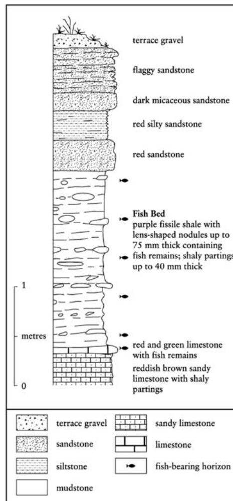
Figure 6.23: Stratigraphical section through Dipple Brae Fish Bed (based on data from M.A. Rowlands MS).
