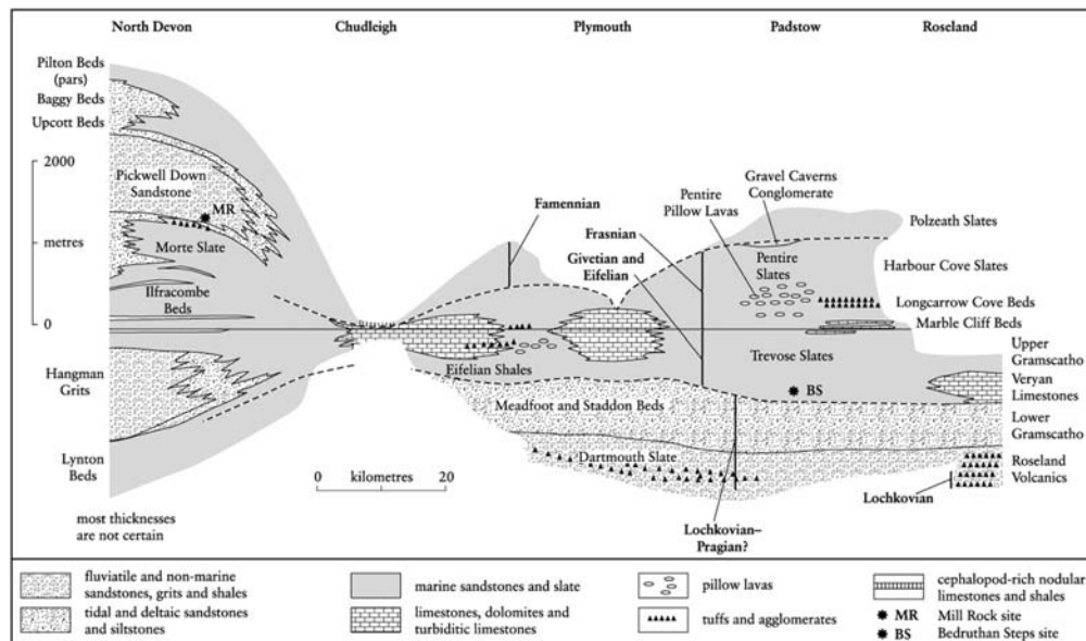
Figure 7.3: Simplified non-palinspastic facies section of Devon and Cornwall (after House, 1975).
