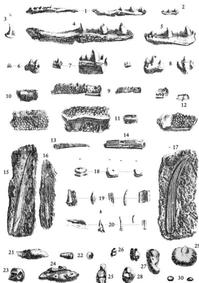
Figure 3.10: Fossils from the Ludlow Bone Bed illustrated in a plate from Murchison's Siluria (1872). 1–8, Plectrodus mirabilis , fragments of jaws; 9–12, P. pustuliferus , fragments of jaws; 13, 14, Onchus murchisoni , fin spines; 15–17, O. trenuistriatus , fin spines; 18, Thelodus parvidens , denticles; 19–20, indeterminate fragments; 21–28, coprolites containing invertebrate fragments; 29, Orthis lunata Sowerby; 30, Pachtheca sphaerica . All approximately natural size.
