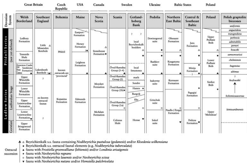
Figure 3.12: Ludlow–Přídolí correlation for Europe and North America. Vertical columns not drawn to scale (after Siveter et al. , 1989).
