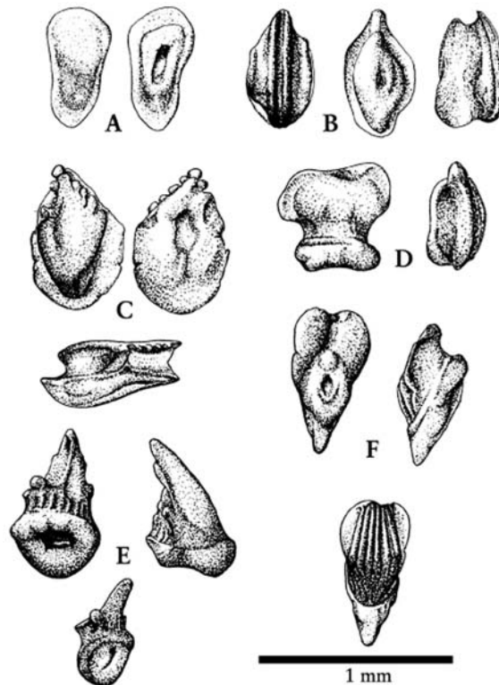
Figure 3.11: Thelodonts from the Ludlow Bone Bed (after Turner 1973) . (A) Thelodolus parvidens ; (B) Thelodolus bicostatus ; (C) Loganellia ludlowiensis head scale; (D) Thelodolus pugniformis ; (E) Thelodolus parvidens ?; (F) Thelodolus trilobatus .
